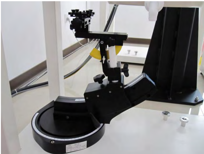
Figure 5-4. Device Holder
