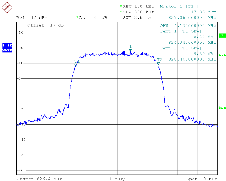
(Plot E2: WCDMA 850MHz Channel = 4132 99% Occupied Bandwidth)
