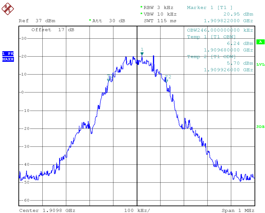
(Plot B6: GSM 1900MHz Channel = 810 99% Occupied Bandwidth)
