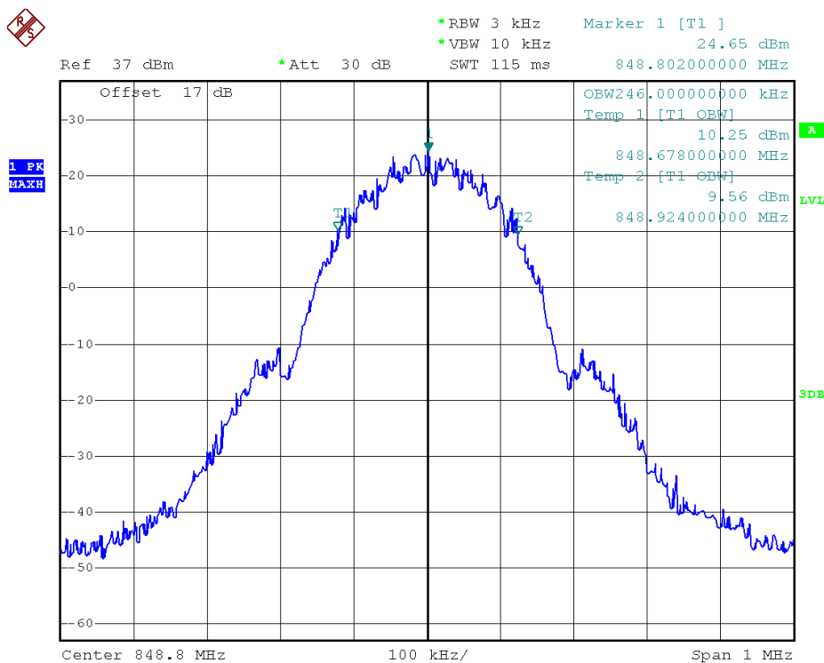
(Plot C6: EDGE 850MHz Channel = 251 99% Occupied Bandwidth)
