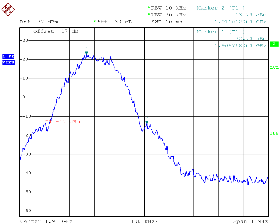
(Plot H: EDGE 1900 Channel = 810)
