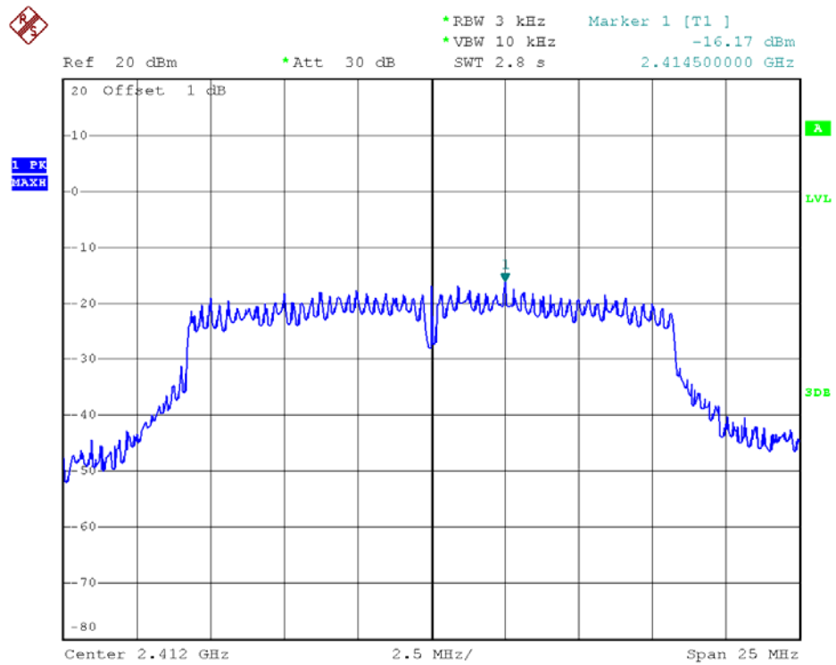
802.11g - Channel 1
