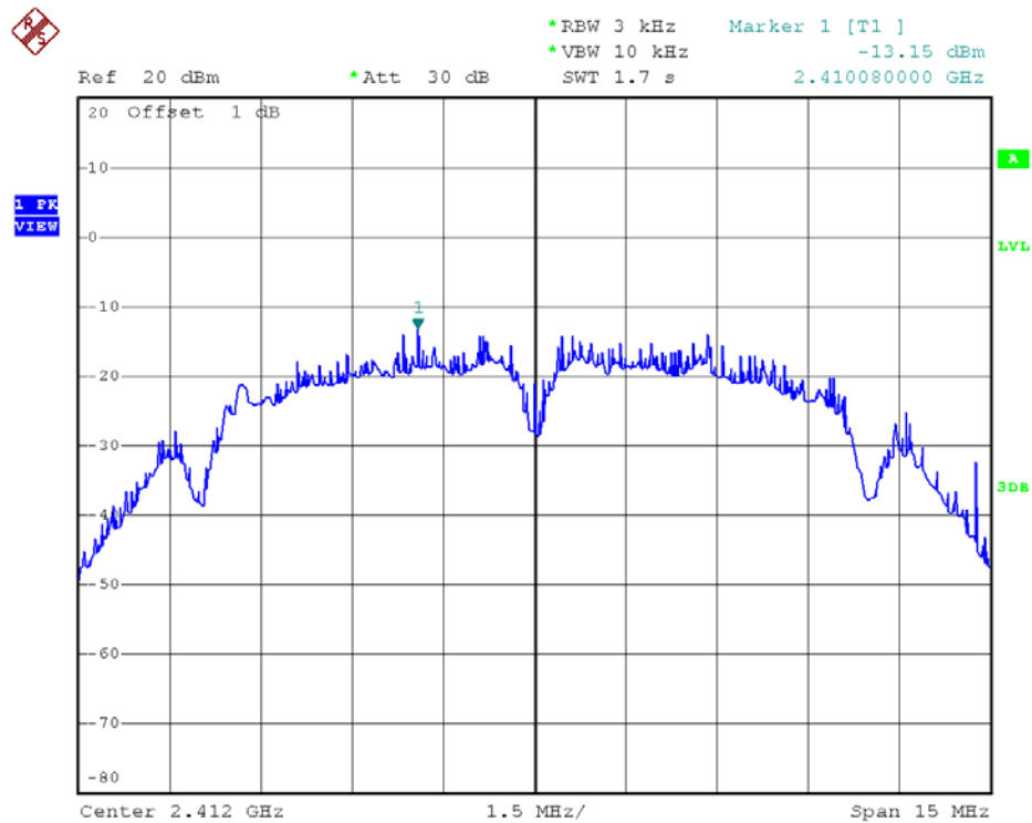
802.11b - Channel 1
