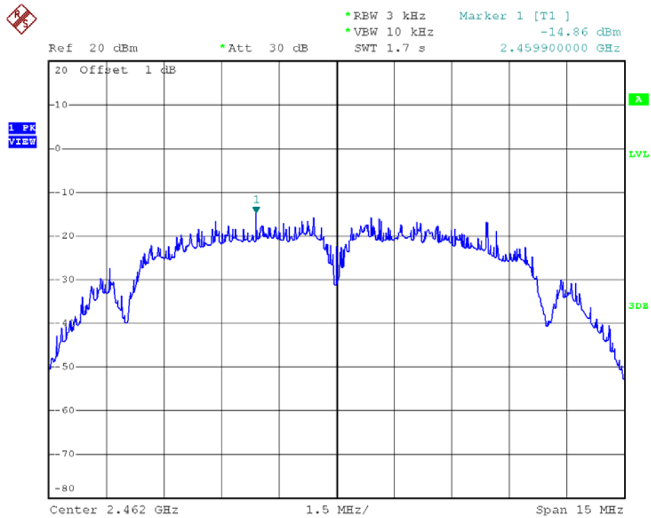
802.11b - Channel 11
