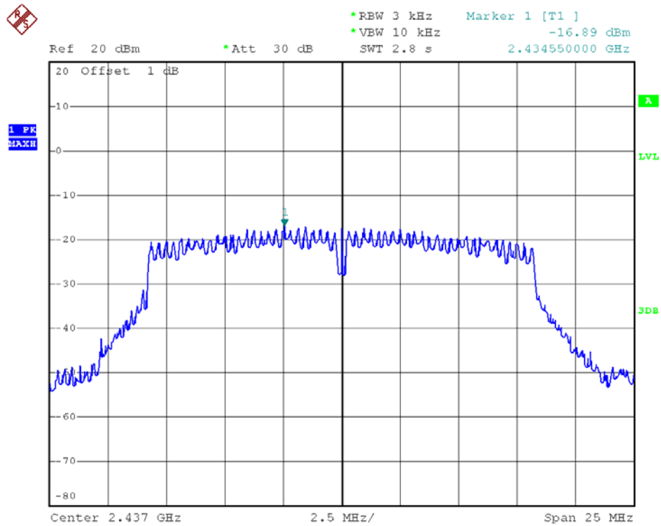
802.11g - Channel 6
