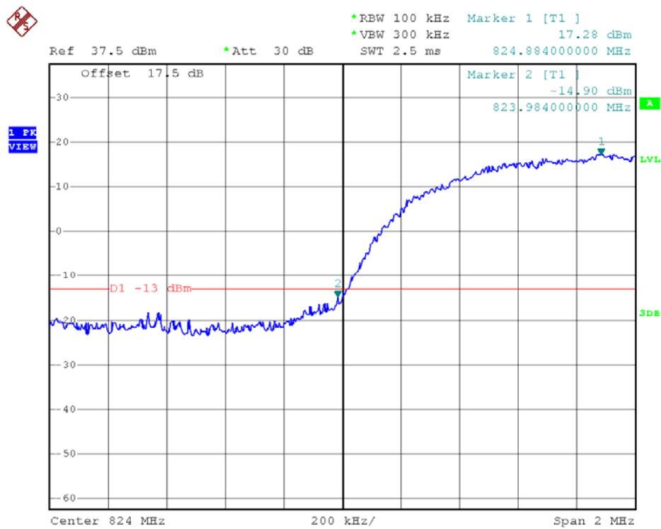
(Plot E: WCDMA 850 Channel = 4132)
