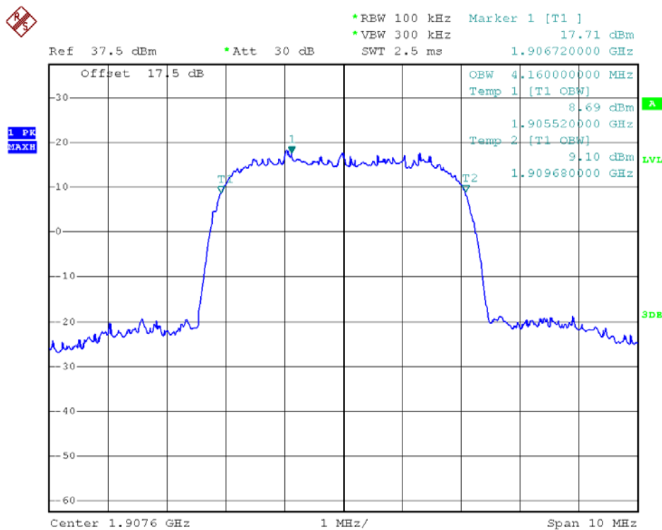
(Plot D6: WCDMA 1900MHz Channel = 9538 99% Occupied Bandwidth)
