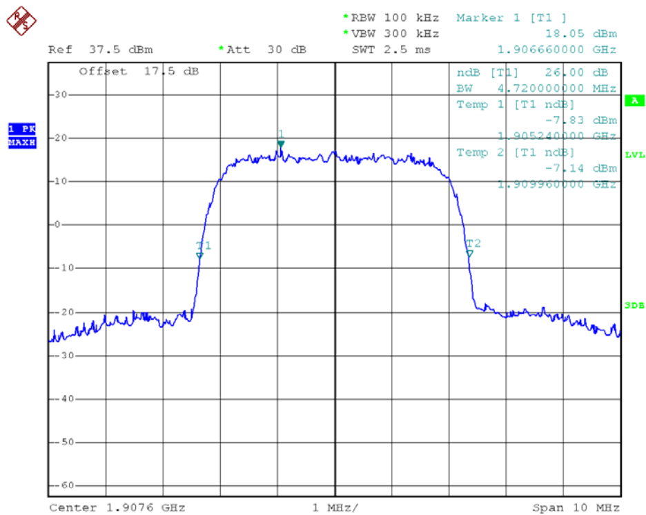
(Plot D5: WCDMA 1900MHz Channel = 9538 26dB bandwidth)
