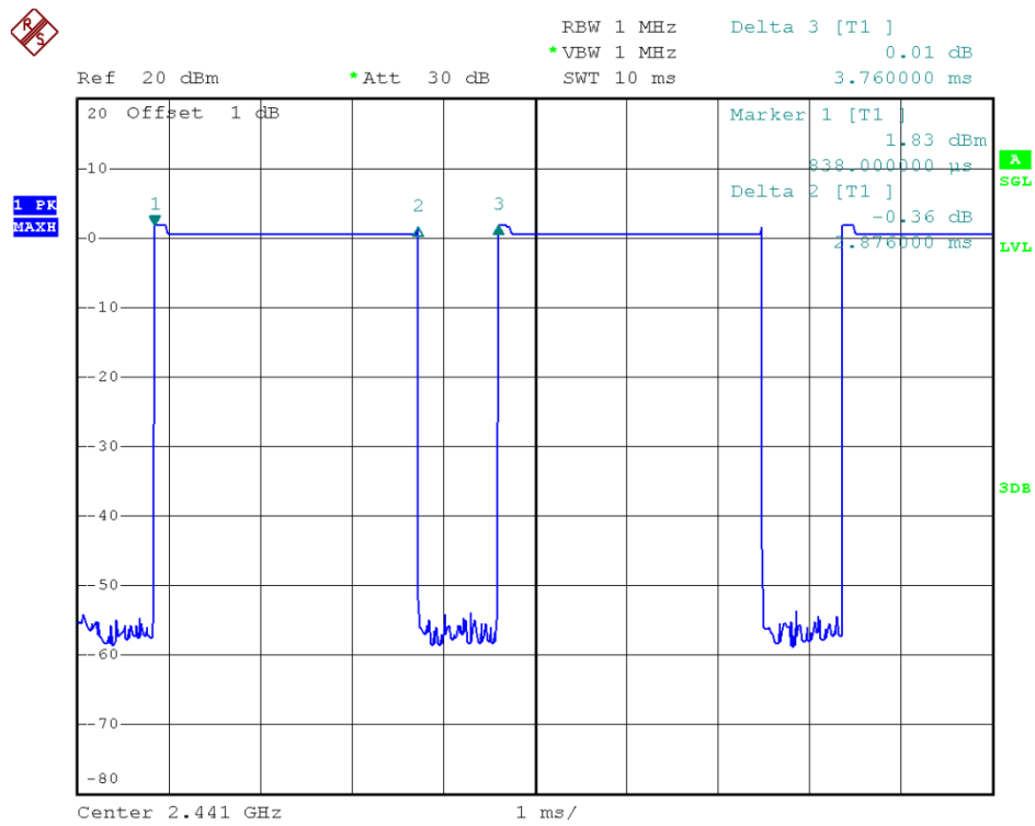
39 Channel @ 2DH5
