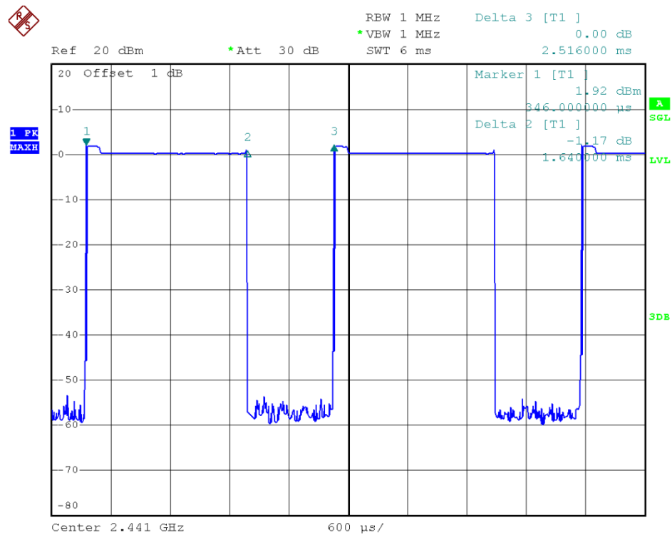
39 Channel @ 3DH3
