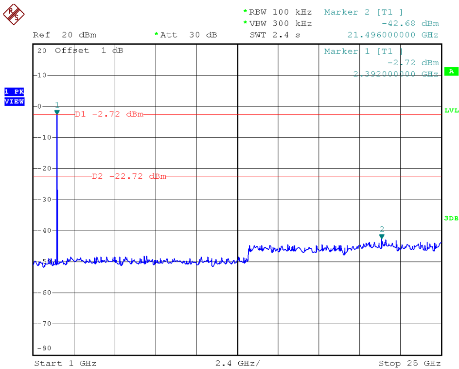
Low Channel 1GHz to 25GHz @ 8-DPSK
