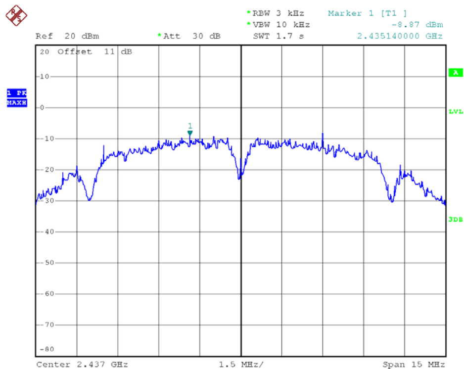
802.11b - Channel 6
