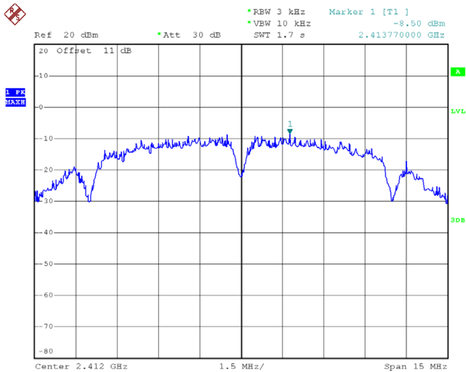
802.11b - Channel 1
