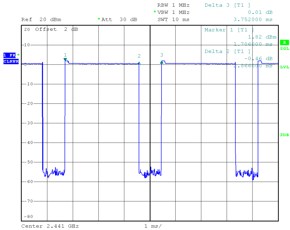
39 Channel @ 3DH5
