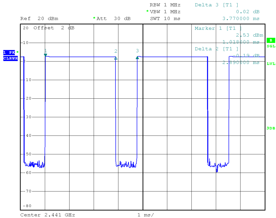
39 Channel @ DH5
