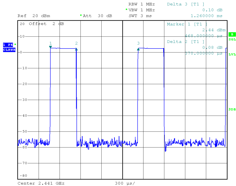
39 Channel @ DH1
