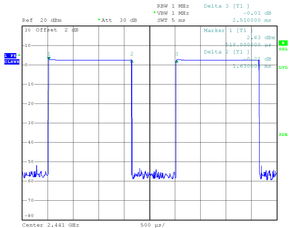
39 Channel @ DH3
