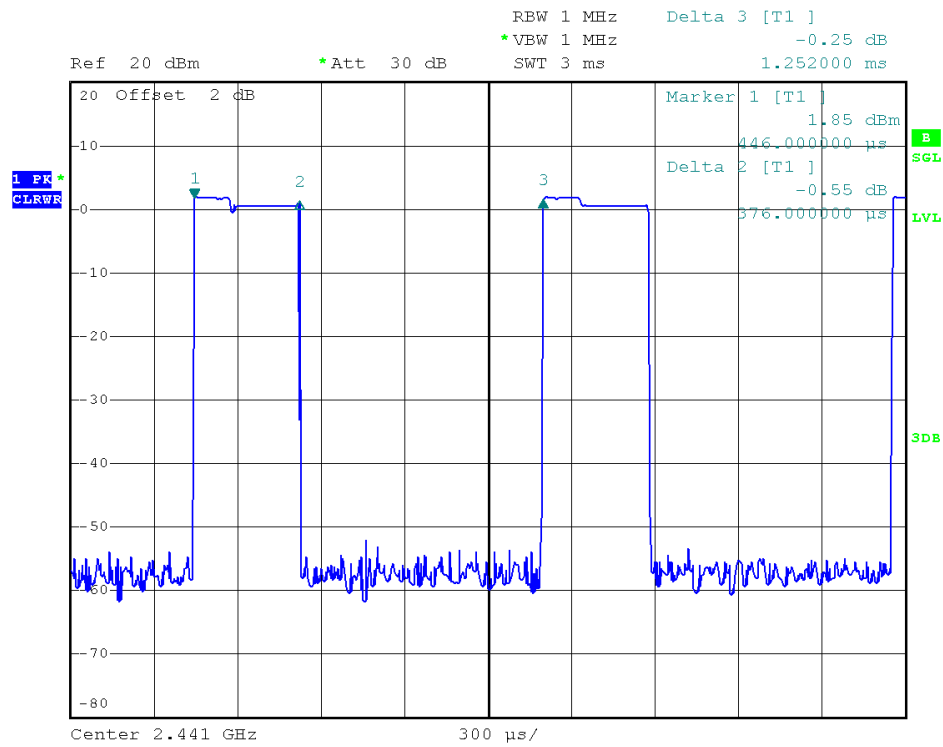
39 Channel @ 3DH1
