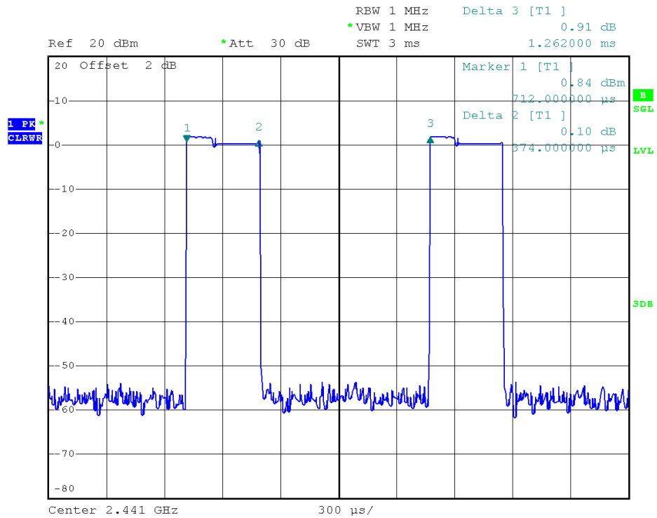
39 Channel @ 2DH1
