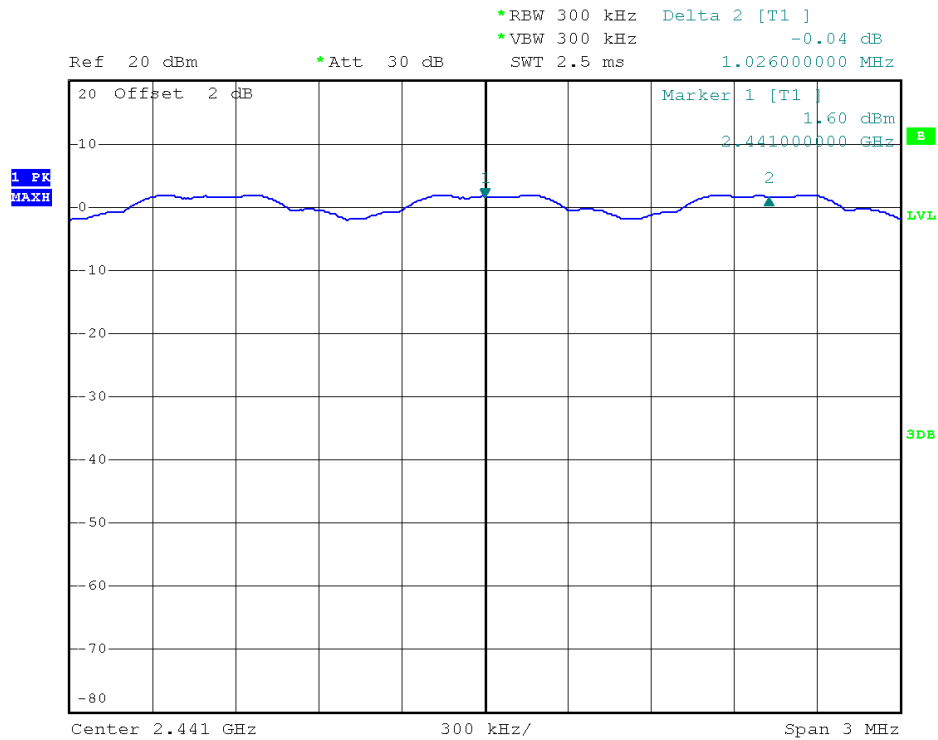
8-DPSK Mode
