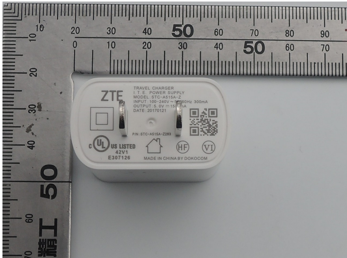
CHARGER View (STC-A515A-Z)
