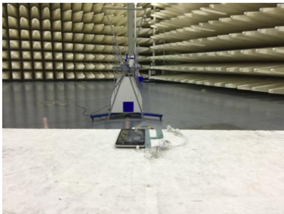
Pic4.Spurious Radiated Emissions Test setup (30MHz~1GHz)
