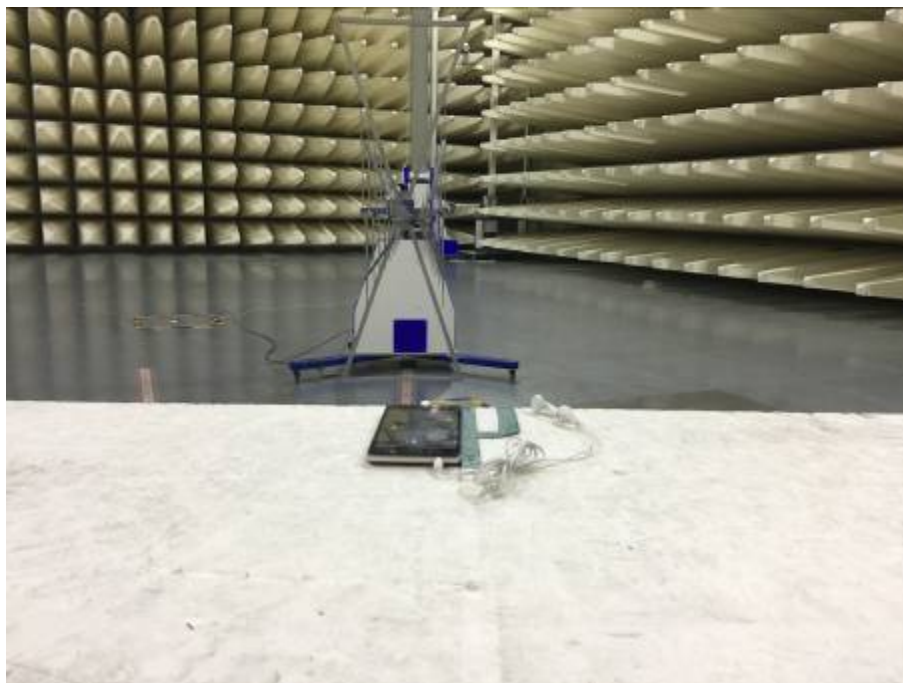
Pic7.Radiated Emissions Test Setup (with charger)
