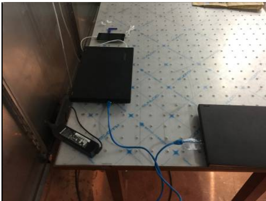
Pic8. Conducted Emissions Test Setup (with laptop)
