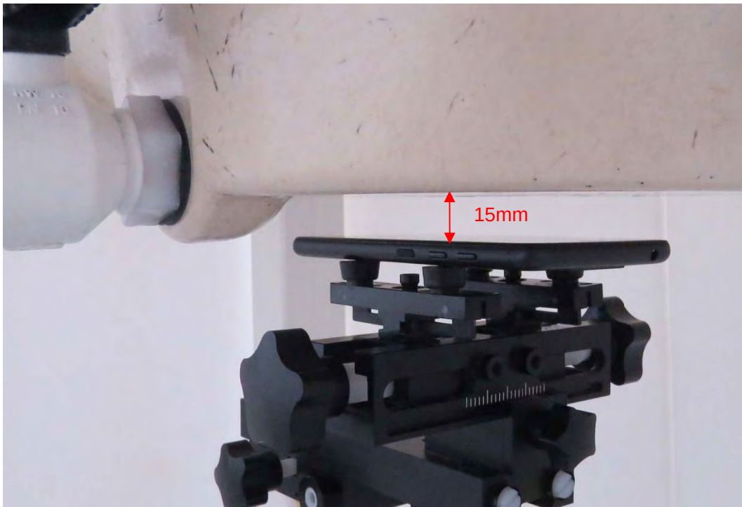
Picture 23: Front Side, the distance from handset to the bottom of the Phantom is 15mm
