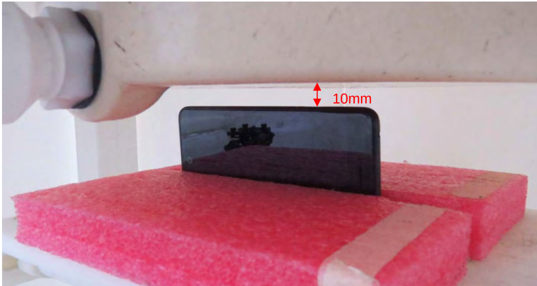
Picture 24: Left Side, the distance from handset to the bottom of the Phantom is 10mm
