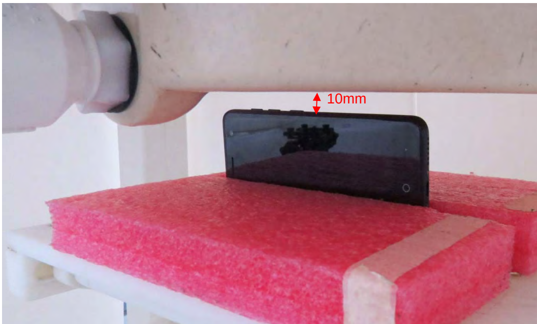
Picture 25: Right Side, the distance from handset to the bottom of the Phantom is 10mm
