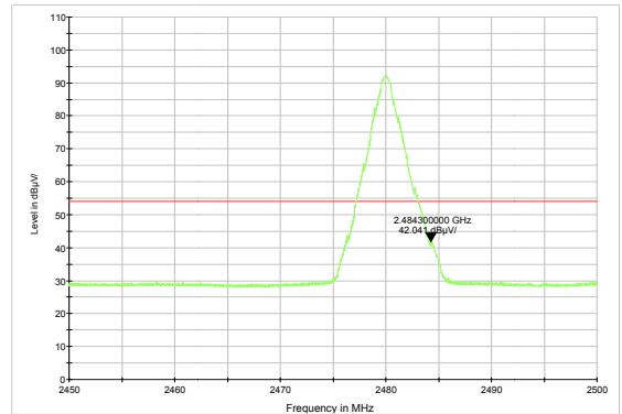
3DH5-Channel 78: Average
