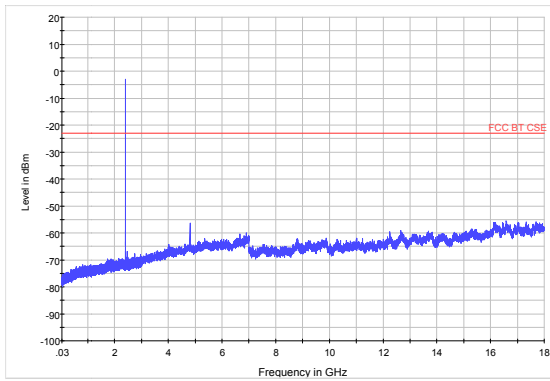
GFSK-CH39 30MHz to 18GHz
