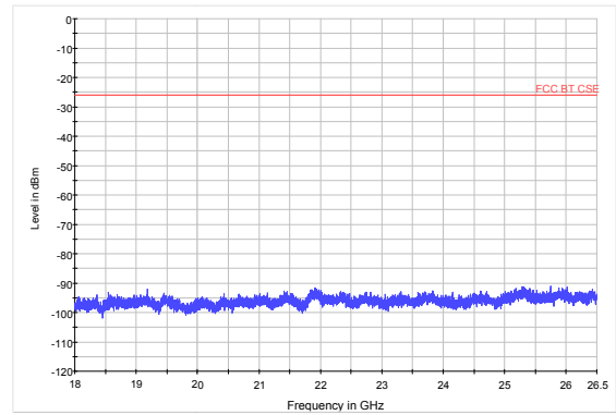
EDR-CH39 18GHz to 26.5GHz
