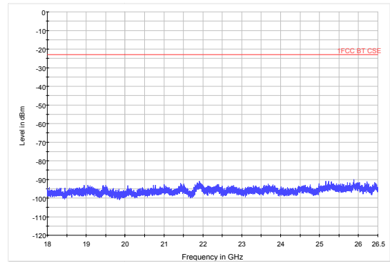
GFSK-CH39 18GHz to 26.5GHz
