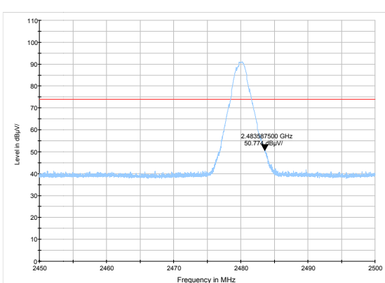
3DH5-Channel 78: Peak
