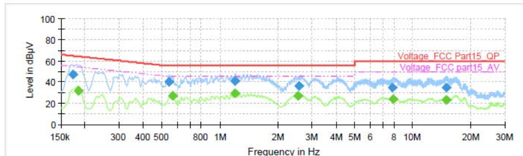
WIFI_L_0.15-30MHz
