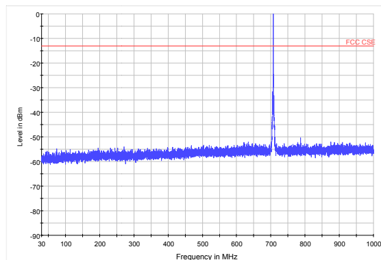
LTE Band 12 1.4MHz CH-Middle 30MHz~1GHz
