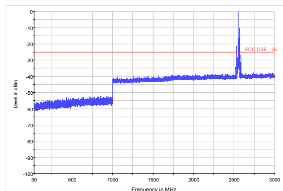
LTE Band 7 20MHz CH-High 30MHz~3GHz
