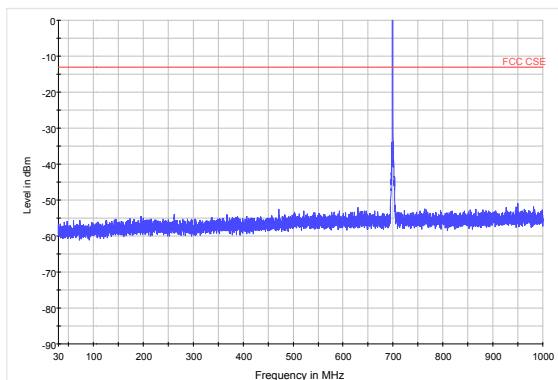
LTE Band 12 1.4MHz CH-Low 30MHz~1GHz
