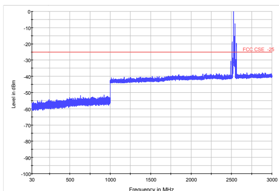
LTE Band 7 20MHz CH-Middle 30MHz~3GHz
