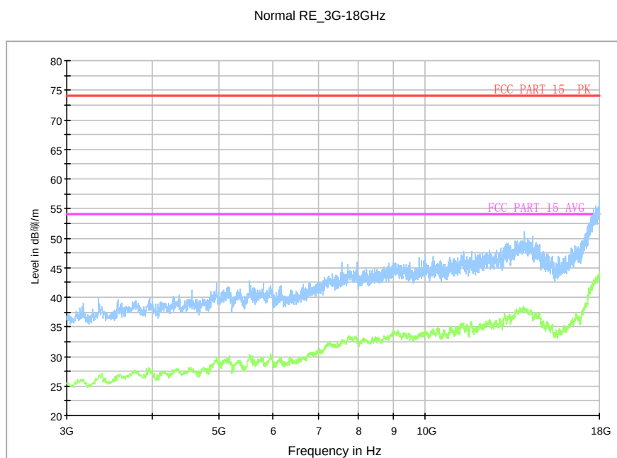
Fig.25. Radiated emission: GFSK, 2480MHz, 3 GHz - 18 GHz
