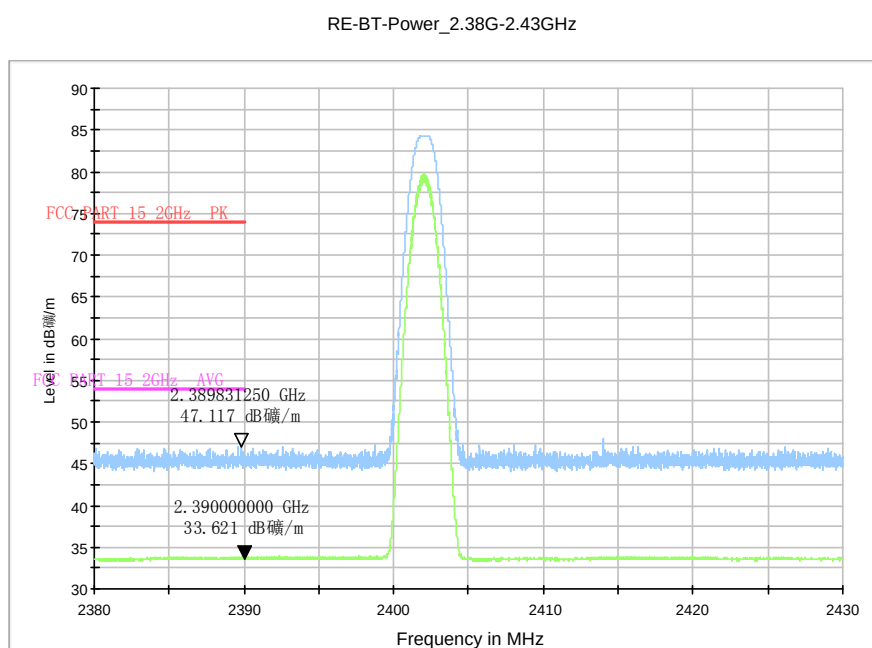
Fig.26. Radiated emission (Power): GFSK low channel
