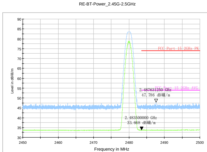
Fig.27. Radiated emission (Power): GFSK high channel
