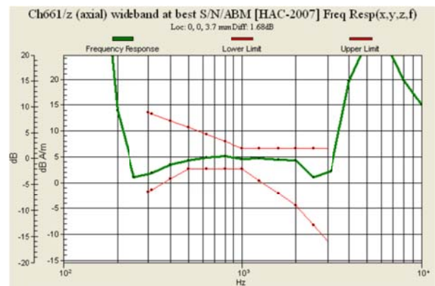
Fig 9.2 GSM1900 Ch661
