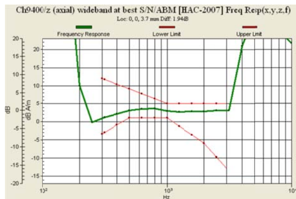
Fig 9.5 WCDMA Band II Ch9400
