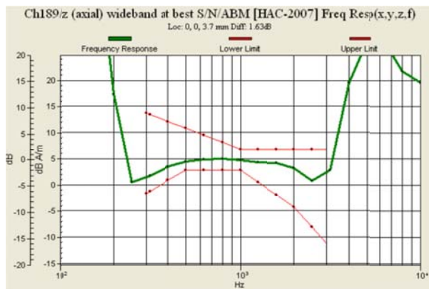
Fig 9.1 GSM850 Ch189
