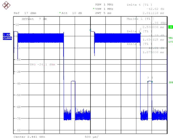
Fig.71 Number of Transmissions Measurement: Ch39, Packet 3-DH1
