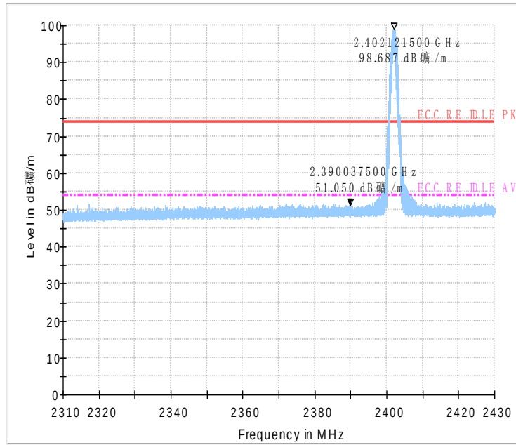
Fig.49 Radiated emission (Power): GFSK, low channel
