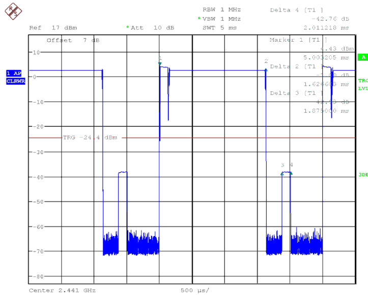
Fig.65 Number of Transmissions Measurement: Ch39, Packet 2-DH1
