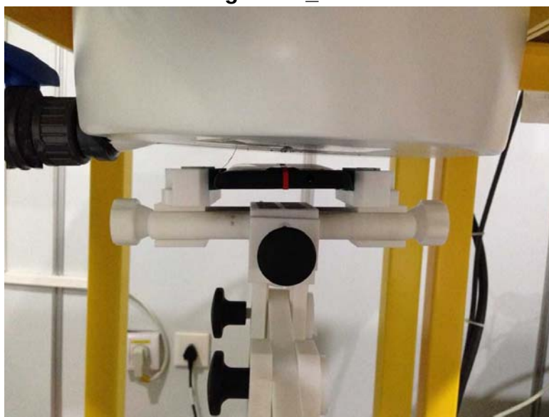
Fig.6 Body (Back upside,10mm separation)
