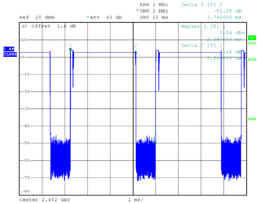
0 Channel @ 3DH5
