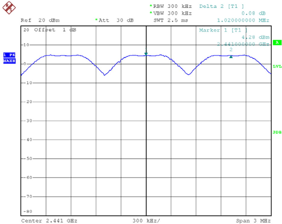
GFSK Mode, Middle Channel
