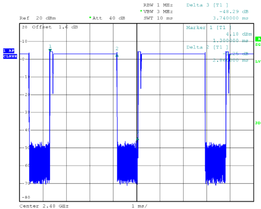
78 Channel @ 2DH5
