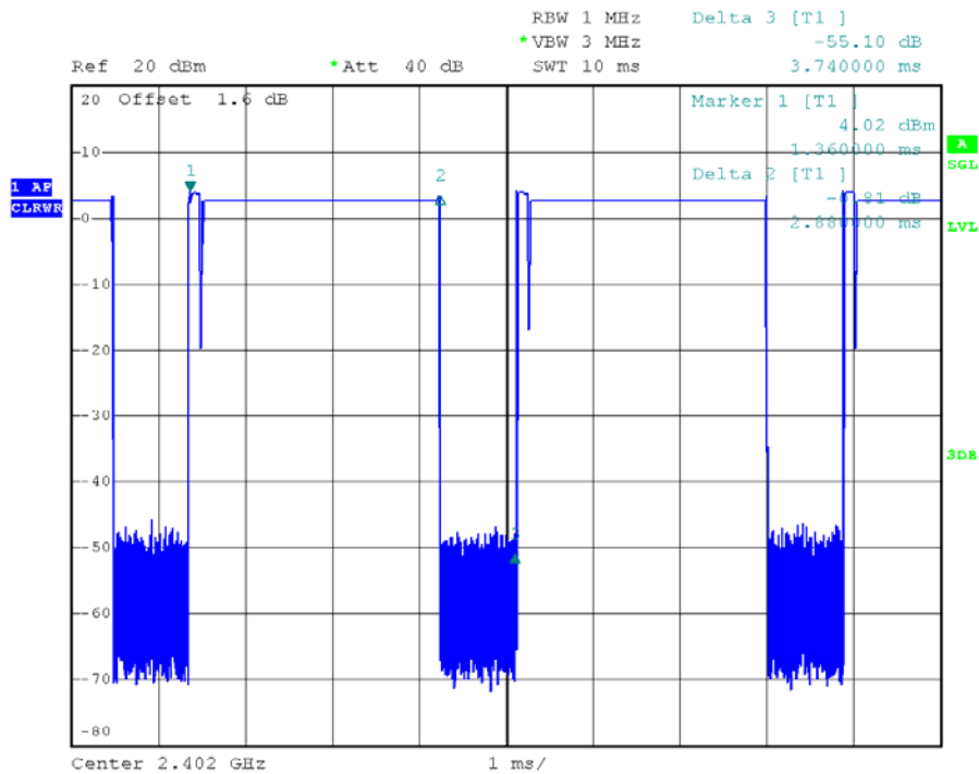
0 Channel @ 2DH5
