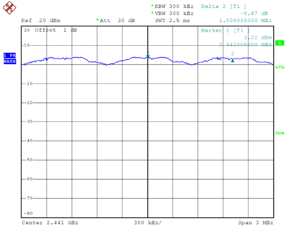
8-DPSK Mode, Middle Channel
