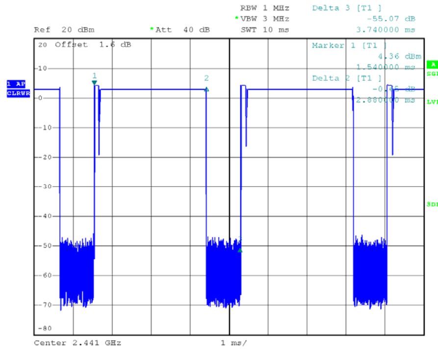
39 Channel @ 2DH5
