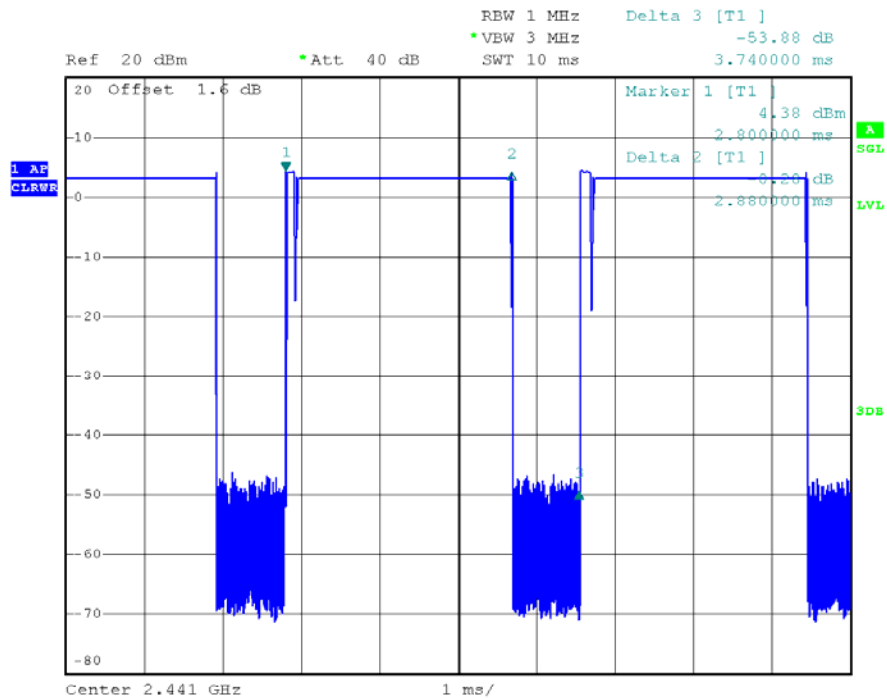
39 Channel @ 3DH5
