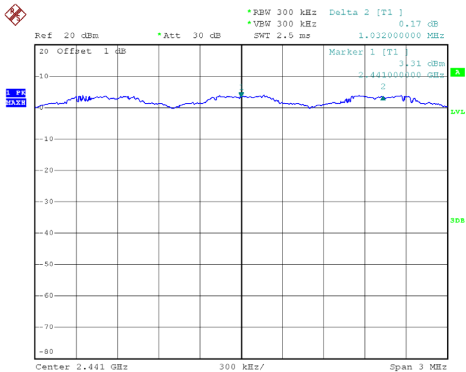
\pi/4 -DQPSK Mode, Middle Channel
