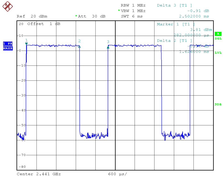
39 Channel @ 3DH3
