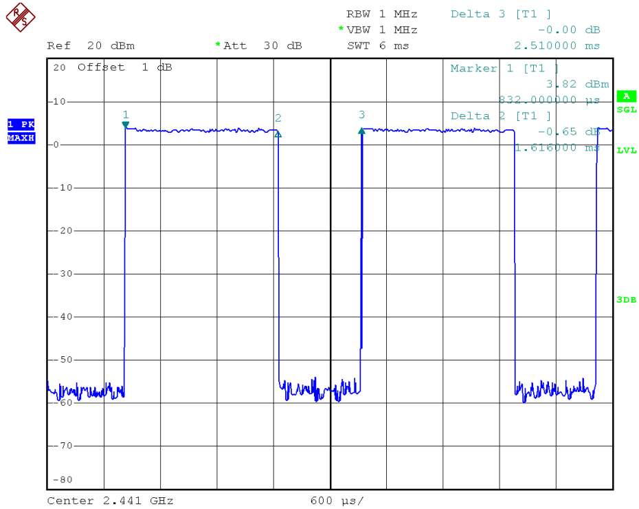
39 Channel @ 2DH3
