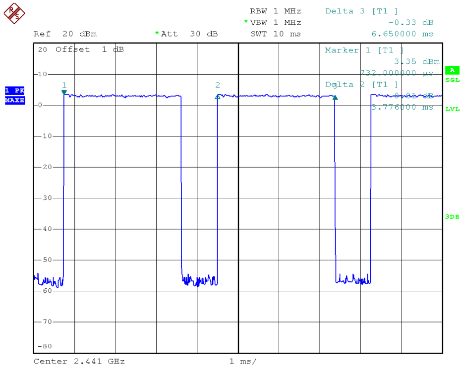
39 Channel @ 2DH5
