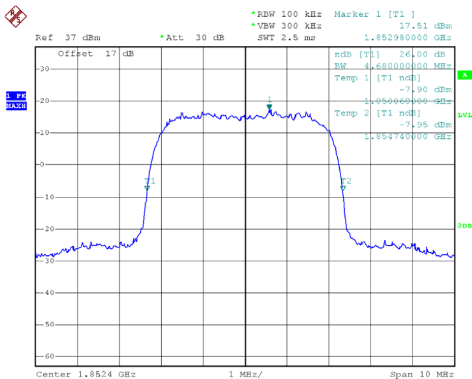
(Plot D1: WCDMA 1900MHz Channel = 9262 26dB bandwidth)
