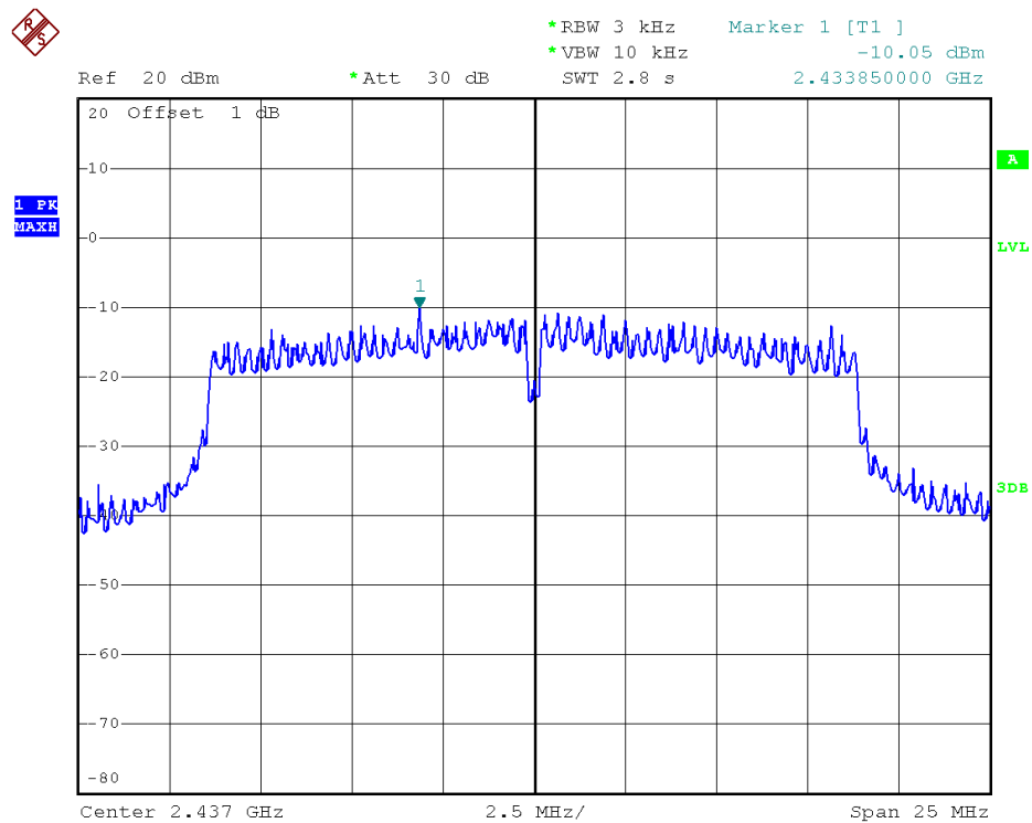
802.11n20 - Channel 6
