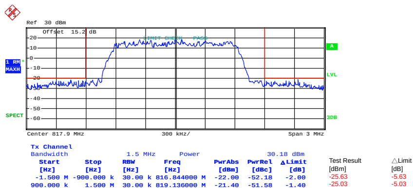
Lower Band Edge Plot on Channel 476 (817.90MHz)
