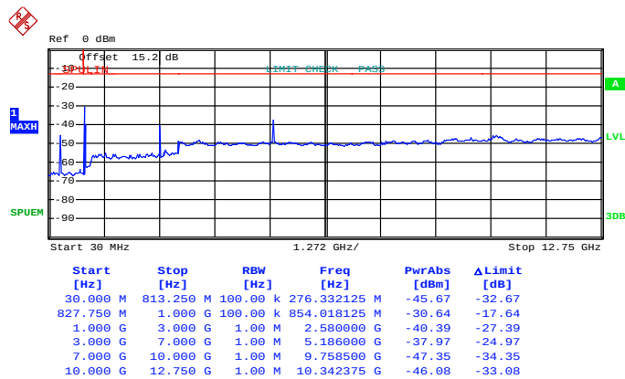
Conducted Emission Plot between on Channel 580 (820.50MHz)
