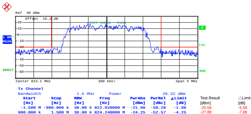
Higher Band Edge Plot on Channel 684 (823.10MHz)
