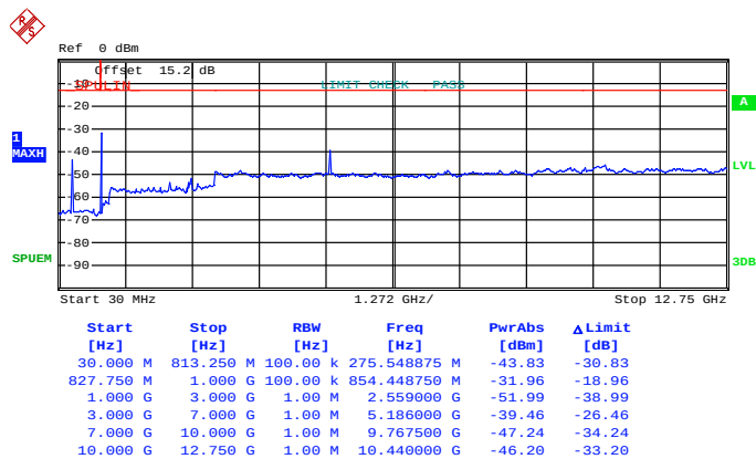
Conducted Emission Plot between on Channel 476 (817.90MHz)
