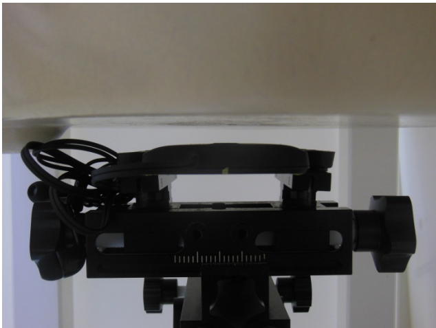
Back with headset of the DUT with Phantom 1 cm Gap
