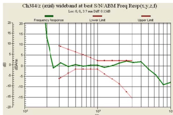
Fig 7.2 CDMA2000 BC0 Ch384
