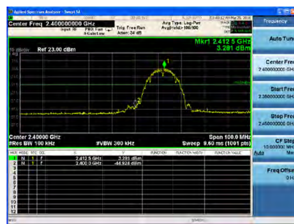
802.11b, Channel/Frequency: 1/2412
