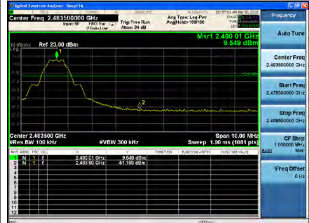
BLE, Channel/Frequency: 39/2480
