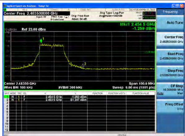
802.11g, Channel/Frequency: 11/2462
