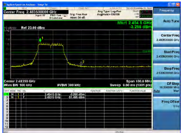
802.11n(HT20), Channel/Frequency: 11/2462
