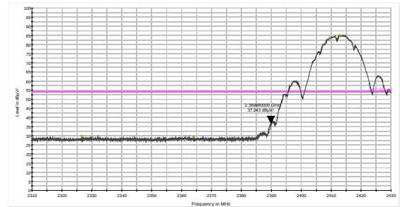
802.11b-Channel 1: Average
