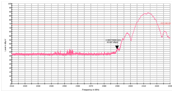
802.11b-Channel 1: Peak
