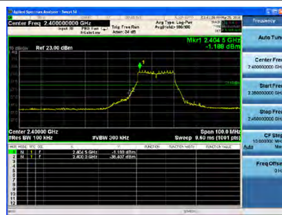
802.11g, Channel/Frequency: 1/2412
