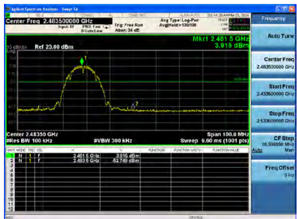
802.11b, Channel/Frequency: 11/2462
