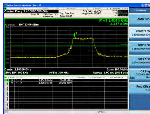
802.11n(HT20), Channel/Frequency: 1/2412
