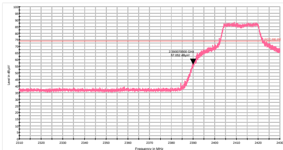
802.11g-Channel 1: Peak
