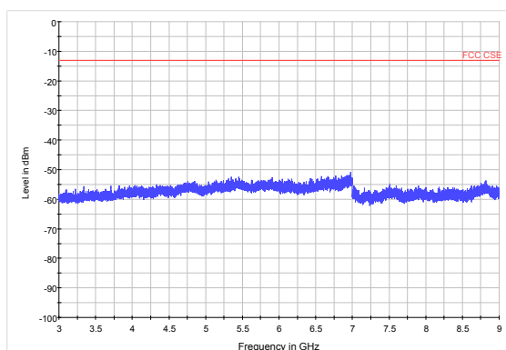
LTE Band 26 3MHz CH26915 3GHz~9GHz
