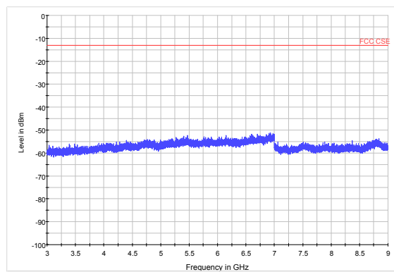
LTE Band 26 1.4MHz CH27033 3GHz~9GHz
