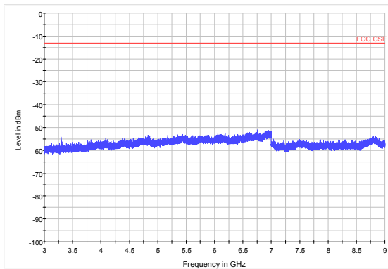
LTE Band 26 15MHz CH26865 3GHz~9GHz
