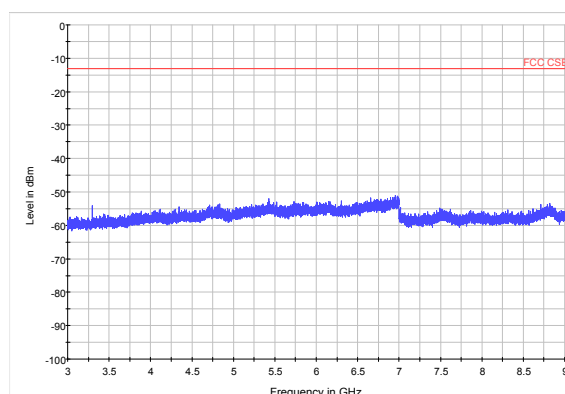
LTE Band 5 1.4MHz CH20407 3GHz~9GHz
