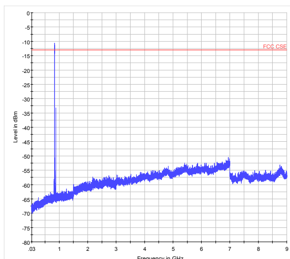
CDMA 1xRTT BC0 CH777 30MHz~9GHz
