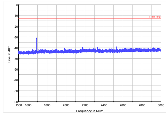
LTE Band 26 5MHz CH27015 1.5GHz~3GHz
