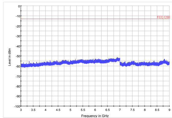
LTE Band 5 3MHz CH20525 3GHz~9GHz
