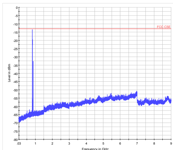
CDMA 1xRTT BC0 CH384 30MHz~9GHz
