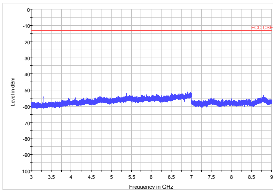
LTE Band 5 3MHz CH20415 3GHz~9GHz
