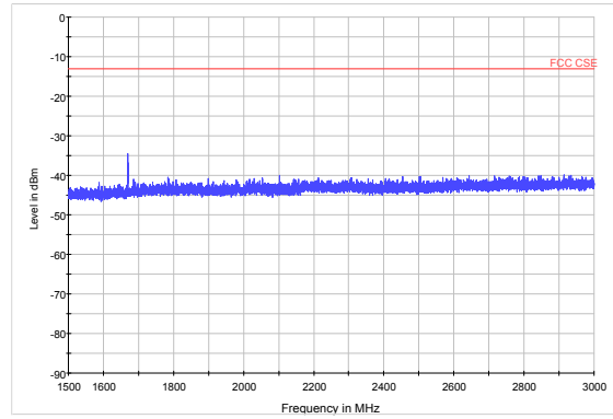
LTE Band 26 15MHz CH26965 1.5GHz~3GHz
