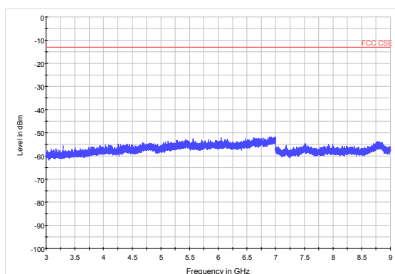
LTE Band 26 3MHz CH26805 3GHz~9GHz
