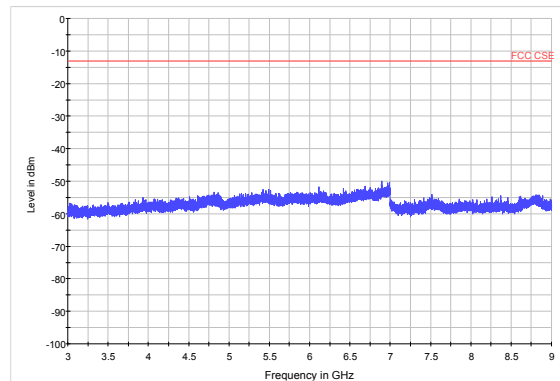
LTE Band 26 5MHz CH26915 3GHz~9GHz
