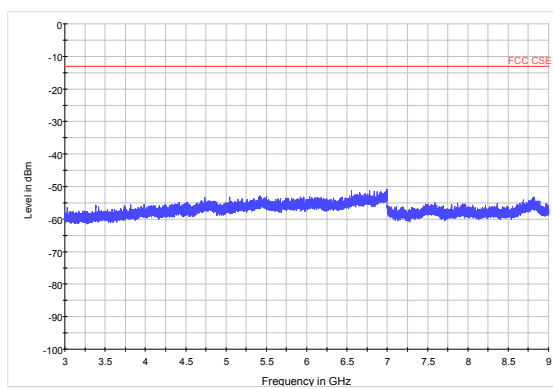
LTE Band 5 3MHz CH20635 3GHz~9GHz
