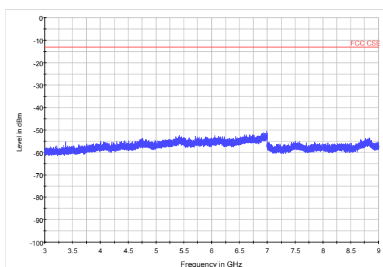
LTE Band 26 10MHz CH26990 3GHz~9GHz
