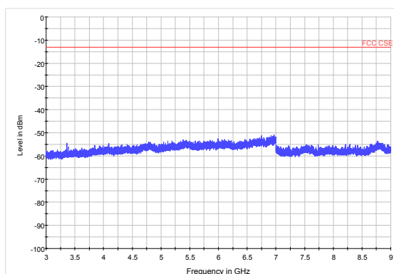
LTE Band 26 10MHz CH26915 3GHz~9GHz
