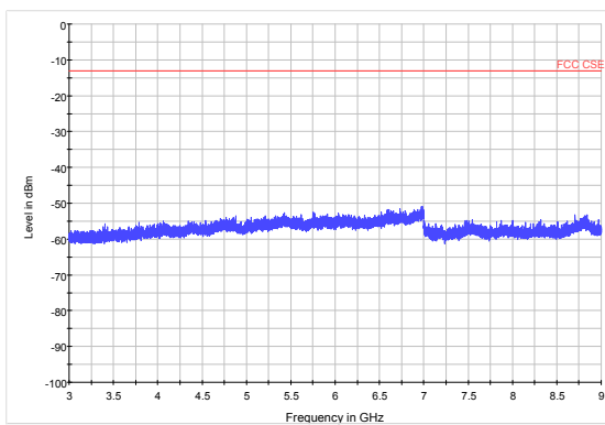
LTE Band 26 1.4MHz CH26915 3GHz~9GHz
