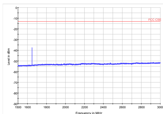
LTE Band 5 1.4MHz CH20407 1.5GHz~3GHz
