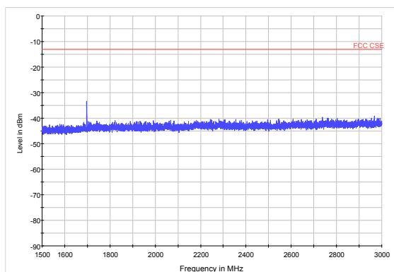
LTE Band 26 10MHz CH26990 1.5GHz~3GHz
