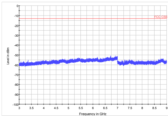
LTE Band 26 15MHz CH26965 3GHz~9GHz
