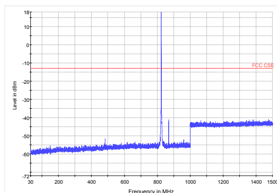
LTE Band 5 1.4MHz CH20407 30MHz~1.5GHz
