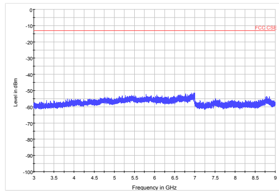
LTE Band 26 15MHz CH26915 3GHz~9GHz
