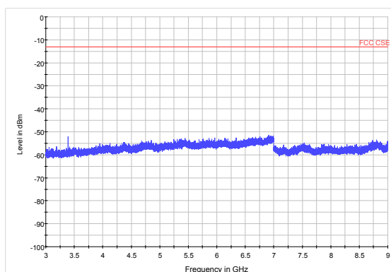
LTE Band 5 1.4MHz CH20643 3GHz~9GHz
