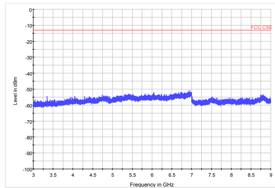
LTE Band 5 10MHz CH20525 3GHz~9GHz
