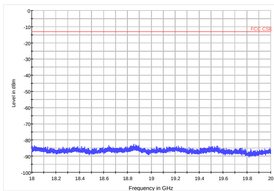
LTE Band 2 15MHz CH18675 18GHz~20GHz
