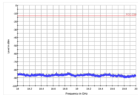
LTE Band 25 10MHz CH26090 18GHz~20GHz
