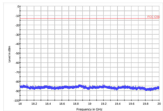
LTE Band 2 15MHz CH18900 18GHz~20GHz
