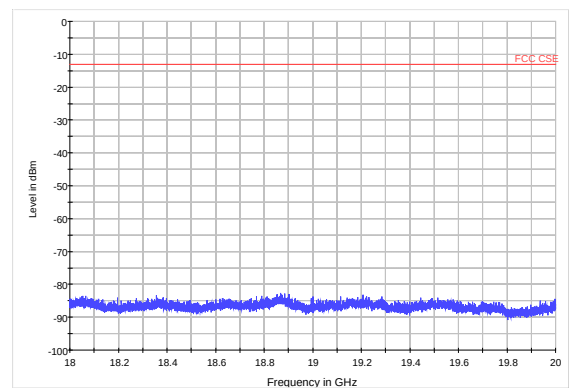
LTE Band 2 10MHz CH19150 18GHz~20GHz
