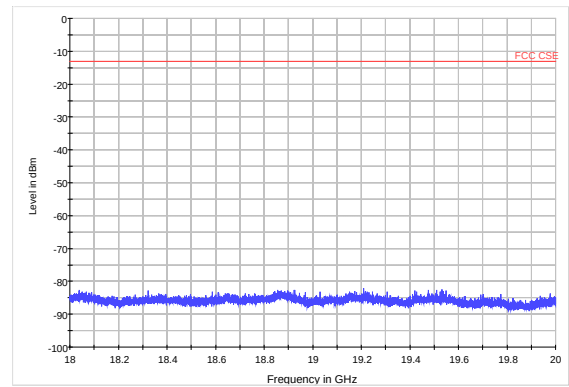
LTE Band 2 1.4MHz CH18900 18GHz~20GHz
