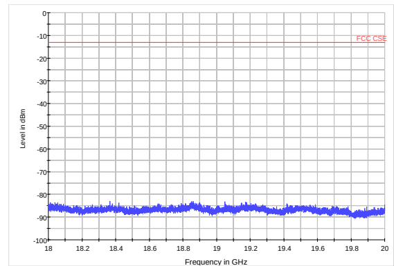
LTE Band 25 1.4MHz CH26365 18GHz~20GHz
