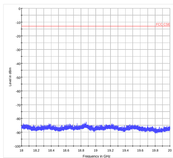
CDMA BC1 1xRTT CH1175 18GHz~20GHz
