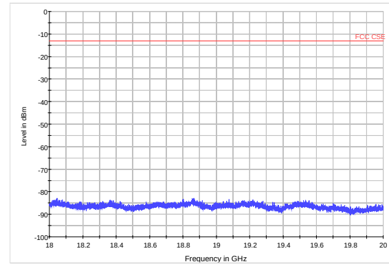
WCDMA Band II CH9538 18GHz~20GHz
