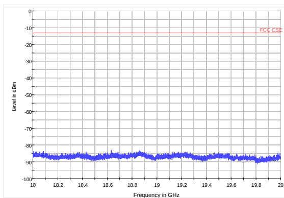
LTE Band 25 10MHz CH26365 18GHz~20GHz
