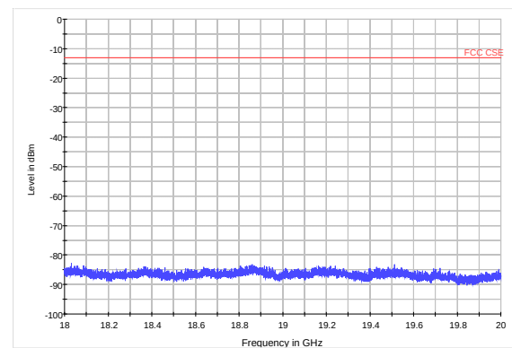
LTE Band 2 5MHz CH18900 18GHz~20GHz
