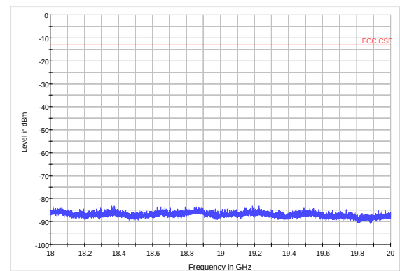
LTE Band 25 3MHz CH26055 18GHz~20GHz
