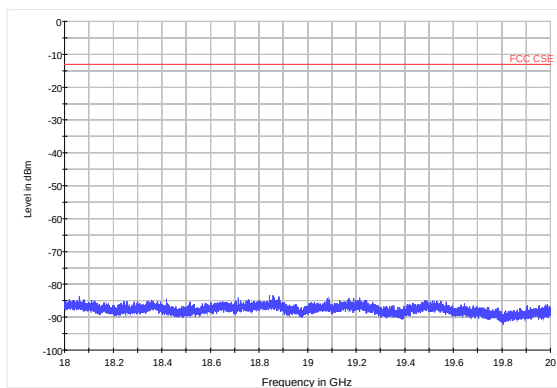
LTE Band 25 15MHz CH26615 18GHz~20GHz
