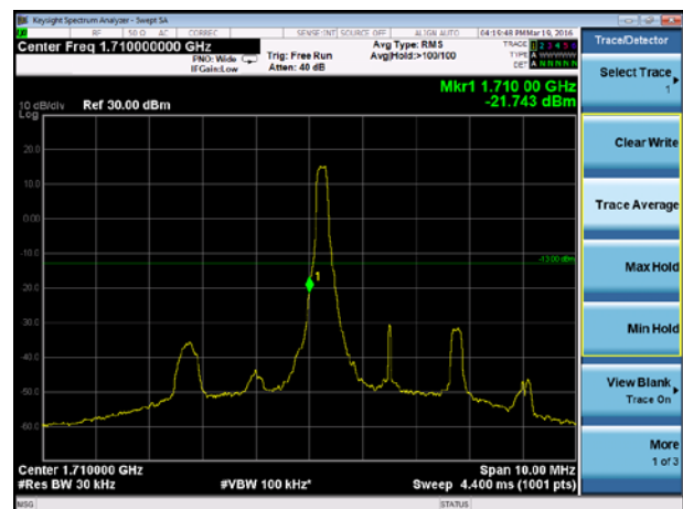
LTE Band 4 16QAM Bandwidth = 3MHz CH19965, RB 15
