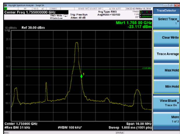
LTE Band 4 16QAM Bandwidth = 5MHz CH20375, RB 25
