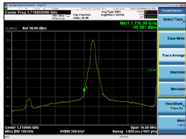
LTE Band 4 16QAM Bandwidth = 10MHz CH20000, RB 50
