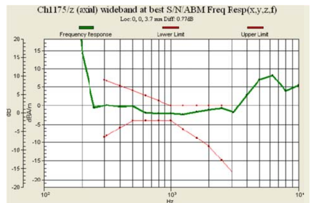
Fig 8.6 CDMA2000 BC1 Ch1175
