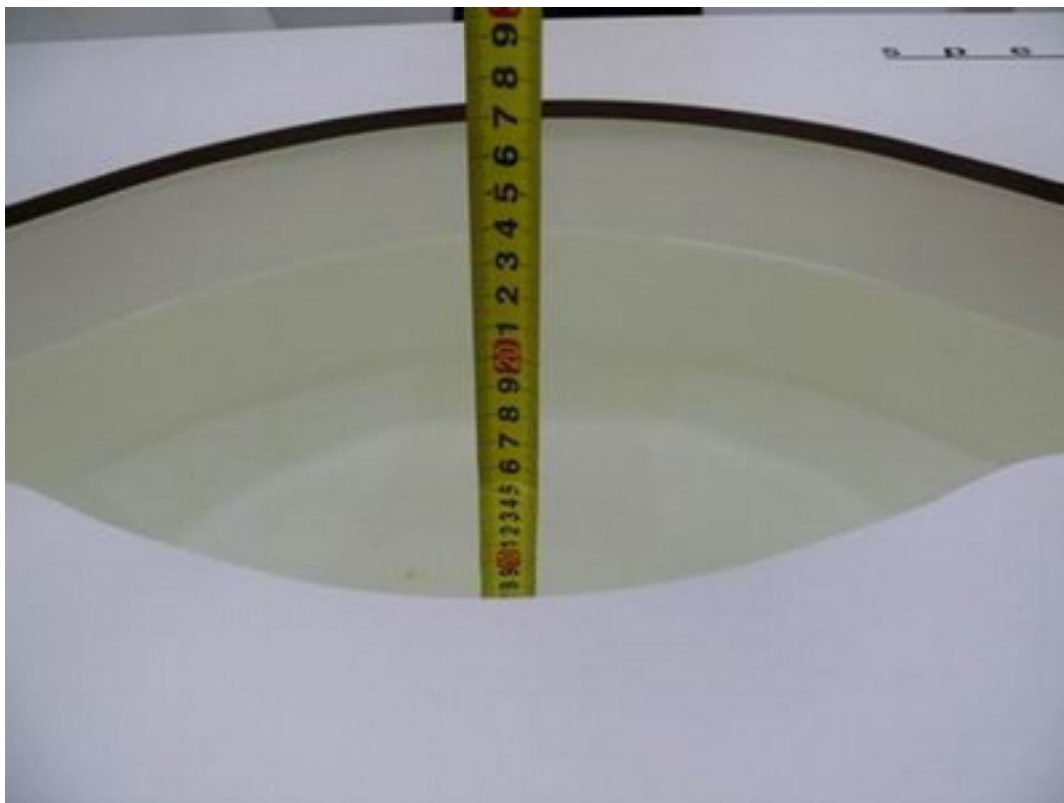
Picture 13: Liquid depth in the flat Phantom (2600 MHz, 15.3cm depth)
