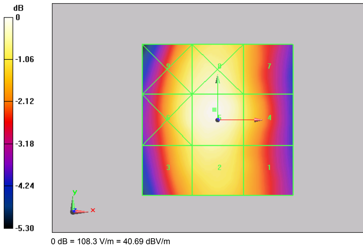
Figure 15 HAC RF E-Field CDMA BC0 Channel 384
