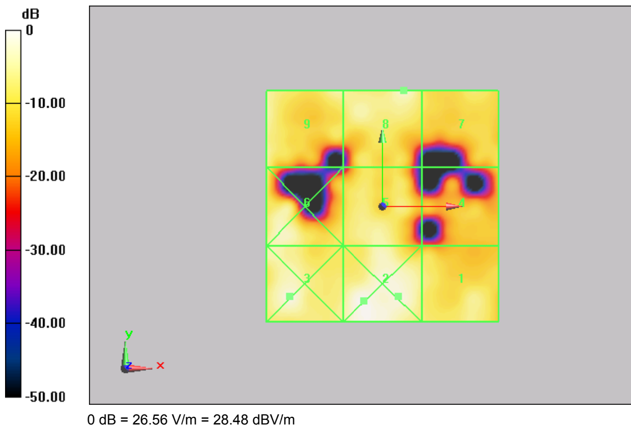
Figure 17 HAC RF E-Field CDMA BC1 Channel 1175
