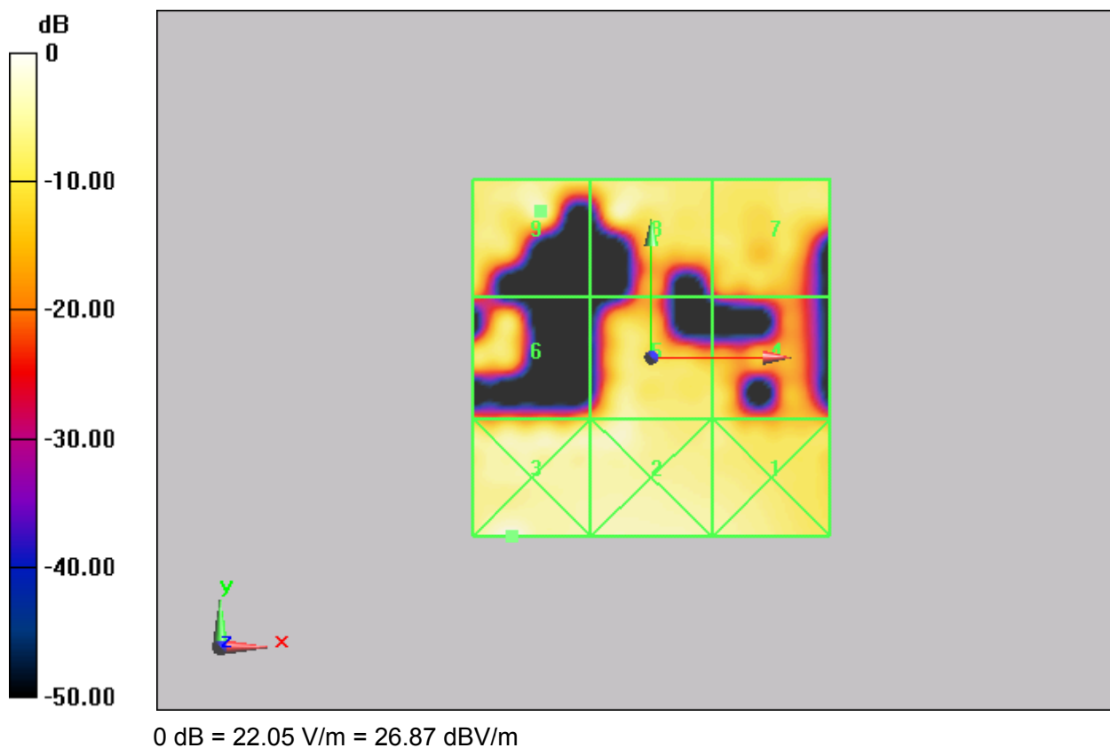
Figure 18 HAC RF E-Field CDMA BC1 Channel 600
