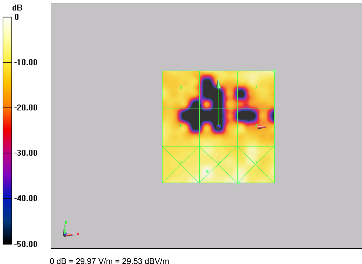
Figure 19 HAC RF E-Field CDMA BC1 Channel 25
