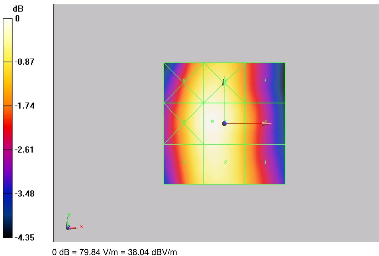
Figure 8 HAC RF E-Field GSM 850 Channel 251
