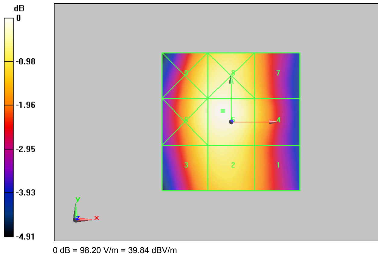
Figure 14 HAC RF E-Field CDMA BC0 Channel 777
