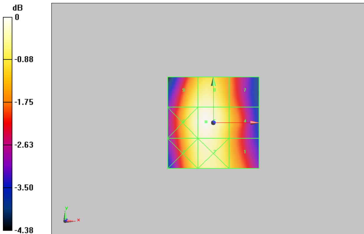
Figure 10 HAC RF E-Field GSM 850 Channel 128
