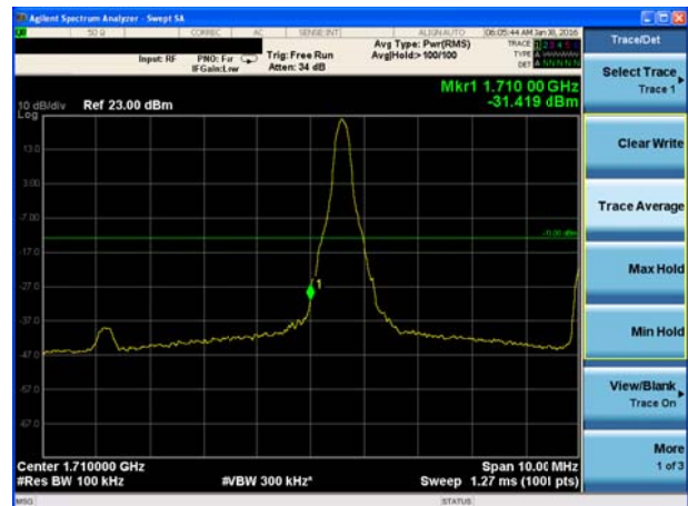
LTE Band 4 16QAM Bandwidth = 10MHz CH20000, RB 50
