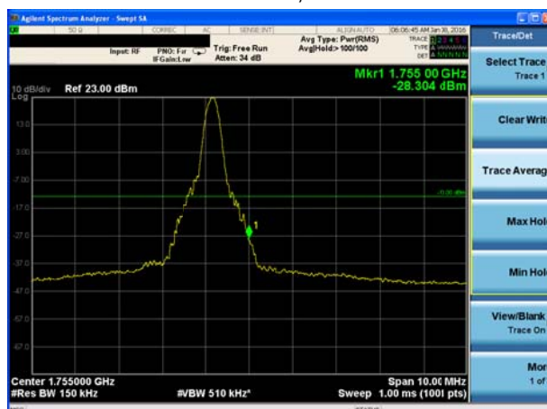
LTE Band 4 16QAM Bandwidth = 15MHz CH20325, RB 75
