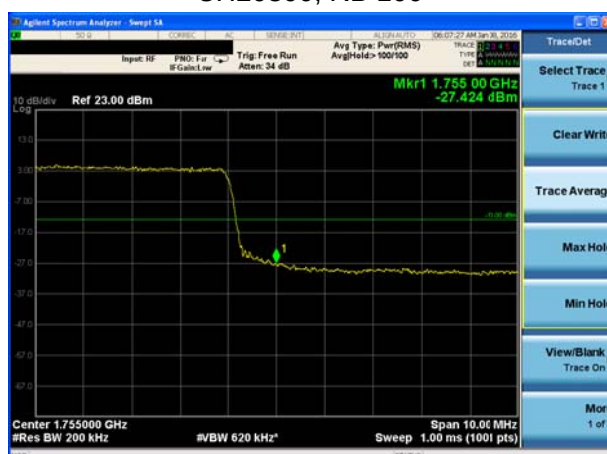
LTE Band 4 16QAM Bandwidth = 20MHz CH20300, RB 100
