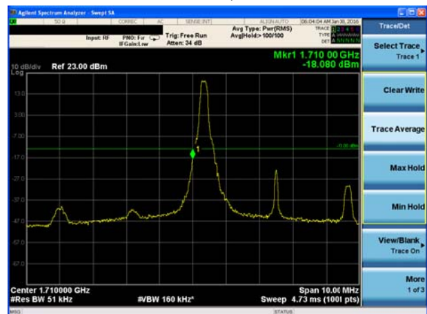
LTE Band 4 16QAM Bandwidth = 5MHz CH19975, RB 1
