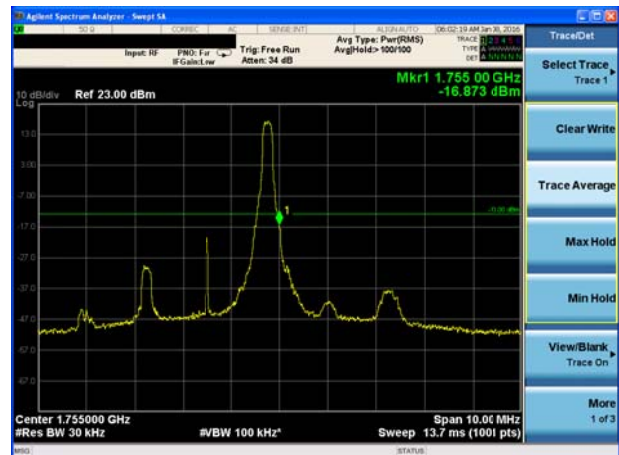
LTE Band 4 16QAM Bandwidth = 3MHz CH20385, RB 15
