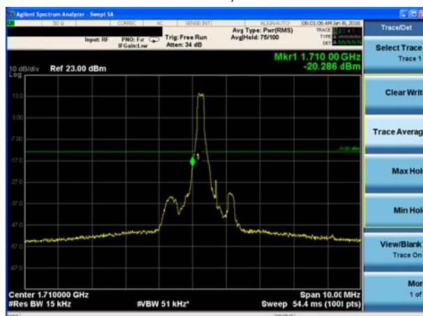
LTE Band 4 16QAM Bandwidth = 1.4MHz CH19957, RB 6
