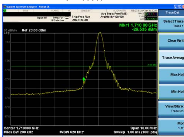
LTE Band 4 16QAM Bandwidth = 20MHz CH20050, RB 1
