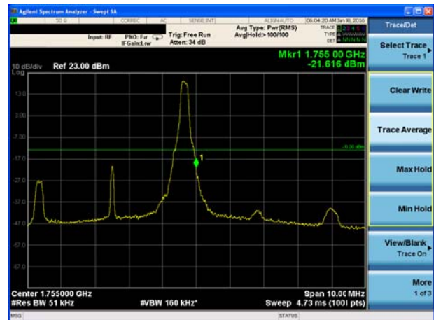
LTE Band 4 16QAM Bandwidth = 5MHz CH20375, RB 25
