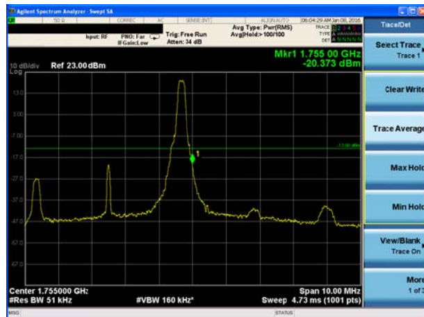
LTE Band 4 QPSK Bandwidth = 5MHz CH20375, RB 25
