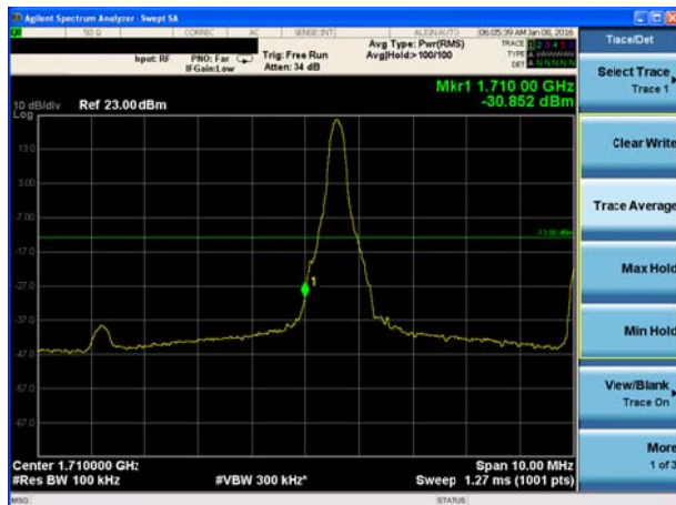
LTE Band 4 QPSK Bandwidth = 10MHz CH20000, RB 50
