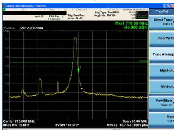
LTE Band 12 QPSK Bandwidth = 3MHz CH23165, RB 15
