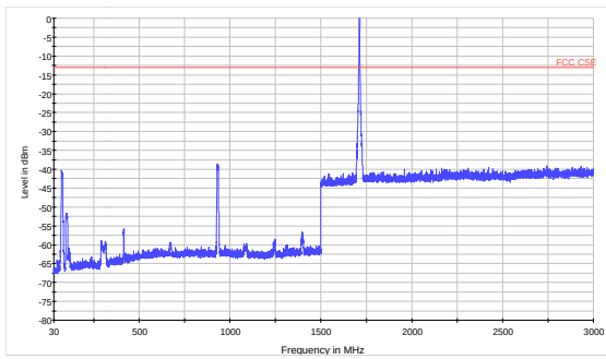
WCDMA Band IV Channel1312 30MHz~3GHz
