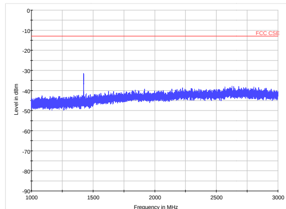
LTE Band 12 CH23155 1GHz~3GHz
