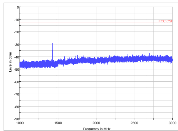
LTE Band 12 CH23173 1GHz~3GHz
