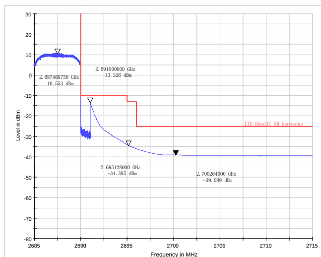
LTE Band 41 QPSK Bandwidth = 5MHz CH41565, RB 25
