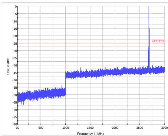
LTE Band 41 CH41565 30MHz~3GHz
