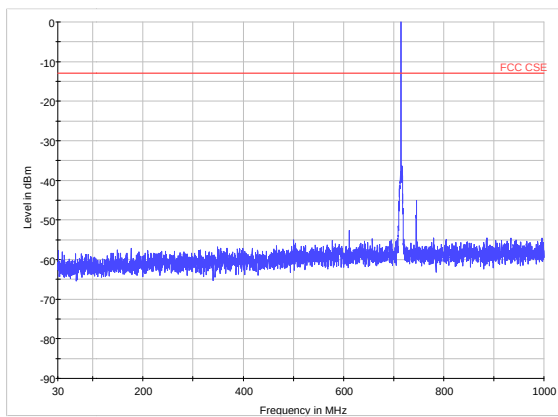
LTE Band 12 CH23173 30MHz~1GHz
