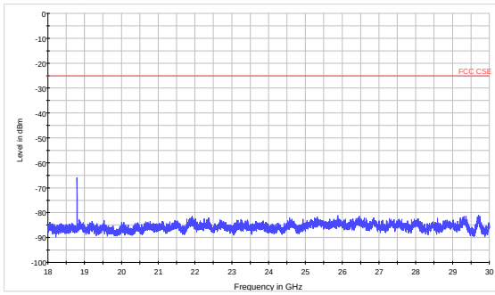
LTE Band 41 CH1540 18GHz~30GHz
