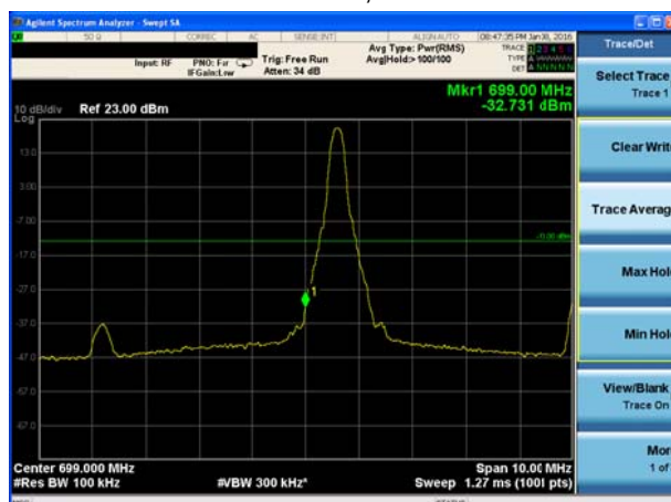
LTE Band 12 16QAM Bandwidth = 10MHz CH23060, RB 50
