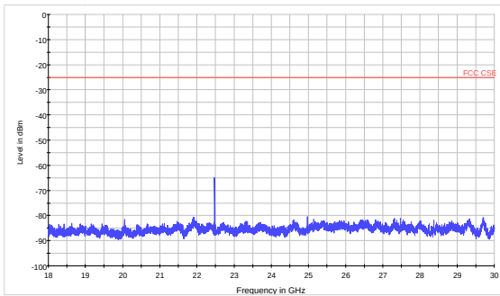
LTE Band 41 CH39750 18GHz~30GHz
