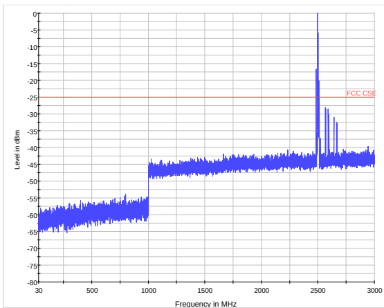
LTE Band 41 CH39725 30MHz~3GHz
