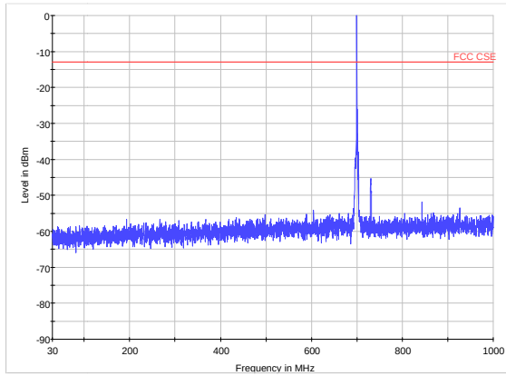
LTE Band 12 CH23025 30MHz~1GHz
