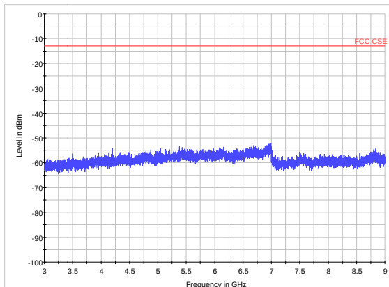
LTE Band 12 CH23035 3GHz~9GHz
