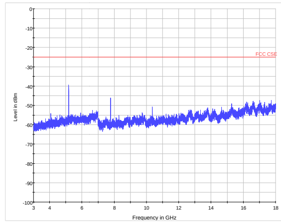
LTE Band 41 CH40620 3GHz~18GHz
