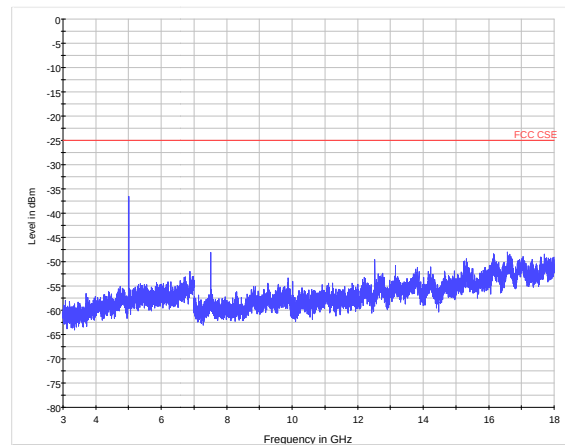
LTE Band 41 CH39700 3GHz~18GHz
