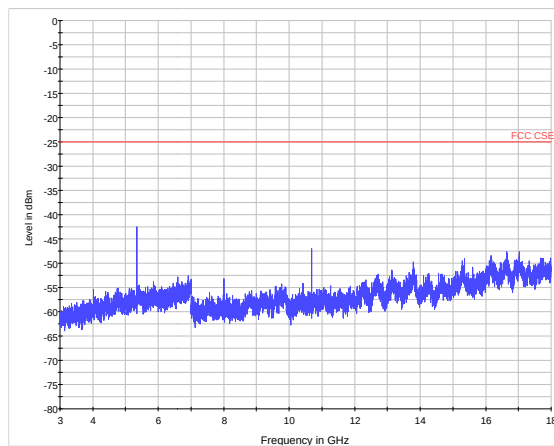
LTE Band 41 CH41490 3GHz~18GHz
