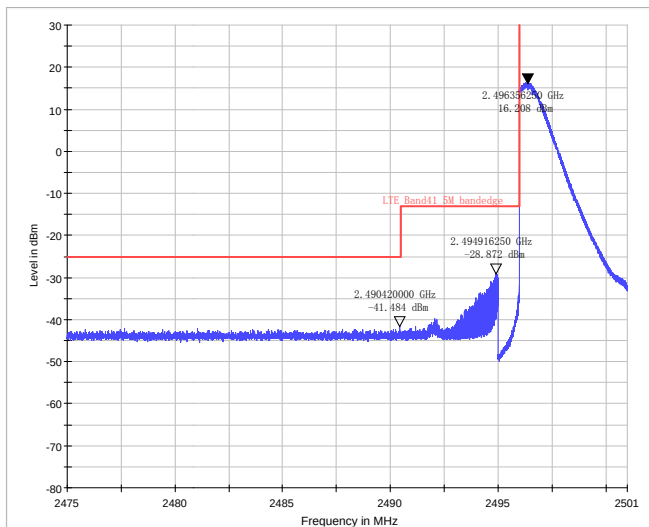
LTE Band 41 16QAM Bandwidth = 5MHz CH39675, RB 1
