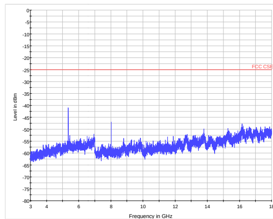
LTE Band 41 CH41515 3GHz~18GHz
