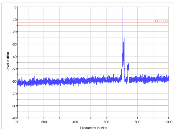
LTE Band 12 CH23130 30MHz~1GHz
