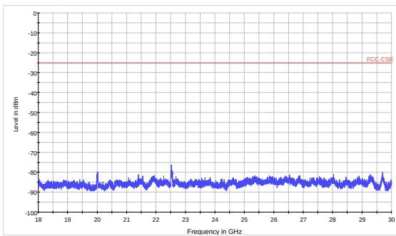
LTE Band 41 CH39725 18GHz~30GHz
