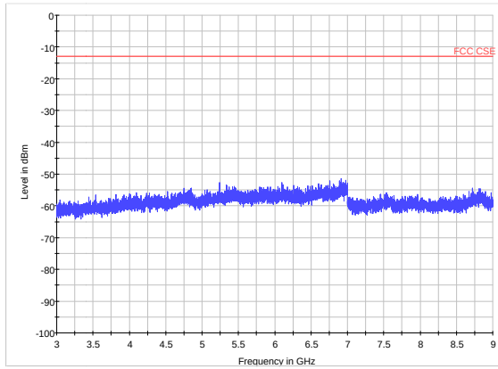
LTE Band 12 CH23155 3GHz~9GHz
