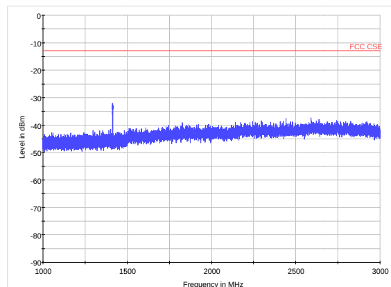
LTE Band 12 CH23130 1GHz~3GHz
