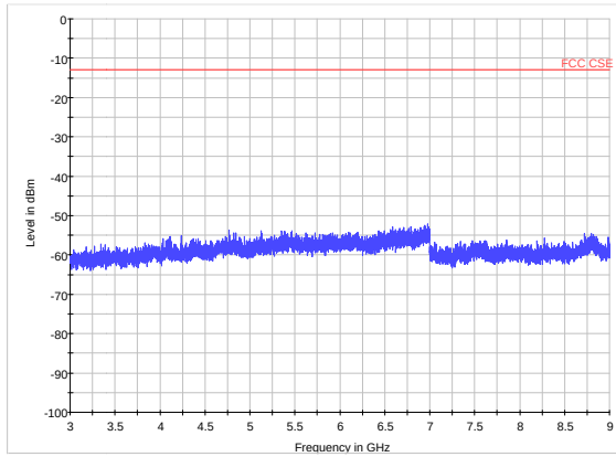
LTE Band 12 CH23130 3GHz~9GHz
