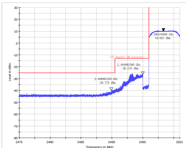
LTE Band 41 QPSK Bandwidth = 5MHz CH39675, RB 25
