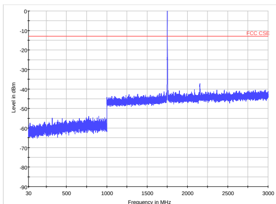
LTE Band 4 CH20385 30MHz~3GHz
