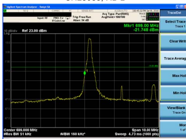
LTE Band 12 16QAM Bandwidth = 5MHz CH23035, RB 1
