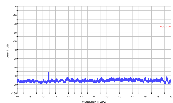
LTE Band 41 CH39675 18GHz~30GHz
