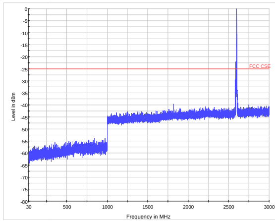
LTE Band 41 CH40620 30MHz~3GHz
