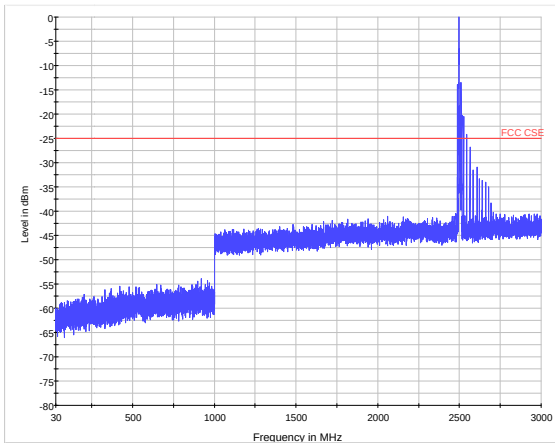
LTE Band 41 CH39750 30MHz~3GHz
