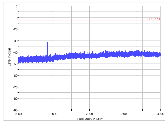
LTE Band 12 CH23095 1GHz~3GHz
