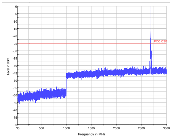
LTE Band 41 CH41540 30MHz~3GHz
