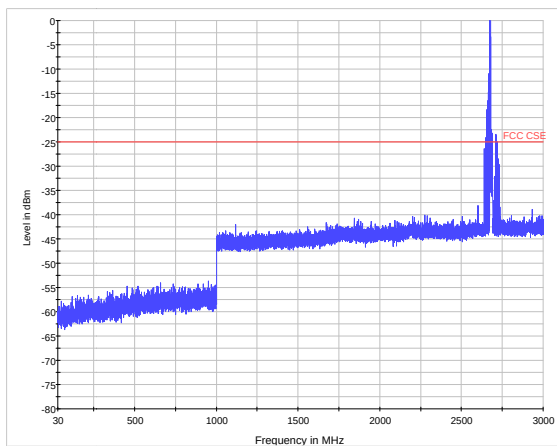
LTE Band 41 CH41515 30MHz~3GHz
