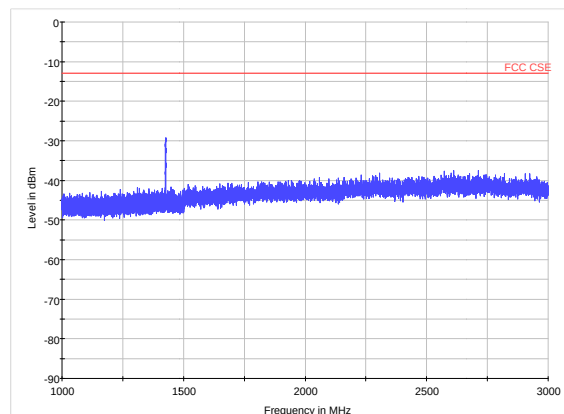
LTE Band 12 CH23165 1GHz~3GHz
