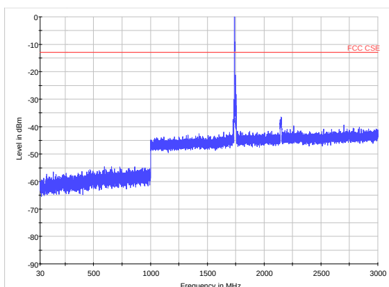
LTE Band 4 CH20325 30MHz~3GHz
