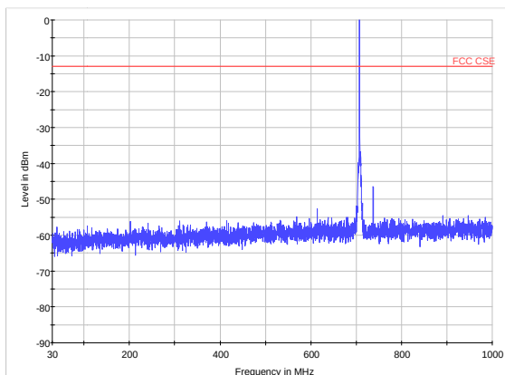
LTE Band 12 CH23095 30MHz~1GHz
