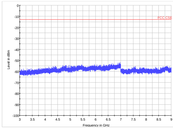
LTE Band 12 CH23165 3GHz~9GHz
