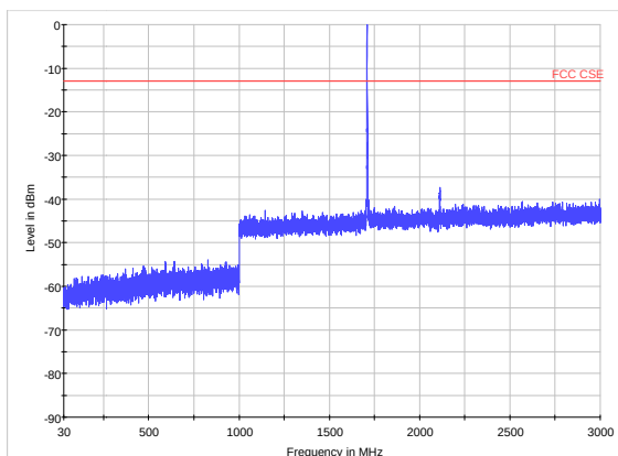
LTE Band 4 CH19965 30MHz~3GHz
