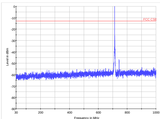
LTE Band 12 CH23165 30MHz~1GHz
