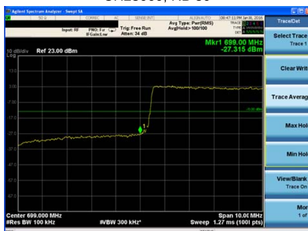
LTE Band 12 16QAM Bandwidth = 10MHz CH23130, RB 1
