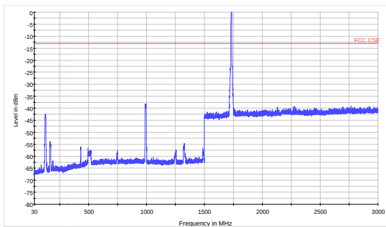
WCDMA Band IV Channel1413 30MHz~3GHz
