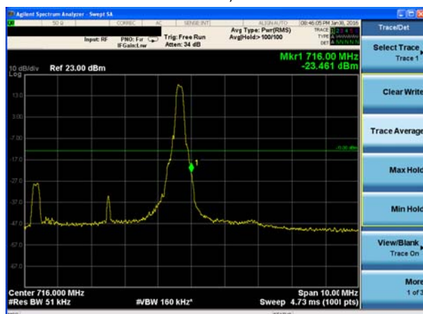
LTE Band 12 16QAM Bandwidth = 5MHz CH23155, RB 25
