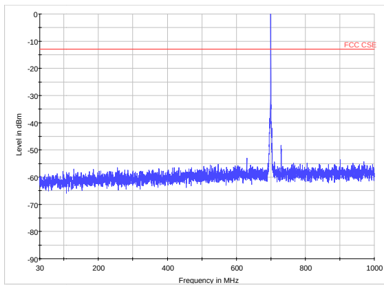
LTE Band 12 CH23017 30MHz~1GHz
