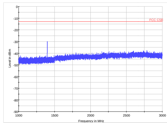
LTE Band 12 CH23035 1GHz~3GHz
