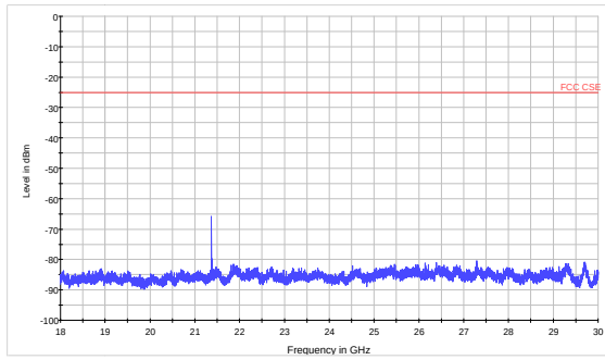
LTE Band 41 CH41490 18GHz~30GHz
