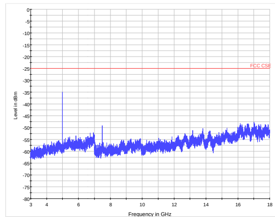
LTE Band 41 CH39725 3GHz~18GHz
