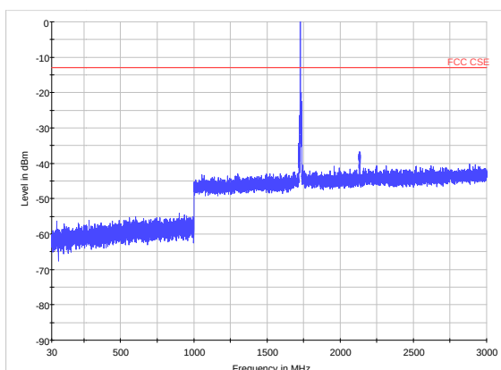
LTE Band 4 CH20175 30MHz~3GHz
