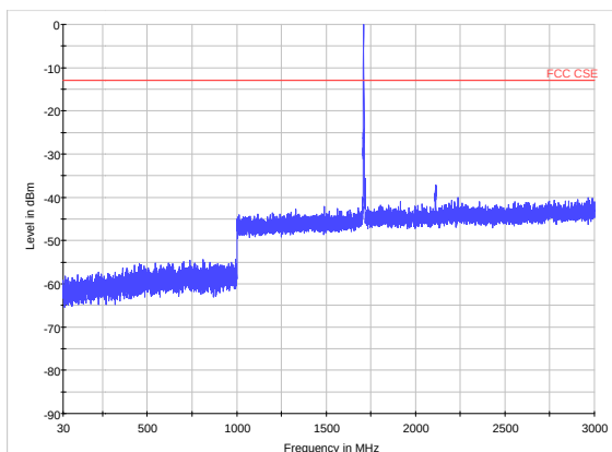
LTE Band 4 CH19975 30MHz~3GHz
