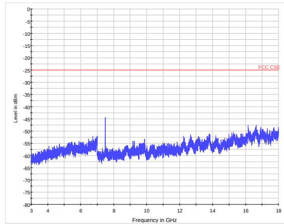
LTE Band CH427235 3GHz~18GHz
