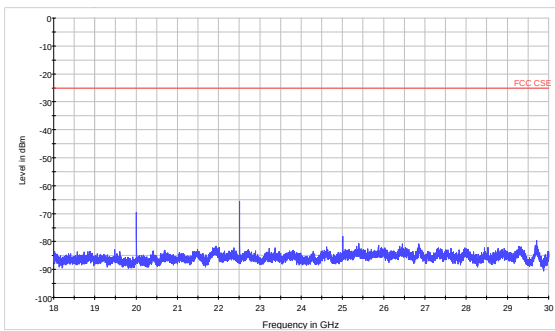
LTE Band 41 CH39700 18GHz~30GHz
