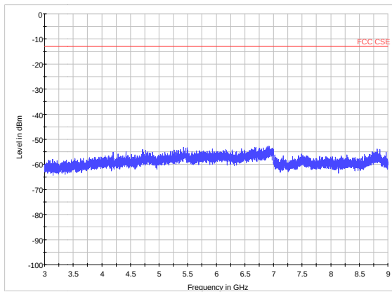
LTE Band 12 CH23060 3GHz~9GHz
