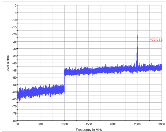
LTE Band 41 CH39675 30MHz~3GHz
