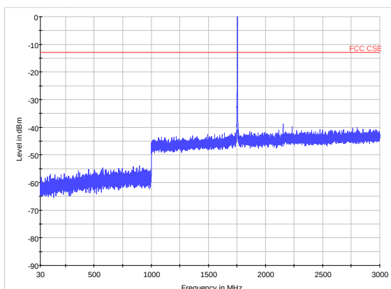
LTE Band 4 CH20393 30MHz~3GHz
