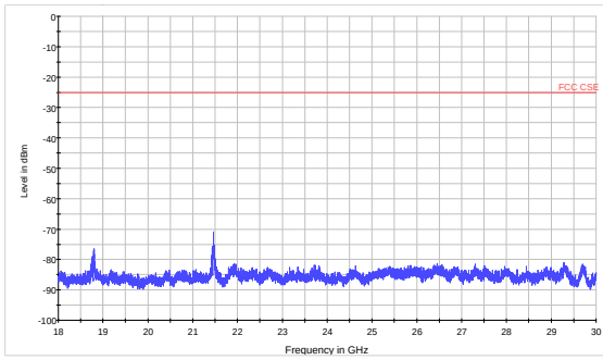
LTE Band 41 CH41515 18GHz~30GHz
