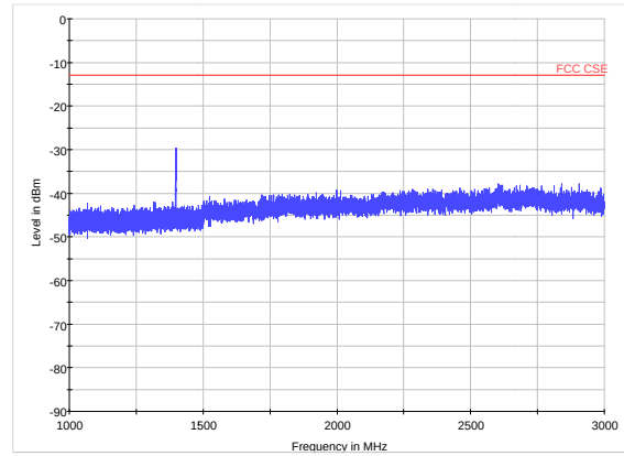
LTE Band 12 CH23025 1GHz~3GHz
