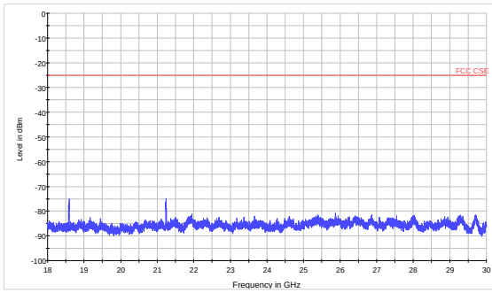
LTE Band 41 CH41565 18GHz~30GHz
