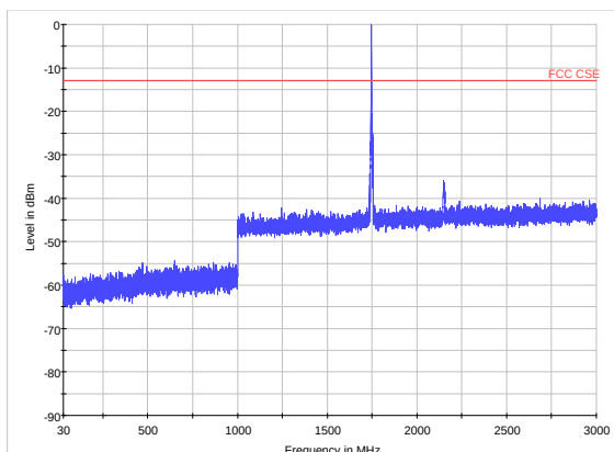
LTE Band 4 CH20350 30MHz~3GHz
