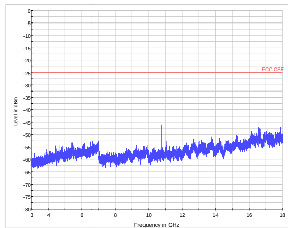
LTE Band 41 CH41540 3GHz~18GHz
