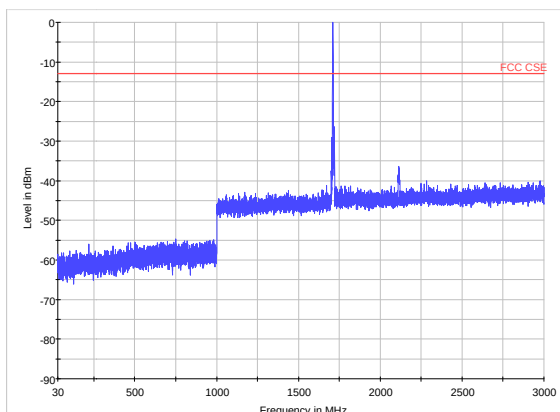
LTE Band 4 CH20000 30MHz~3GHz
