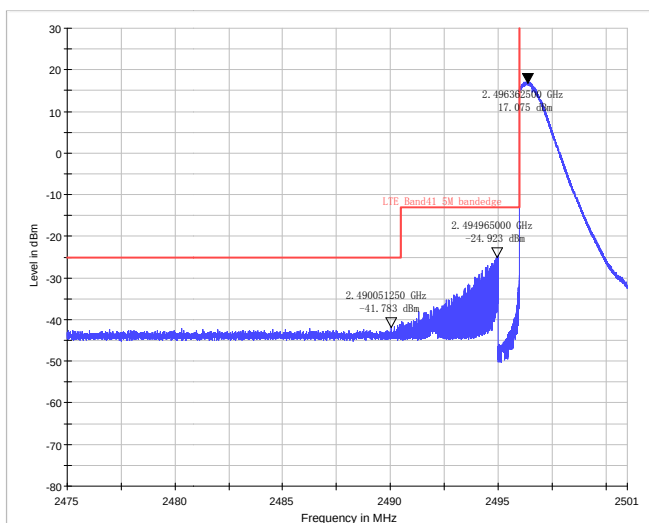
LTE Band 41 QPSK Bandwidth = 5MHz CH39675, RB 1
