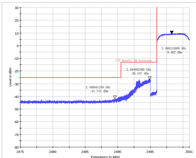
LTE Band 41 16QAM Bandwidth = 5MHz CH39675, RB 25
