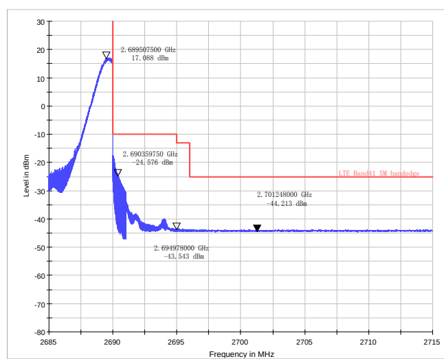
LTE Band 41 QPSK Bandwidth = 5MHz CH41565, RB 1
