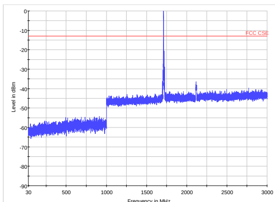
LTE Band 4 CH20025 30MHz~3GHz
