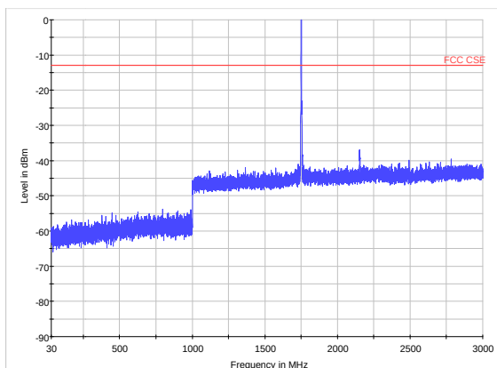
LTE Band 4 CH20375 30MHz~3GHz
