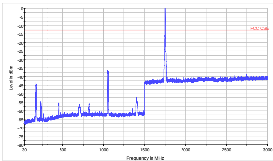
WCDMA Band IV Channel1513 30MHz~3GHz
