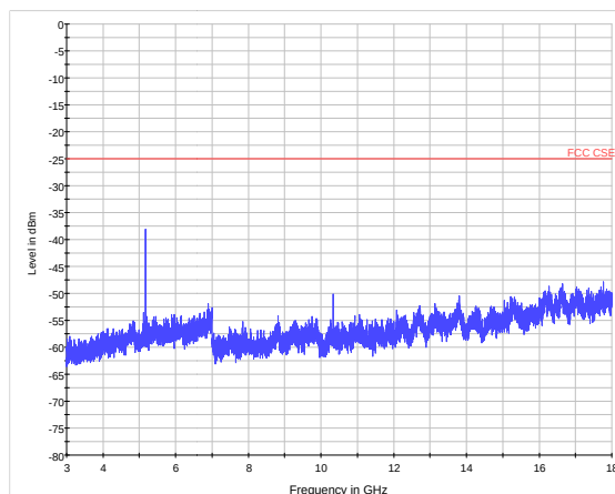
LTE Band 41 CH40620 3GHz~18GHz
