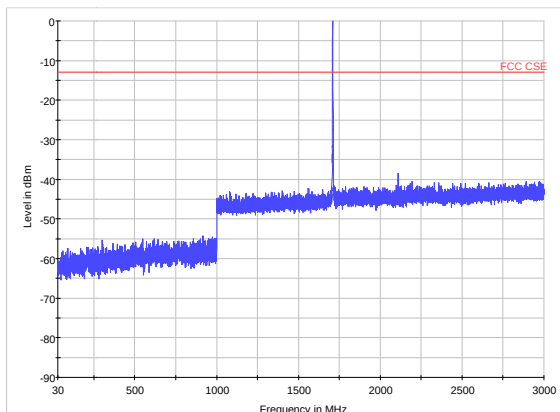
LTE Band 4 CH19957 30MHz~3GHz
