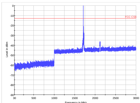
LTE Band 4 CH20050 30MHz~3GHz
