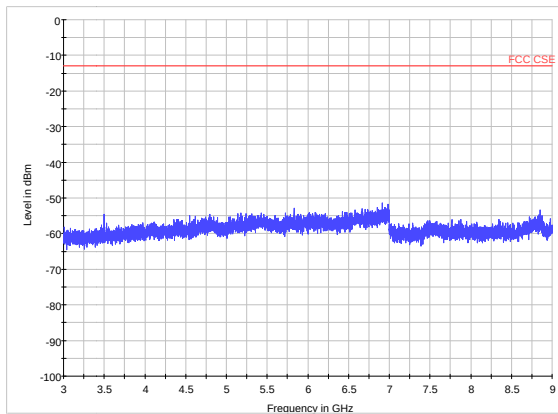
LTE Band 12 CH23025 3GHz~9GHz
