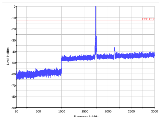
LTE Band 4 CH20300 30MHz~3GHz
