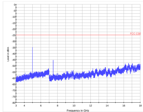
LTE Band 41 CH39750 3GHz~18GHz
