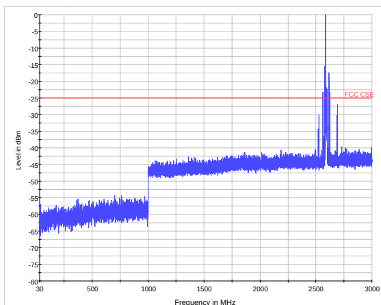
LTE Band 41 CH40620 30MHz~3GHz
