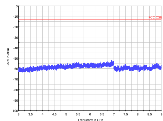
LTE Band 12 CH23173 3GHz~9GHz
