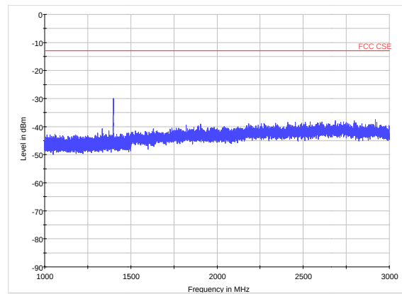
LTE Band 12 CH23017 1GHz~3GHz
