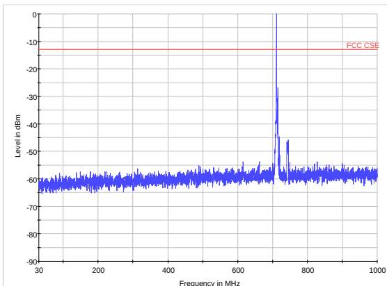
LTE Band 12 CH23155 30MHz~1GHz
