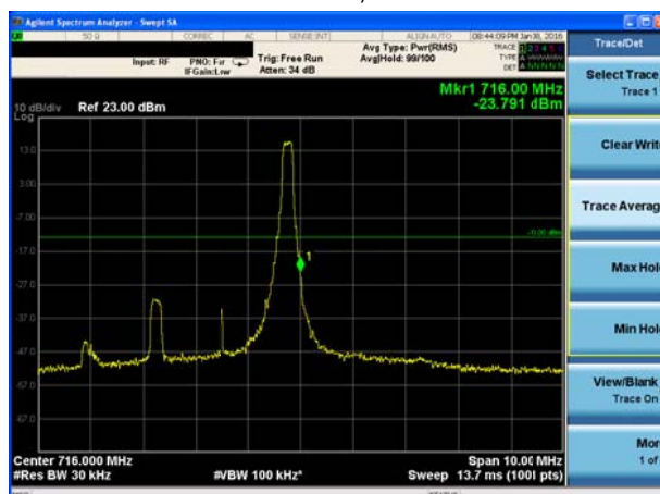
LTE Band 12 16QAM Bandwidth = 3MHz CH23165, RB 15
