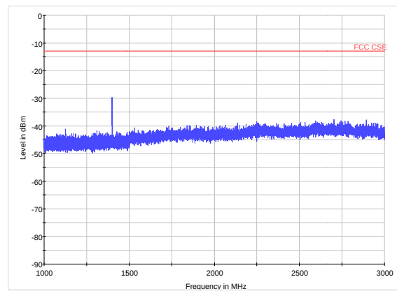
LTE Band 12 CH23060 1GHz~3GHz
