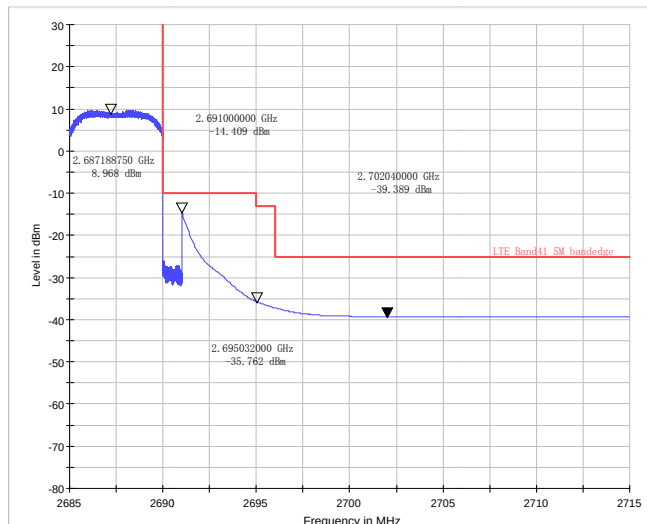
LTE Band 41 16QAM Bandwidth = 5MHz CH41565, RB 25
