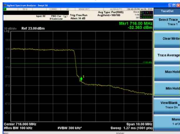
LTE Band 12 QPSK Bandwidth = 10MHz CH23130, RB 50
