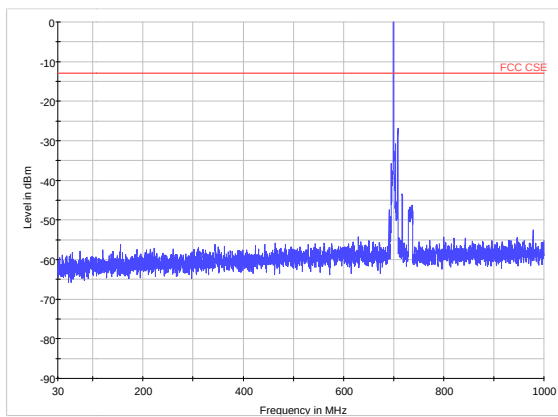
LTE Band 12 CH23060 30MHz~1GHz
