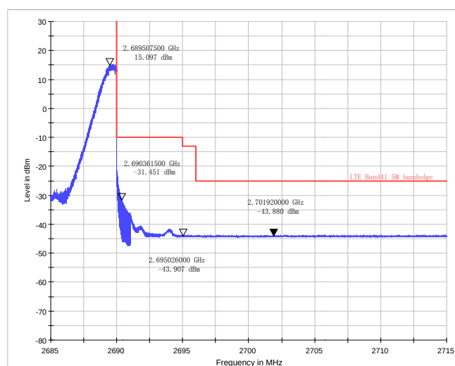
LTE Band 41 16QAM Bandwidth = 5MHz CH41565, RB 1
