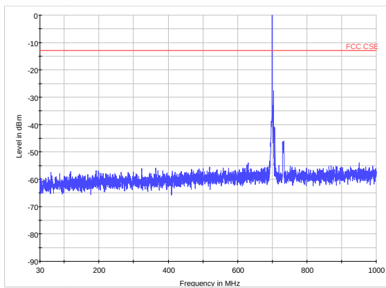
LTE Band 12 CH23035 30MHz~1GHz
