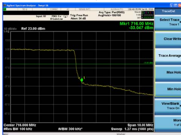
LTE Band 12 16QAM Bandwidth = 10MHz CH23130, RB 50
