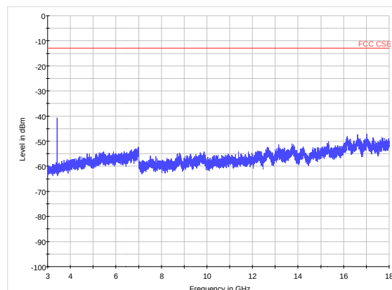
LTE Band 4 CH20025 3GHz~18GHz
