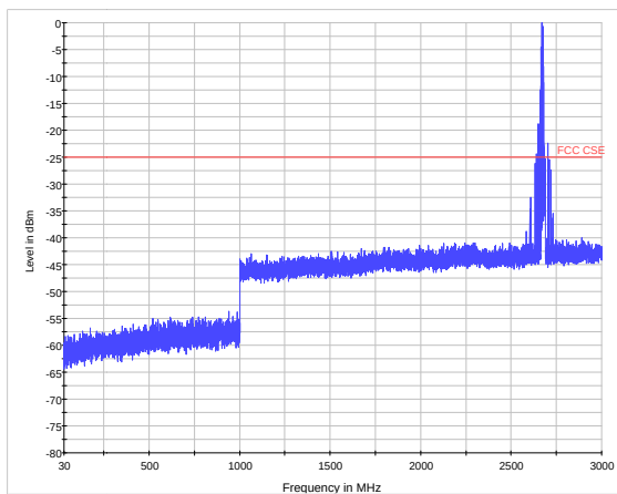
LTE Band 41 CH41490 30MHz~3GHz
