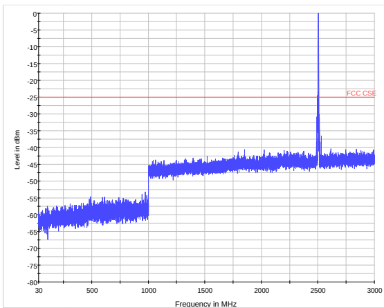
LTE Band 41 CH39700 30MHz~3GHz
