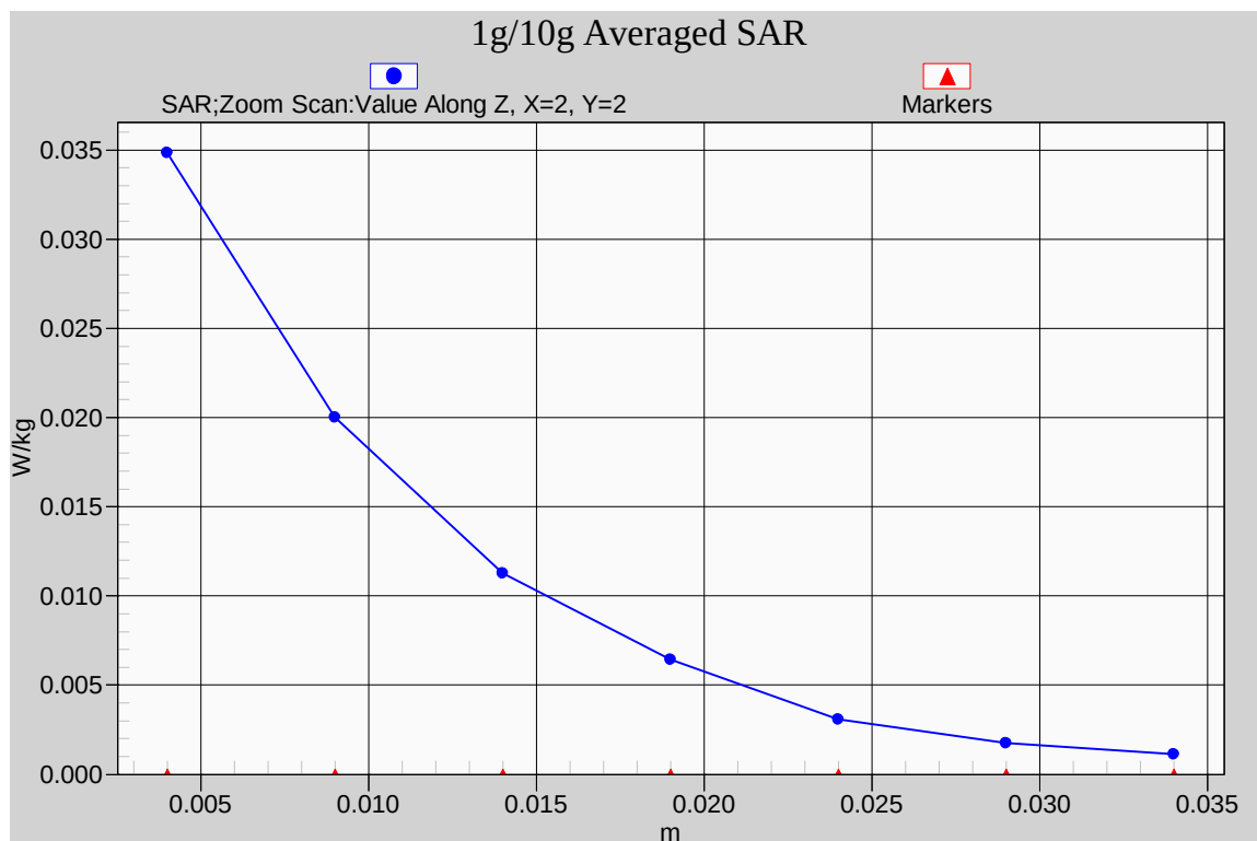
Fig. 5-1 Z-Scan at power reference point (2450 MHz CH11)
