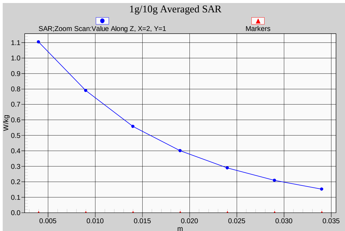
Fig. 2-1 Z-Scan at power reference point (850MHz CH251)
