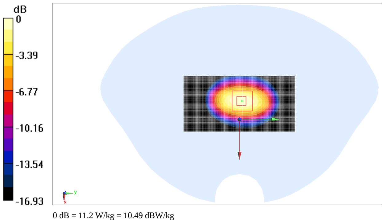
Fig.B.4 validation 1900MHz 250Mw
