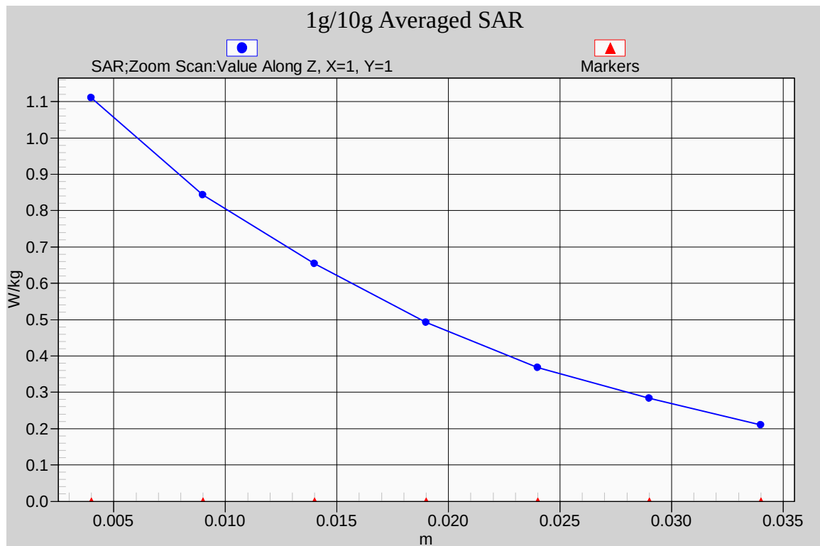
Fig. 1-1 Z-Scan at power reference point (850MHz CH190)
