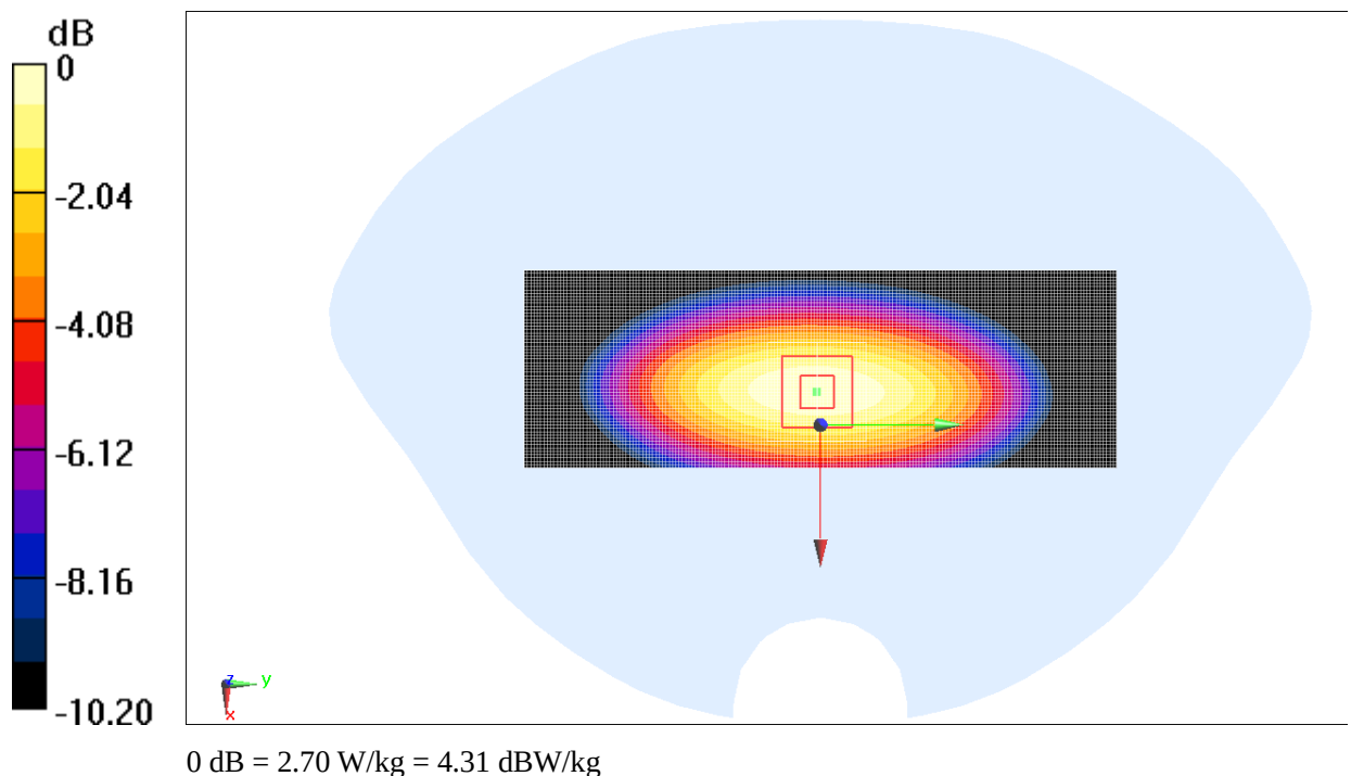
Fig.B.2 validation 835MHz 250mW
