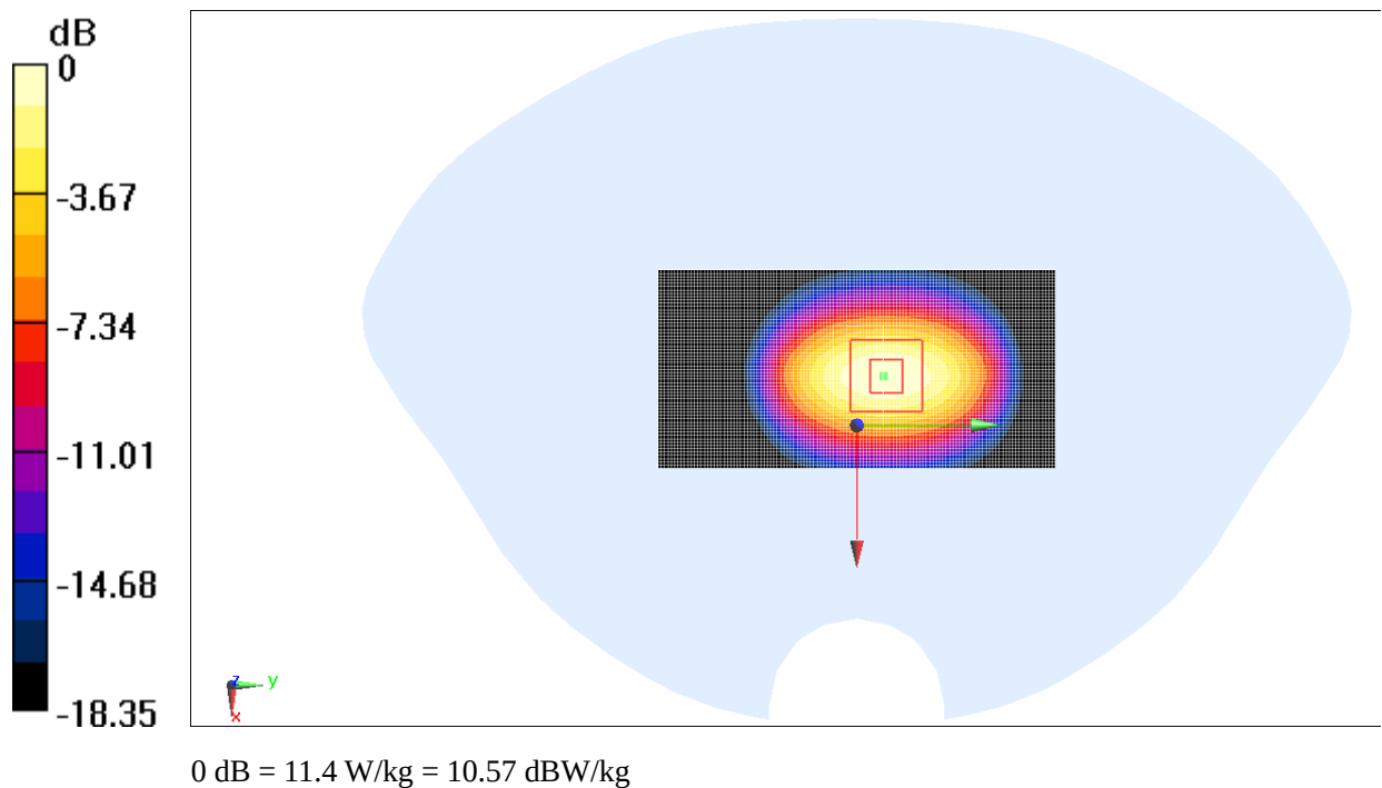
Fig.B.3 validation 1900MHz 250mW
