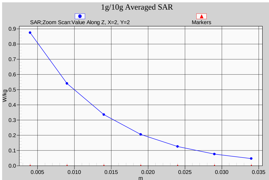
Fig. 4-1 Z-Scan at power reference point (1900 MHz CH661)
