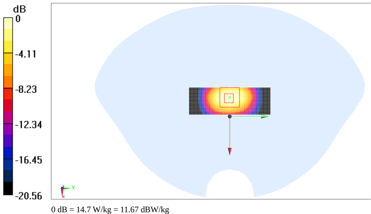
Fig.B.6 validation 2450MHz 250mW
