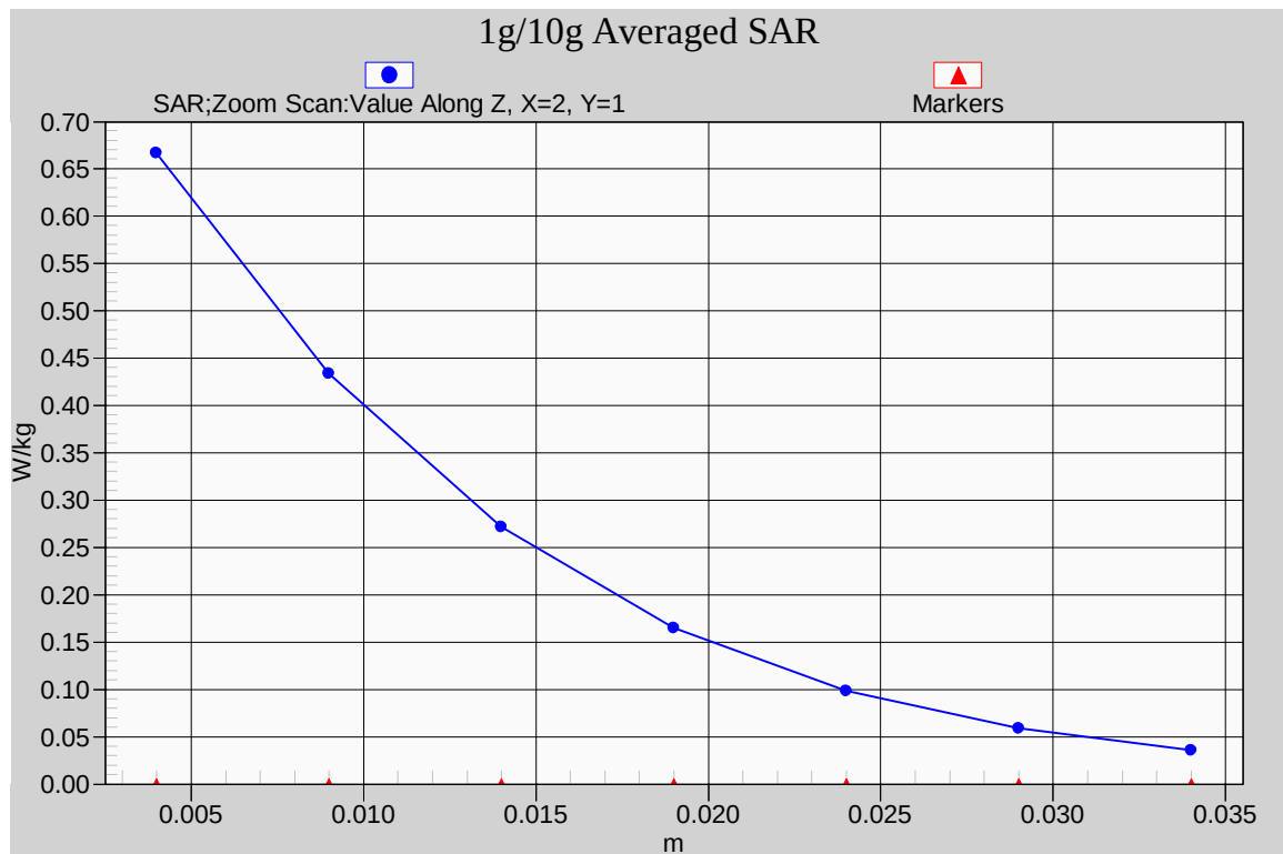
Fig. 3-1 Z-Scan at power reference point (1900MHz CH512)
