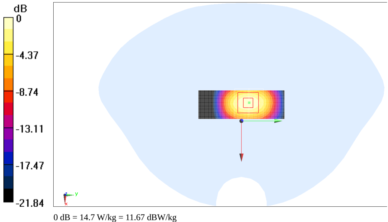
Fig.B.5 validation 2450MHz 250mW
