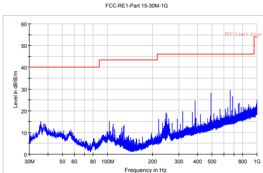
Fig. 54 Radiated Spurious Emission (GFSK, Ch78, 30 MHz ~1 GHz)
