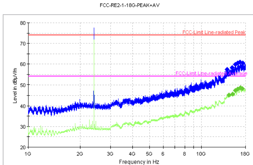
Fig. 67 Radiated Spurious Emission (8DPSK, Ch0, 1 GHz ~18 GHz)
