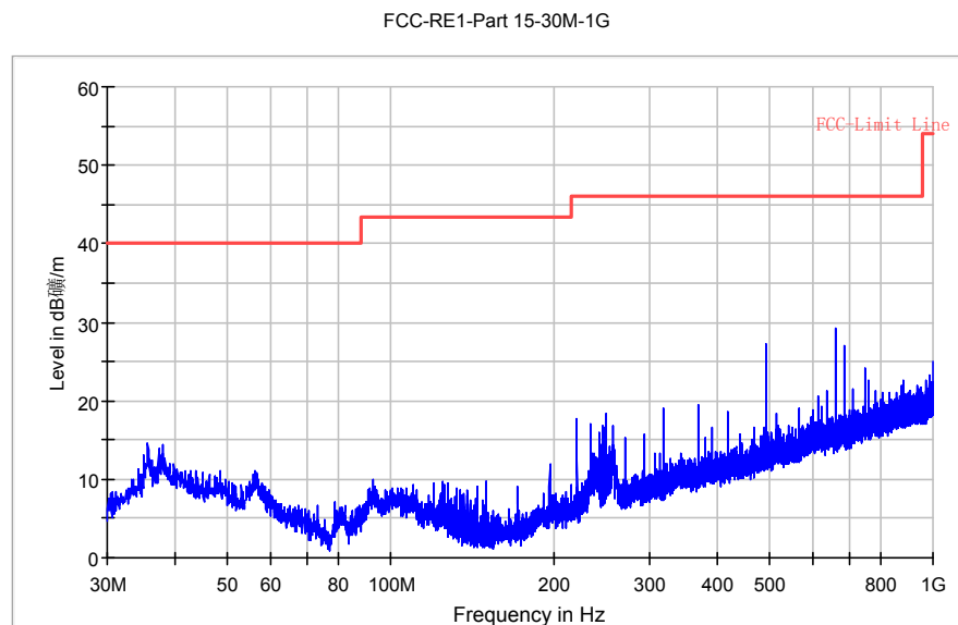
Fig. 60 Radiated Spurious Emission ( \pi/4 DQPSK, Ch39, 30 MHz ~1 GHz)
