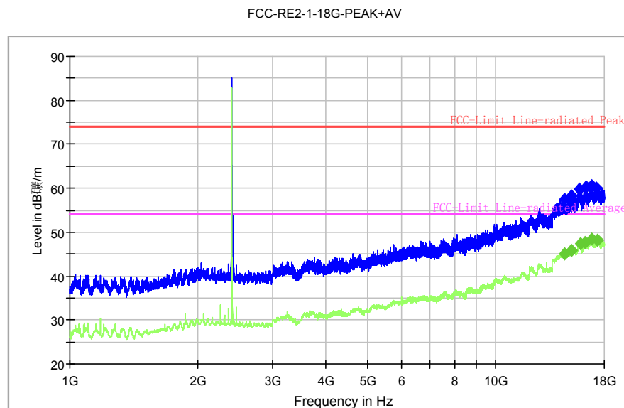
Fig. 51 Radiated Spurious Emission (GFSK, Ch0, 1 GHz ~18 GHz)
