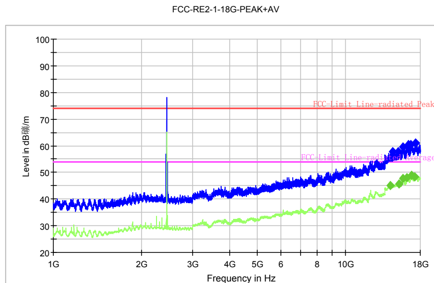
Fig. 61 Radiated Spurious Emission ( \pi/4 DQPSK, Ch39, 1 GHz ~18 GHz)
