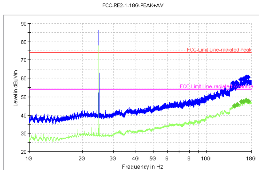
Fig. 71 Radiated Spurious Emission (8DPSK, Ch78, 1 GHz ~18 GHz)
