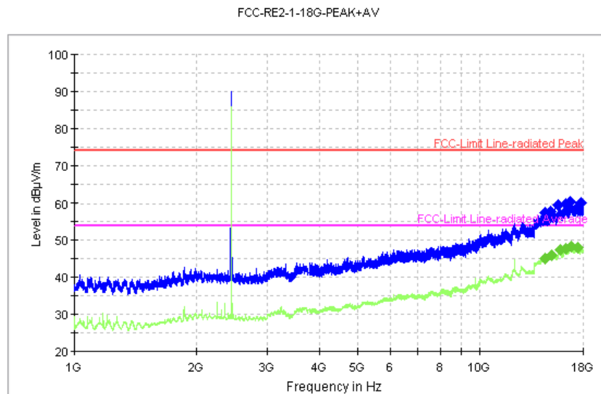
Fig. 69 Radiated Spurious Emission (8DPSK, Ch39, 1 GHz ~18 GHz)
