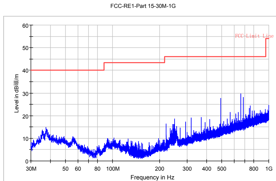
Fig. 52 Radiated Spurious Emission (GFSK, Ch39, 30 MHz ~1 GHz)
