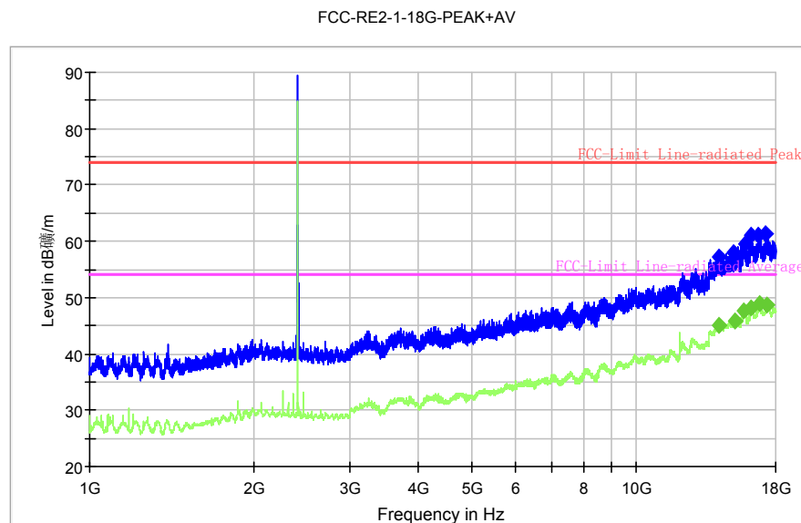
Fig. 59 Radiated Spurious Emission ( \pi/4 DQPSK, Ch0, 1 GHz ~18 GHz)
