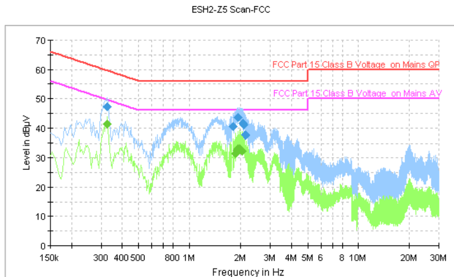
Fig. 99 AC Power line Conducted Emission (Traffic, AE1)
