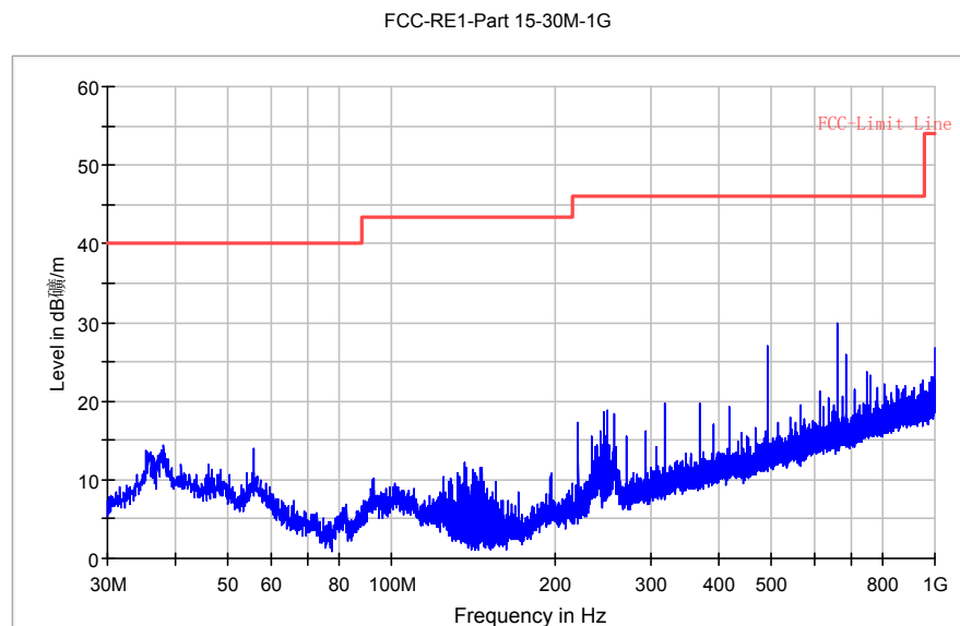
Fig. 121 Radiated Spurious Emission (802.11g, Ch1,30MHz-1 GHz)
