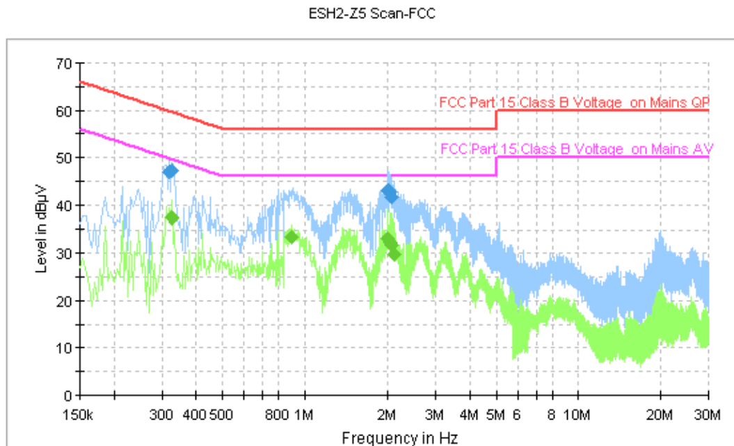
Fig. 139 AC Powerline Conducted Emission (Idle, AE2)
