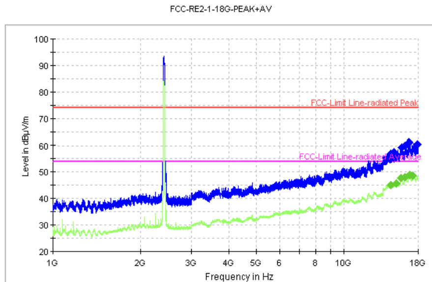
Fig. 122 Radiated Spurious Emission (802.11g, Ch1, 1 GHz-18 GHz)
