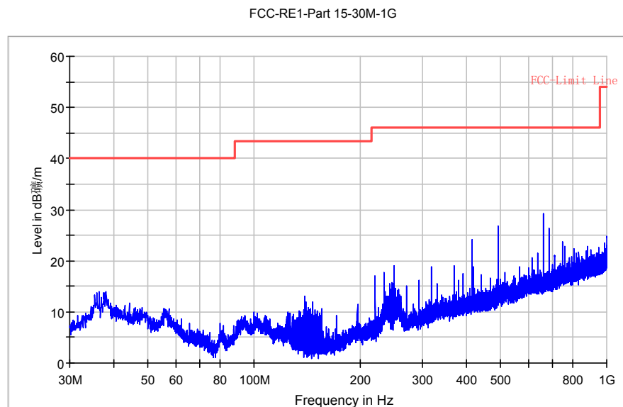
Fig. 125 Radiated Spurious Emission (802.11g, Ch11, 30MHz-1 GHz)
