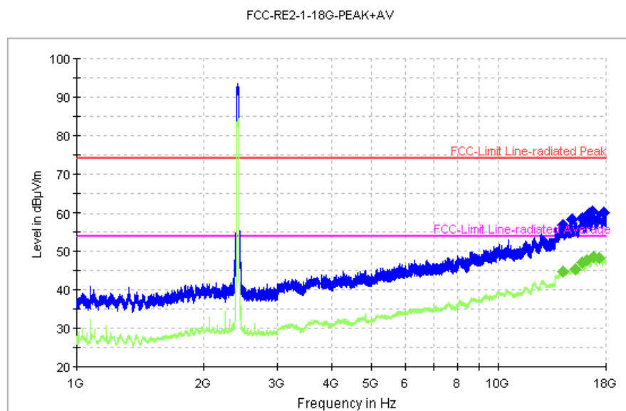
Fig. 130 Radiated Spurious Emission (802.11n-20M, Ch1, 1 GHz-18 GHz)
