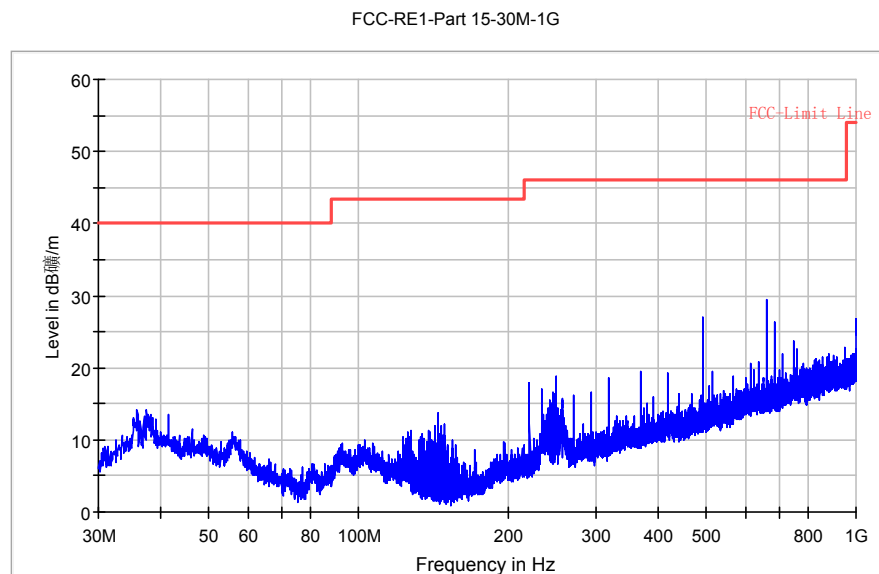
Fig. 115 Radiated Spurious Emission (802.11b, Ch6, 30MHz-1 GHz)
