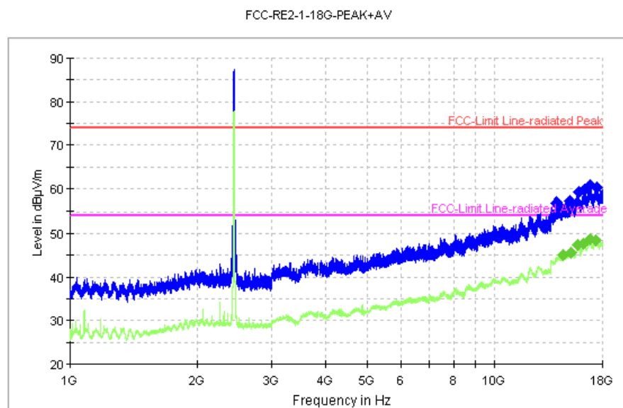
Fig. 132 Radiated Spurious Emission (802.11n-20M, Ch6, 1 GHz-18 GHz)
