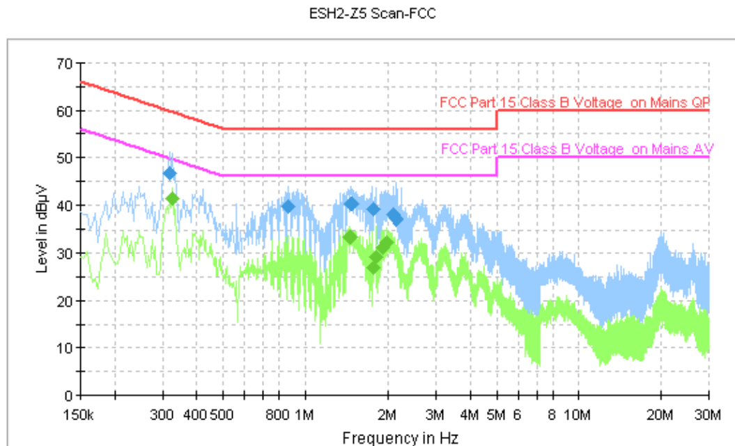
Fig. 138 AC Powerline Conducted Emission (Traffic, AE2)
