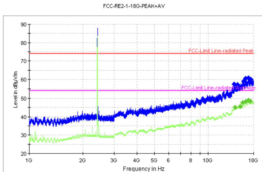
Fig. 114 Radiated Spurious Emission (802.11b, Ch1, 1 GHz-18 GHz)
