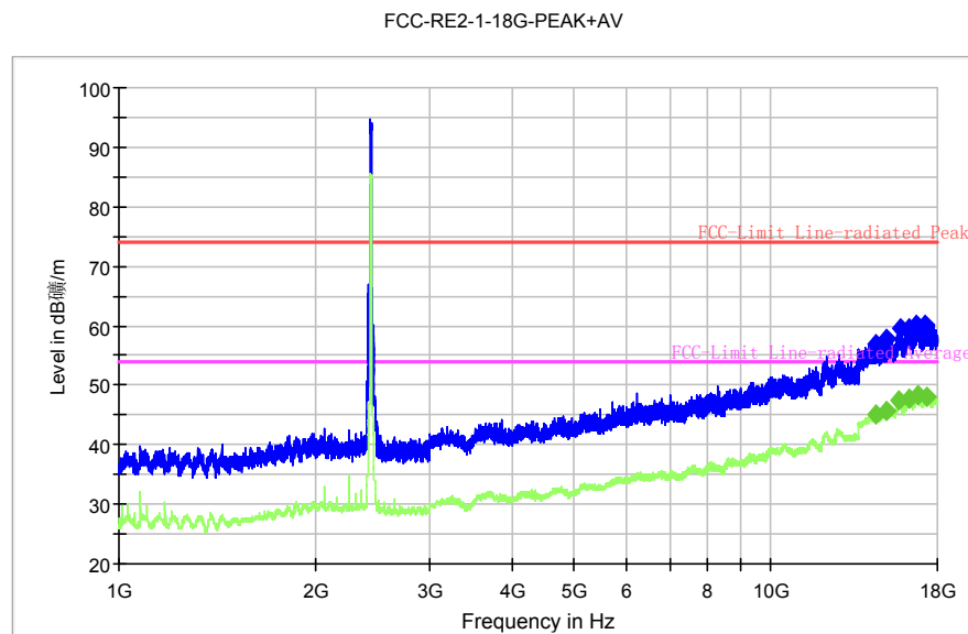
Fig. 124 Radiated Spurious Emission (802.11g, Ch6, 1 GHz-18 GHz)
