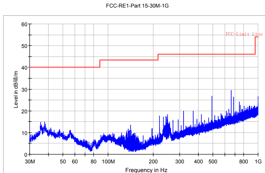
Fig. 129 Radiated Spurious Emission (802.11n-20M, Ch1, 30MHz-1 GHz)
