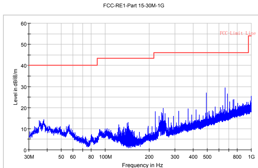
Fig. 123 Radiated Spurious Emission (802.11g, Ch6, 30MHz-1 GHz)
