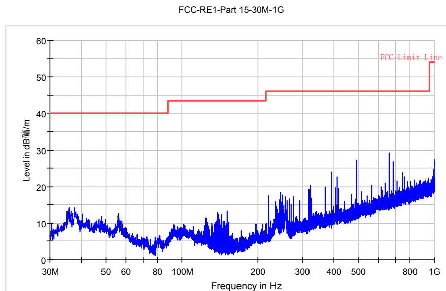
Fig. 131 Radiated Spurious Emission (802.11n-20M, Ch6, 30MHz-1 GHz)
