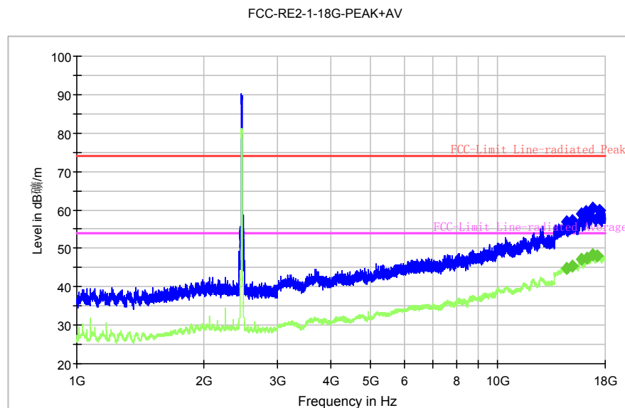
Fig. 134 Radiated Spurious Emission (802.11n-20M, Ch11, 1 GHz-18 GHz)
