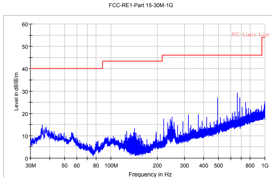
Fig. 133 Radiated Spurious Emission (802.11n-20M, Ch11, 30MHz-1 GHz)
