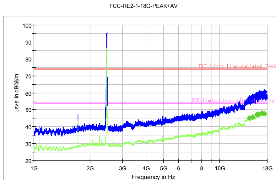
Fig. 126 Radiated Spurious Emission (802.11g, Ch11, 1 GHz-18 GHz)
