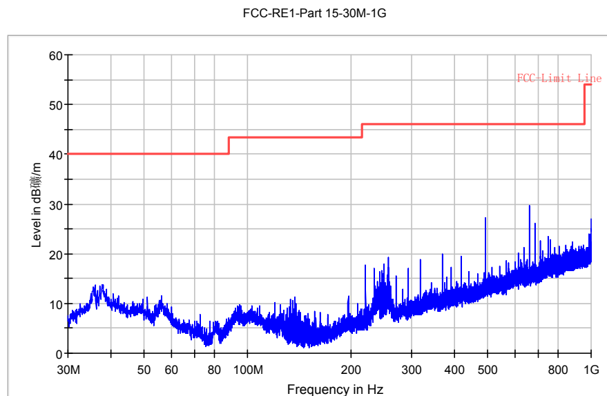
Fig. 113 Radiated Spurious Emission (802.11b, Ch1, 30MHz-1 GHz)
