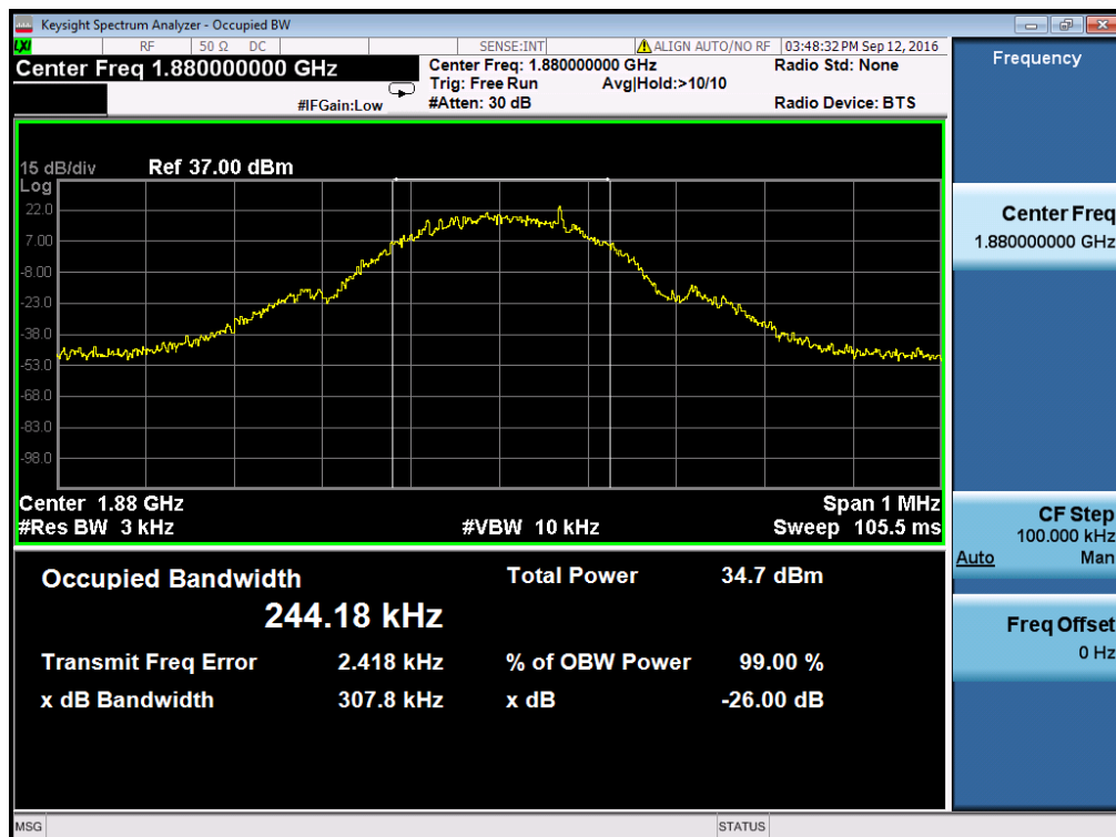
(Plot B2: GSM 1900MHz Channel = 661 bandwidth)
