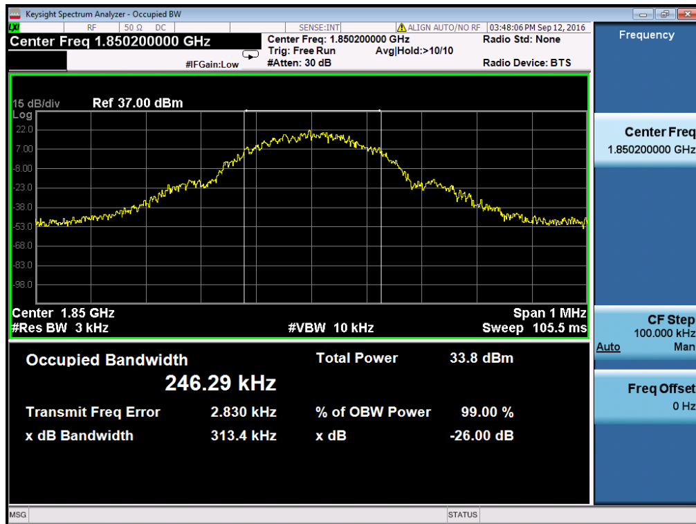
(Plot B1: GSM 1900MHz Channel = 512 bandwidth)
