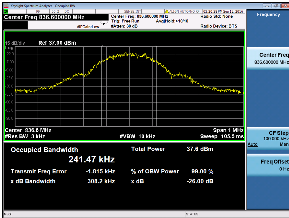
(Plot A2: GSM 850MHz Channel = 190 bandwidth)
