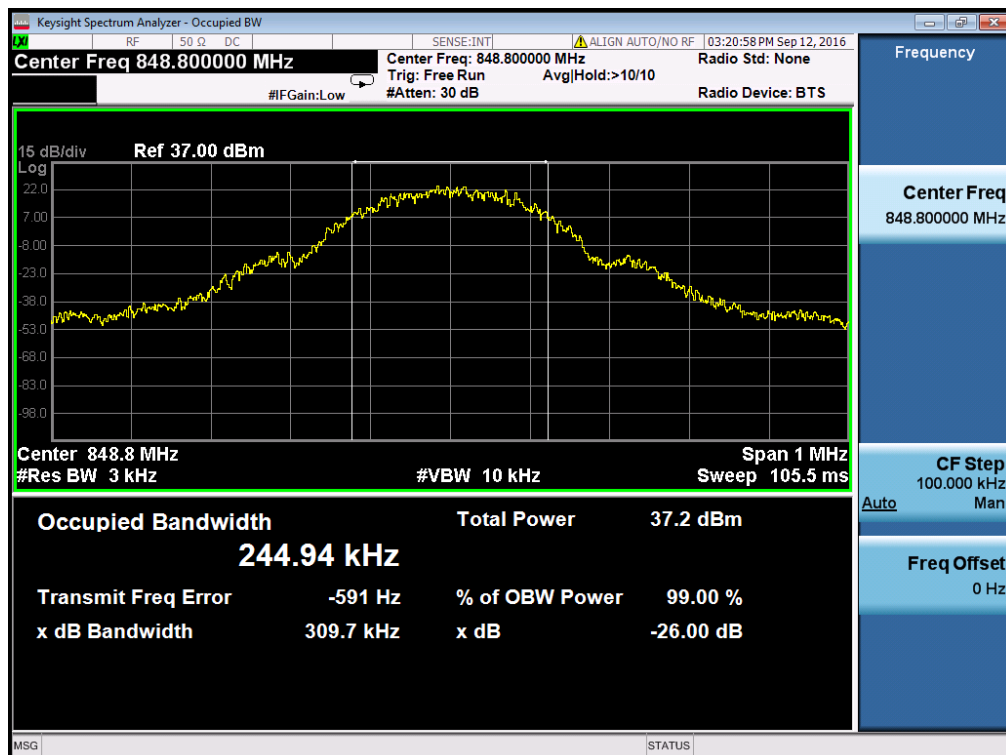
(Plot A3: GSM 850MHz Channel = 251 bandwidth)
