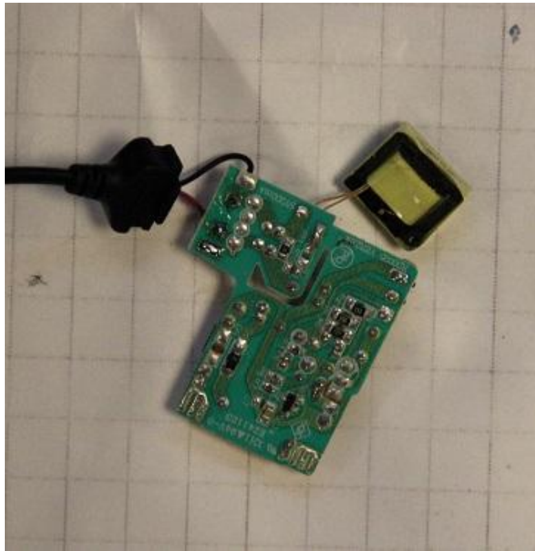
Charger board
