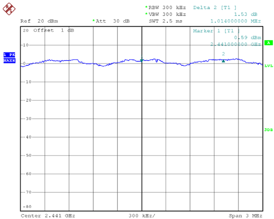
8-DPSK Mode
