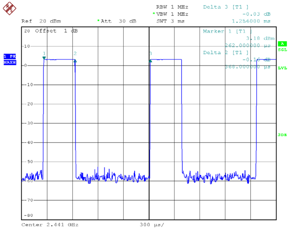
39 Channel @ DH1
