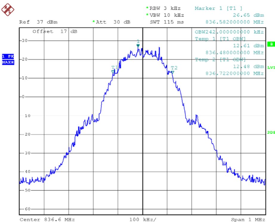
(Plot A4: GSM 850MHz Channel = 190 99% Occupied Bandwidth)
