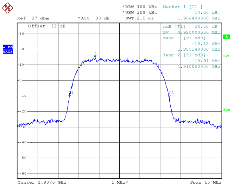
(Plot F5: WCDMA 1900MHz Channel = 9538 26dB bandwidth)
