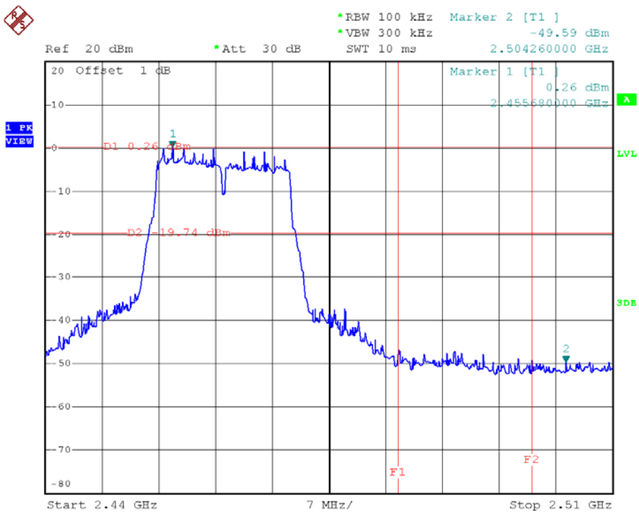
802.11g - High Band Edge Plot on Channel 11
