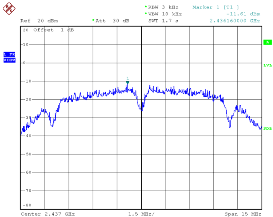
802.11b - Channel 6
