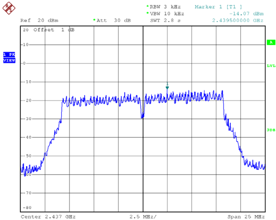
802.11g - Channel 6
