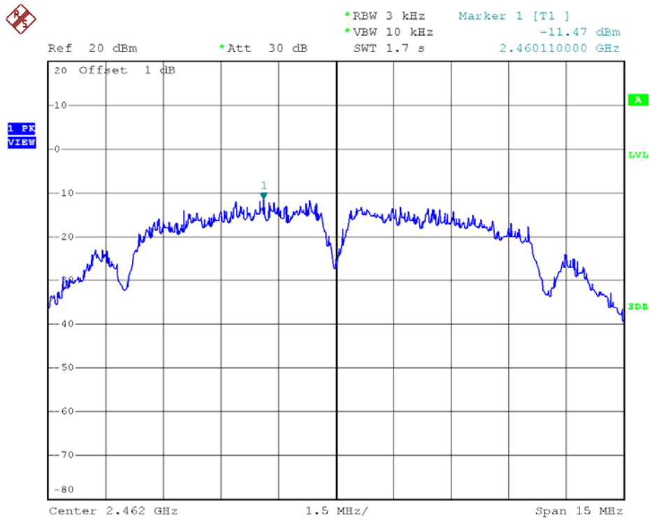
802.11b - Channel 11
