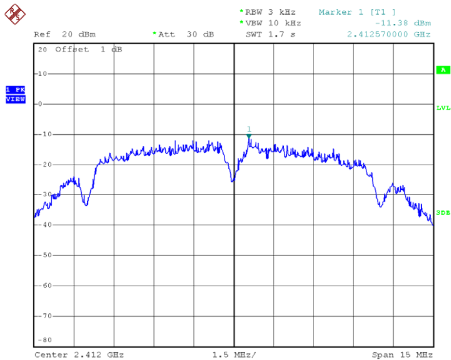
802.11b - Channel 1
