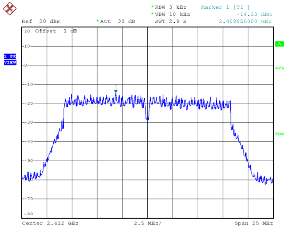
802.11g - Channel 1
