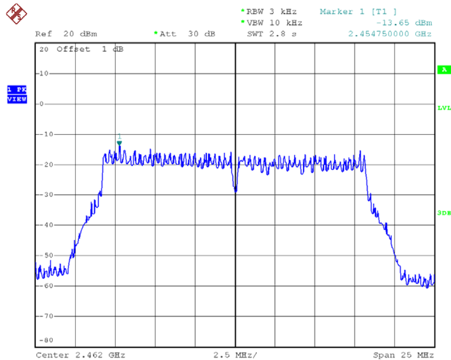
802.11g - Channel 11
