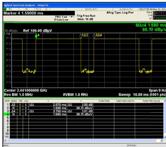
DH5 on time (One Pulse) Plot on Channel 39
