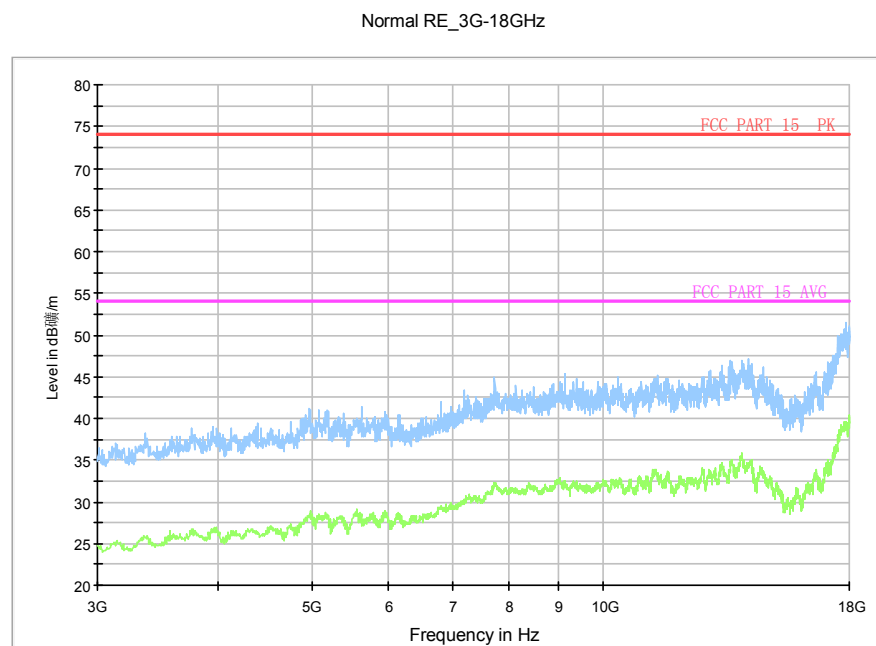
Fig.81. Radiated emission: 8DPSK, Channel 0, 3 GHz - 18 GHz
