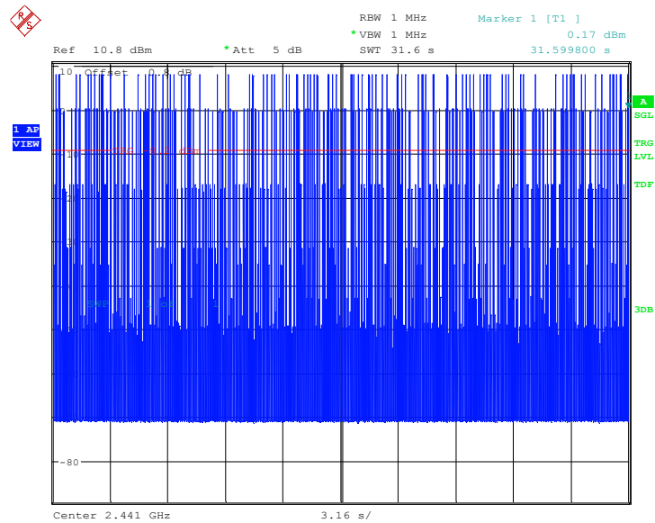
Fig.93. Time of occupancy (Dwell Time): Channel 39, Packet DH3
