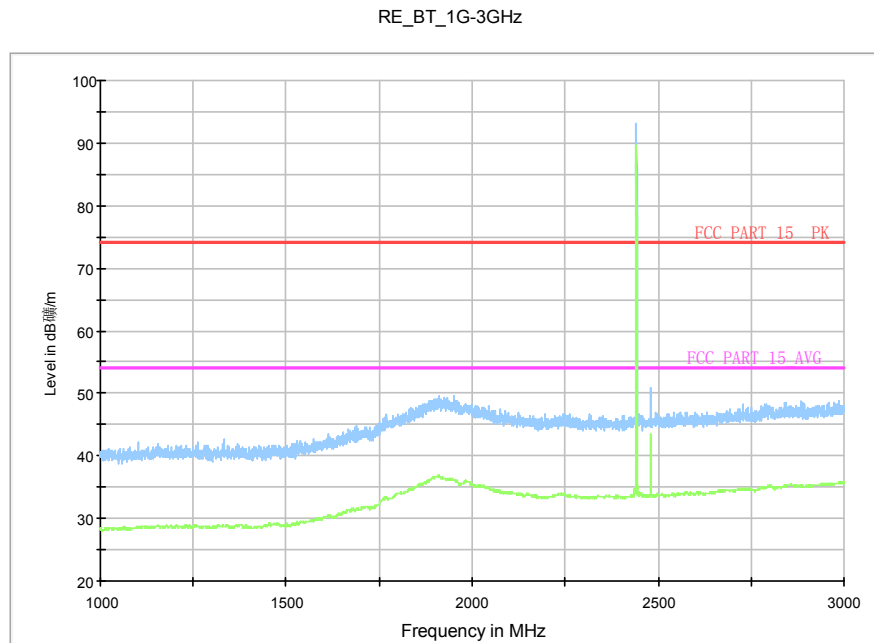
Fig.84. Radiated emission: 8DPSK, Channel 39, 1 GHz - 3 GHz
