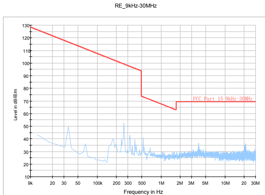
Fig.71. Radiated emission: \pi/4 DQPSK, Channel 39, 9 kHz ~ 30 MHz
