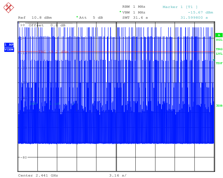
Fig.105. Time of occupancy (Dwell Time): Channel 39, Packet 3-DH3
