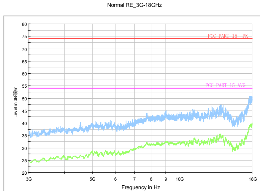
Fig.74. Radiated emission: \pi/4 DQPSK, Channel 39, 3 GHz - 18 GHz
