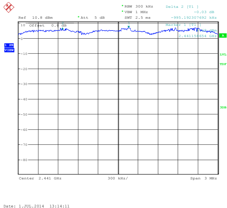
Fig.120. Carrier frequency separation measurement: 8DPSK, Channel 39
