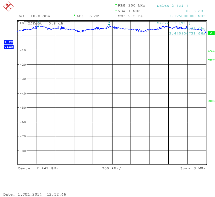
Fig.119. Carrier frequency separation measurement: \pi/4 DQPSK, Channel 39
