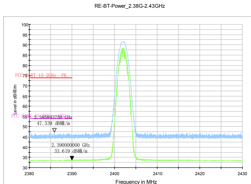
Fig.77. Radiated emission (Power): \pi/4 DQPSK, low channel
