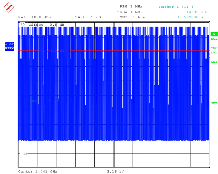
Fig.97. Time of occupancy (Dwell Time): Channel 39, Packet 2-DH1
