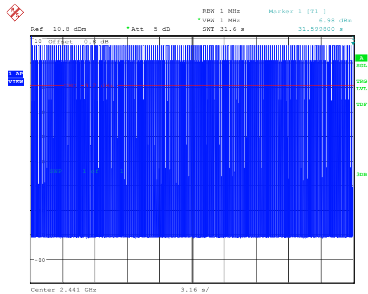
Fig.103. Time of occupancy (Dwell Time): Channel 39, Packet 3-DH1
