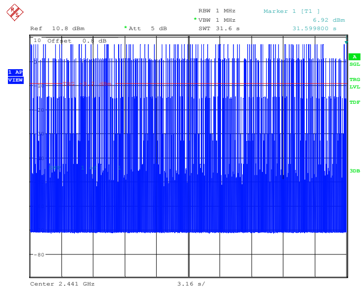
Fig.99. Time of occupancy (Dwell Time): Channel 39, Packet 2-DH3
