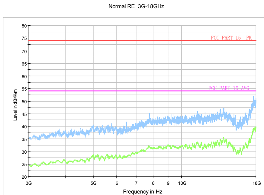
Fig.85. Radiated emission: 8DPSK, Channel 39, 3 GHz - 18 GHz
