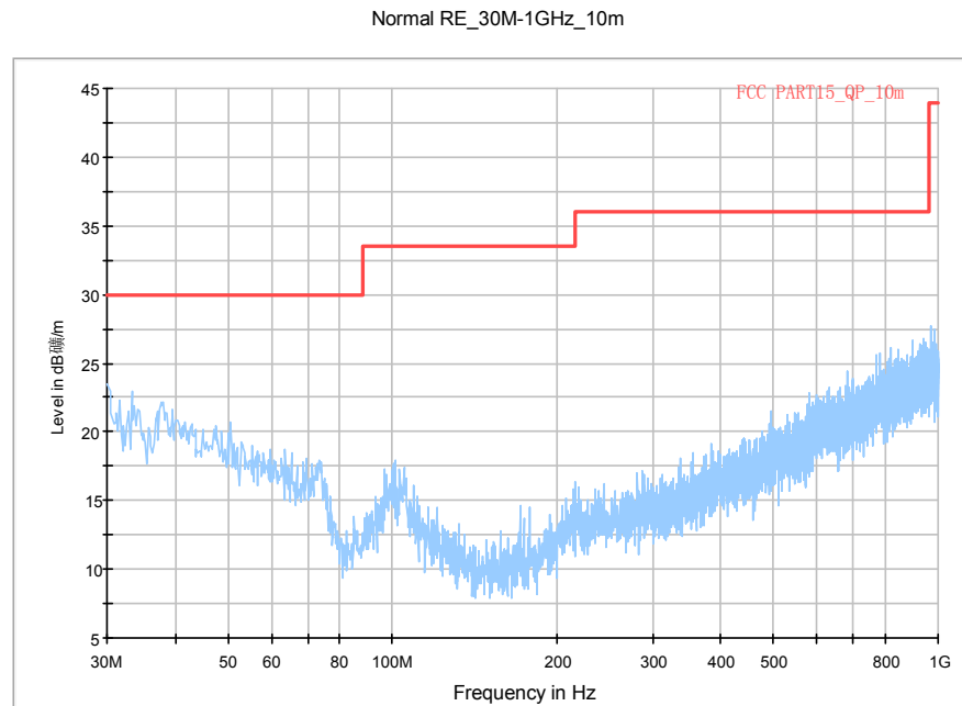
Fig.72. Radiated emission: \pi/4 DQPSK, Channel 39, 30 MHz - 1 GHz
