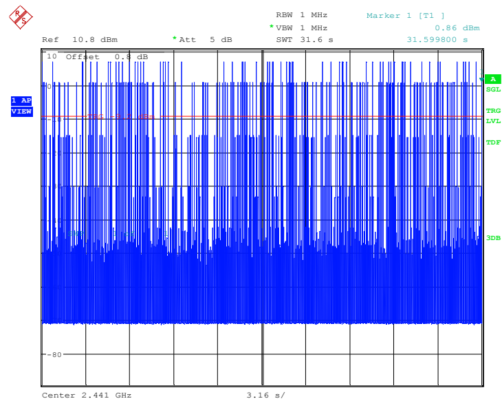
Fig.107. Time of occupancy (Dwell Time): Channel 39, Packet 3-DH5
