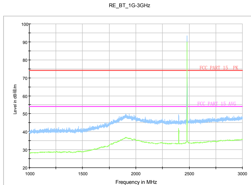
Fig.75. Radiated emission: \pi/4 DQPSK, Channel 78, 1 GHz - 3 GHz
