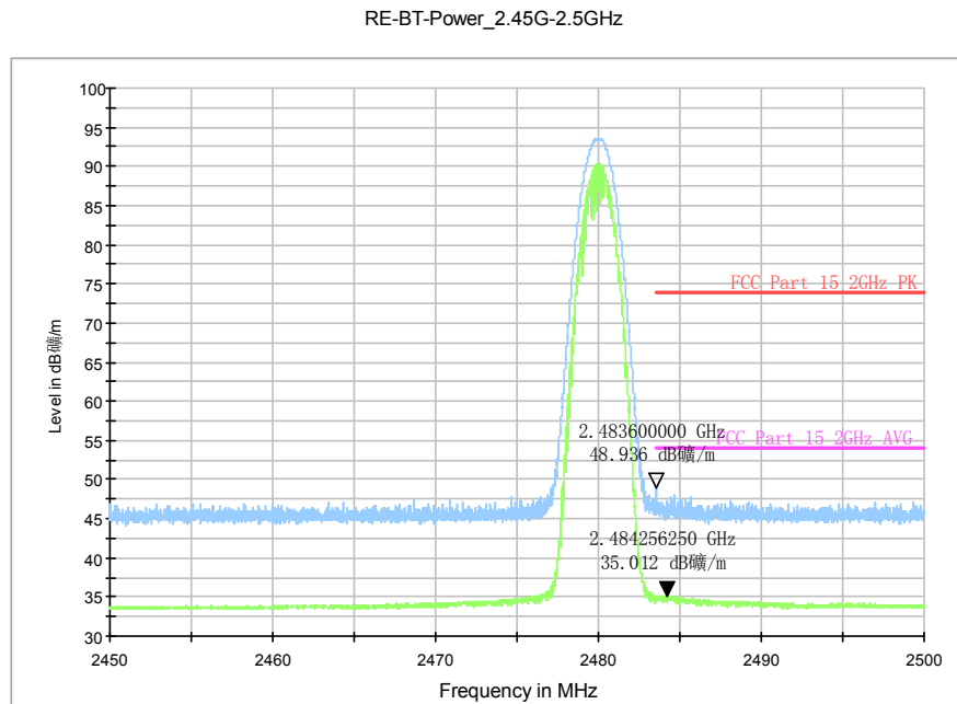
Fig.78. Radiated emission (Power): \pi/4 DQPSK, high channel
