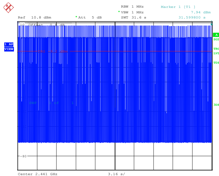
Fig.91. Time of occupancy (Dwell Time): Channel 39, Packet DH1
