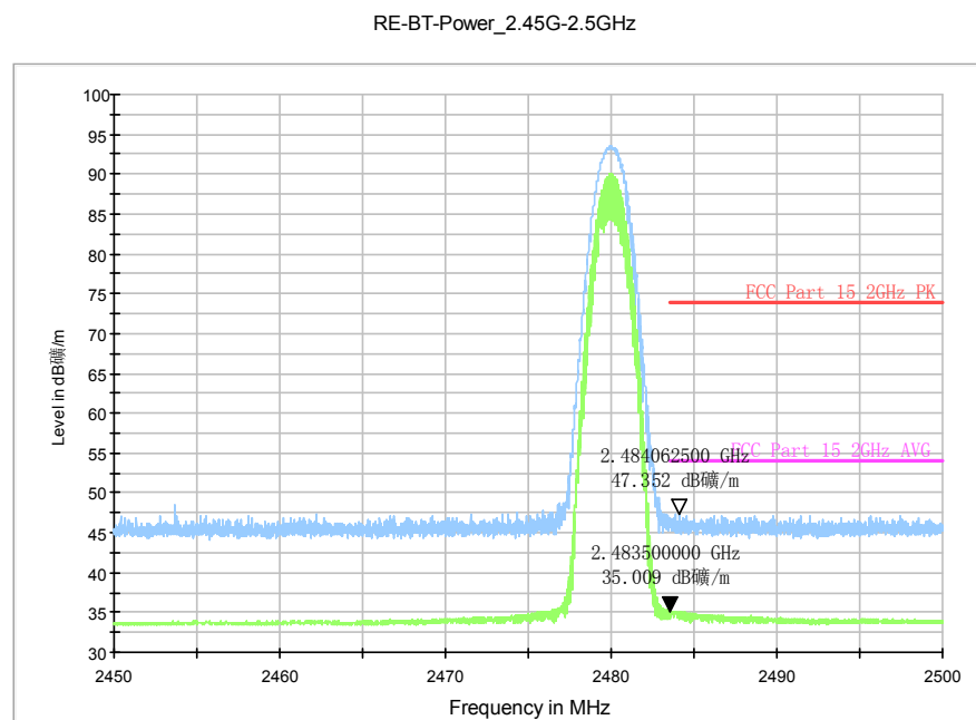
Fig.89. Radiated emission (Power): 8DPSK, high channel
