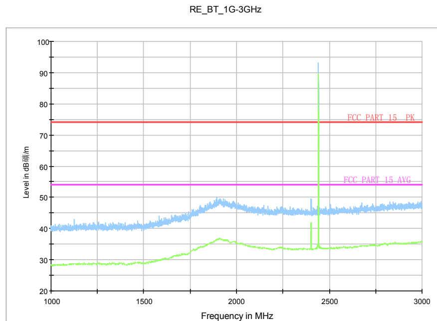
Fig.73. Radiated emission: \pi/4 DQPSK, Channel 39, 1 GHz - 3 GHz
