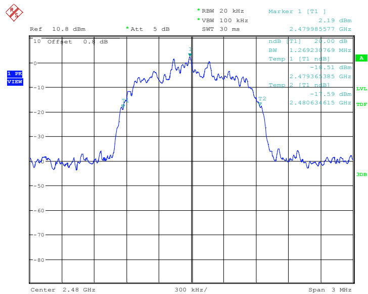
Fig.113. 20dB Bandwidth: \pi/4 DQPSK, Channel 39
