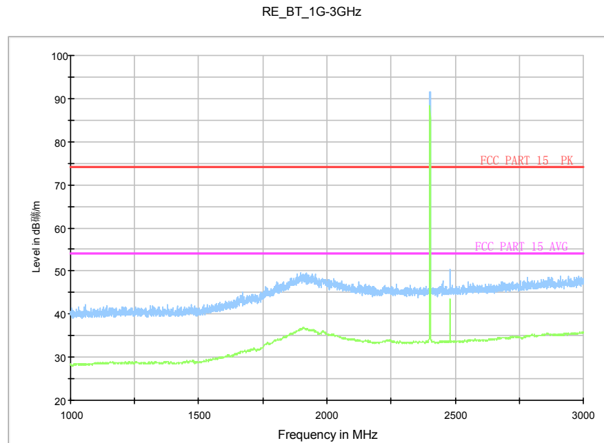
Fig.80. Radiated emission: 8DPSK, Channel 0, 1 GHz - 3 GHz
