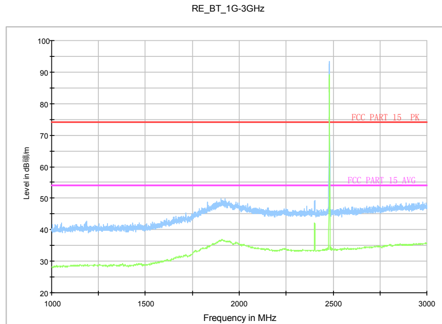
Fig.86. Radiated emission: 8DPSK, Channel 78, 1 GHz - 3 GHz
