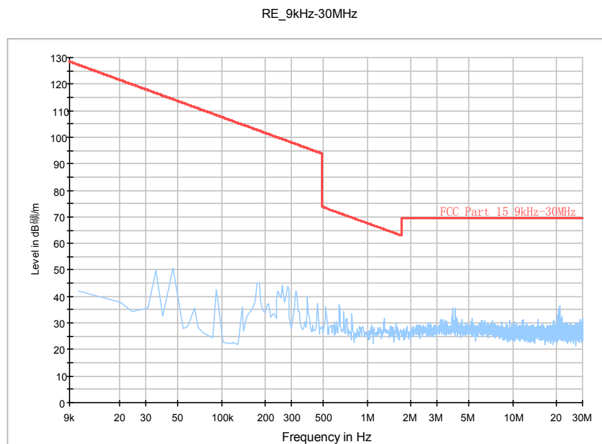
Fig.82. Radiated emission: 8DPSK, Channel 39, 9 kHz ~ 30 MHz
