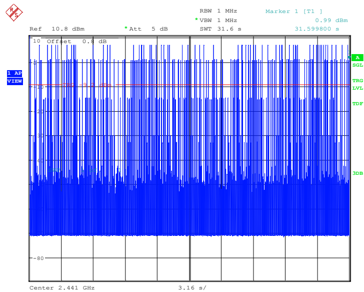
Fig.101. Time of occupancy (Dwell Time): Channel 39, Packet 2-DH5
