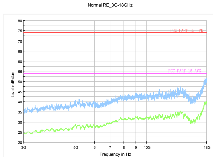
Fig.87. Radiated emission: 8DPSK, Channel 78, 3 GHz - 18 GHz
