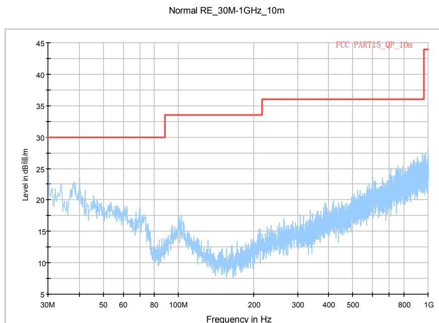
Fig.83. Radiated emission: 8DPSK, Channel 39, 30 MHz - 1 GHz
