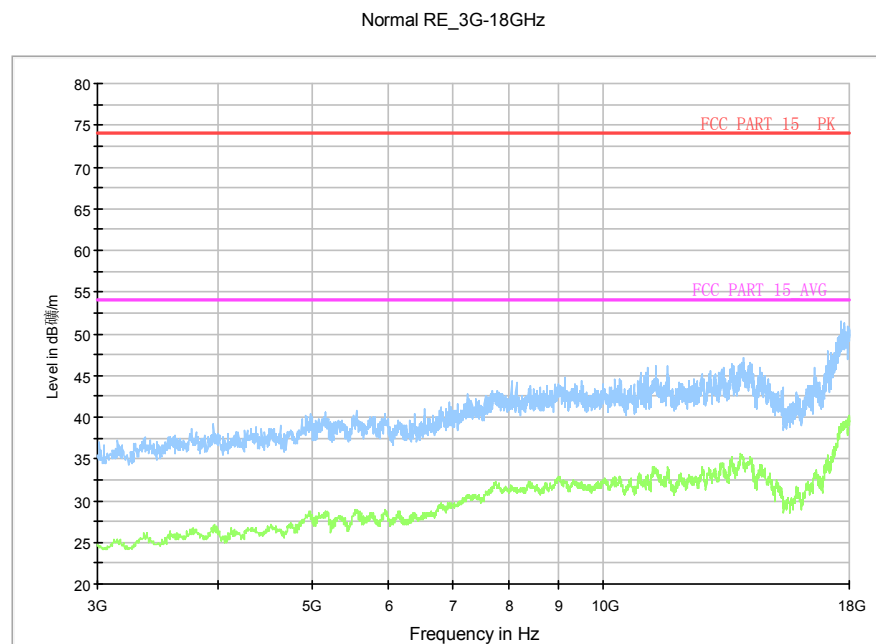
Fig.76. Radiated emission: \pi/4 DQPSK, Channel 78, 3 GHz - 18 GHz
