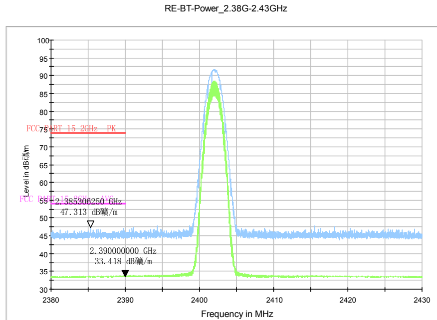
Fig.88. Radiated emission (Power): 8DPSK, low channel
