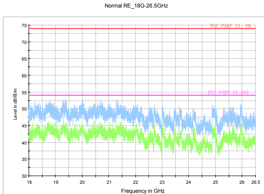
Fig.79. Radiated emission: \pi/4 DQPSK, 18 GHz - 26 GHz
