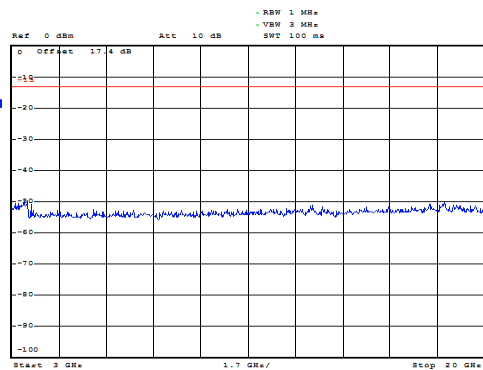
GSM 1900 CH-Low 3GHz~20GHz
