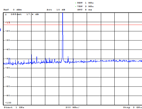
GSM 1900 CH-Low 1GHz~3GHz
