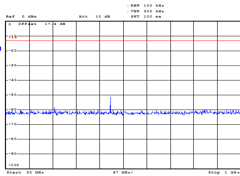
GSM 1900 CH-Low 30MHz~1GHz
