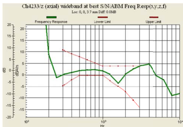
Fig. 7.9 WCDMA Band V Ch4233
