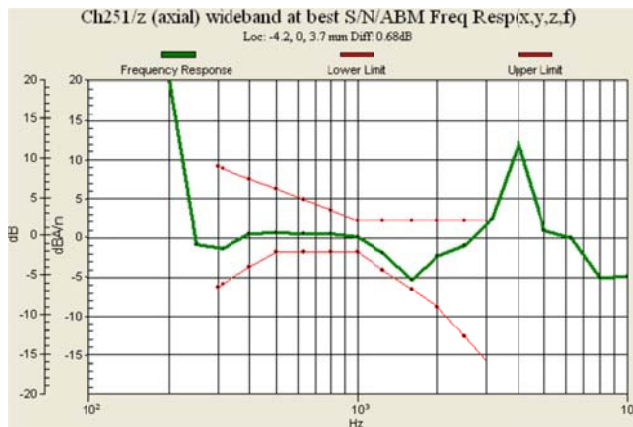
Fig 7.3 GSM850 Ch251
