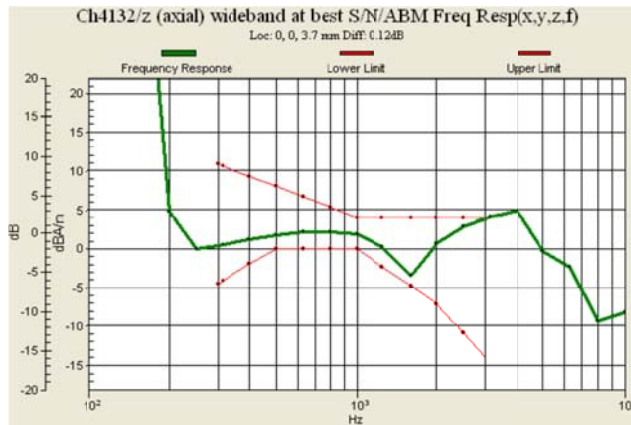
Fig 7.7 WCDMA Band V Ch4132
