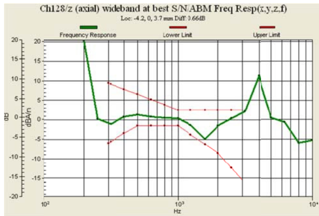
Fig 7.1 GSM850 Ch128
