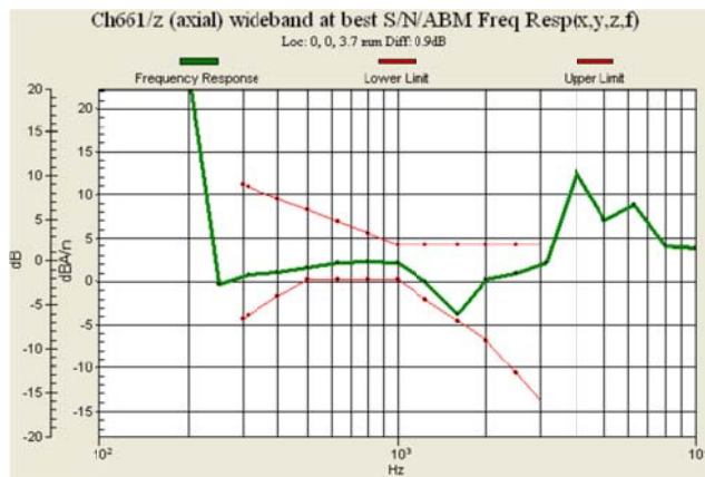
Fig 7.5 GSM1900 Ch661
