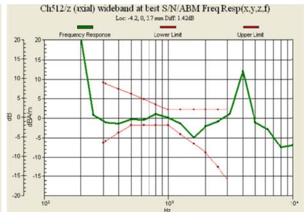
Fig 7.4 GSM1900 Ch512
