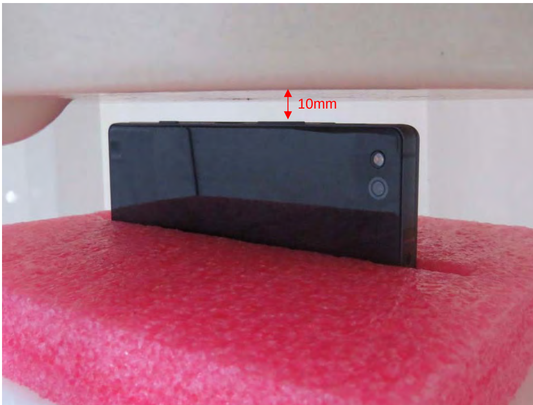
Picture 18: Left Side, the distance from handset to the bottom of the Phantom is 10mm For Single Screen Mode
