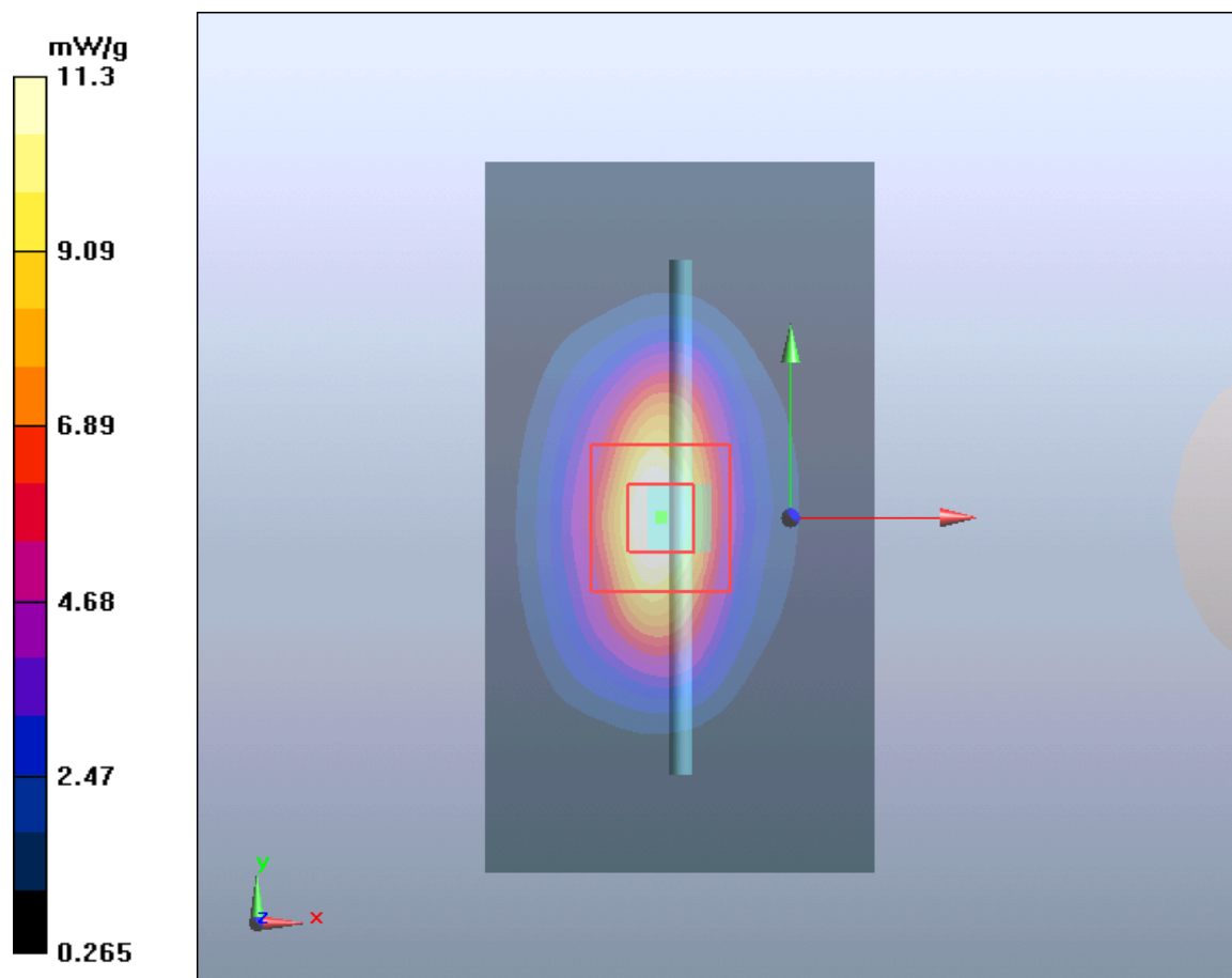
Plot 9 System Performance Check at 2450 MHz Head TSL
