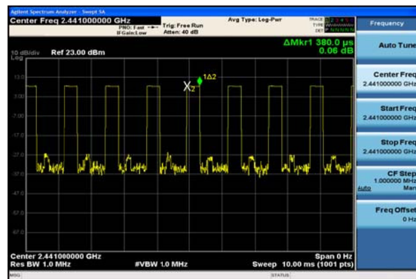
BT DH3 CH39, Carrier frequency (MHz): 2441
