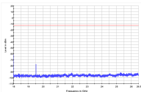
GFSK-CH39 18GHz to 26.5GHz
