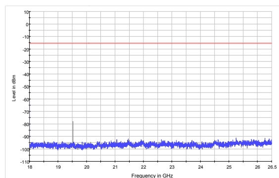
EDR-CH39 18GHz to 26.5GHz
