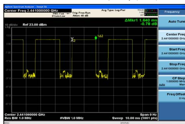
BT DH5 CH39, Carrier frequency (MHz): 2441
