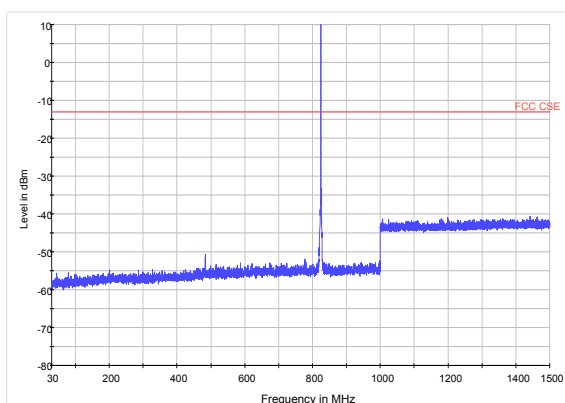
LTE Band 5 1.4MHz CH-Middle 30MHz~1.5GHz
