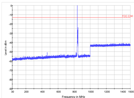
LTE Band 5 10MHz CH-High 30MHz~1.5GHz
