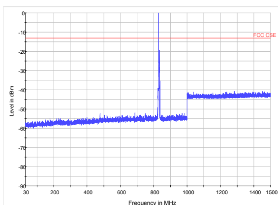
LTE Band 26 5MHz CH-High 30MHz~1.5GHz
