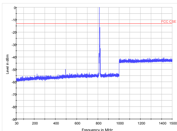
LTE Band 26 5MHz CH-Middle 30MHz~1.5GHz
