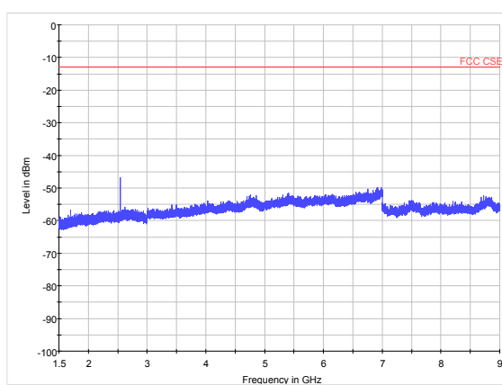
LTE Band 26 1.4MHz CH-High 1.5GHz~9GHz
