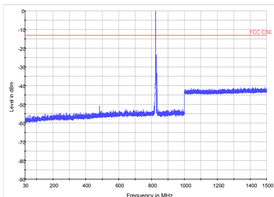
LTE Band 5 5MHz CH-Middle 30MHz~1.5GHz
