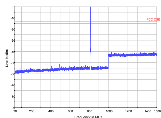
LTE Band 26 1.4MHz CH-Middle 30MHz~1.5GHz
