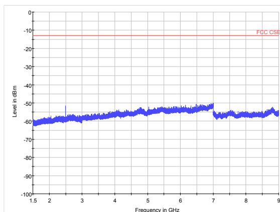
LTE Band 26 10MHz CH-High 1.5GHz~9GHz
