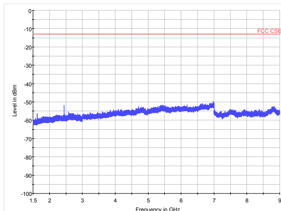
LTE Band 26 1.4MHz CH-Middle 1.5GHz~9GHz
