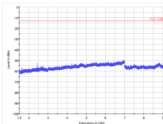
LTE Band 26 5MHz CH-Middle 1.5GHz~9GHz
