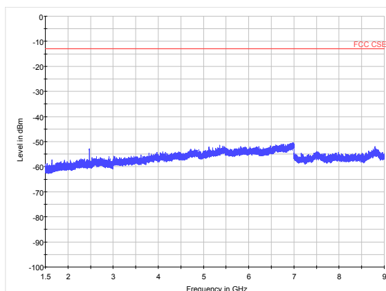
LTE Band 26 15MHz CH-Middle 1.5GHz~9GHz
