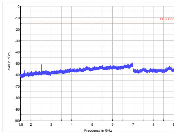
LTE Band 26 5MHz CH-High 1.5GHz~9GHz
