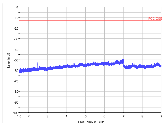
LTE Band 26 15MHz CH-High 1.5GHz~9GHz
