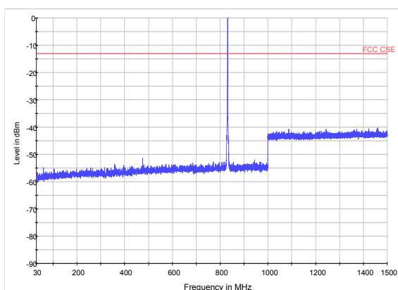
LTE Band 26 1.4MHz CH-High 30MHz~1.5GHz
