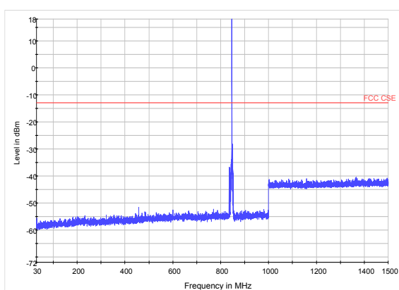
LTE Band 5 3MHz CH-High 30MHz~1.5GHz
