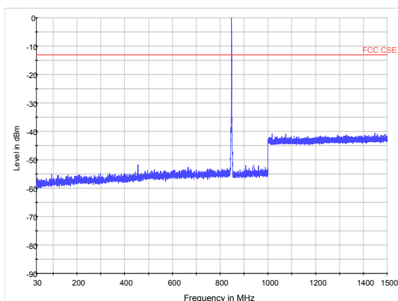
LTE Band 26 1.4MHz CH-High 30MHz~1.5GHz
