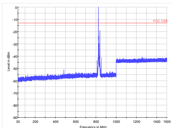
LTE Band 26 15MHz CH-Middle 30MHz~1.5GHz
