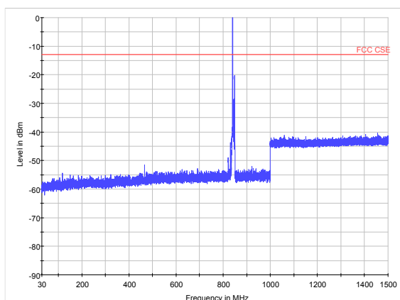
LTE Band 26 10MHz CH-High 30MHz~1.5GHz
