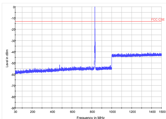
LTE Band 26 3MHz CH-High 30MHz~1.5GHz
