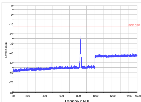
LTE Band 5 10MHz CH-Middle 30MHz~1.5GHz
