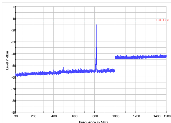
LTE Band 26 3MHz CH-Middle 30MHz~1.5GHz
