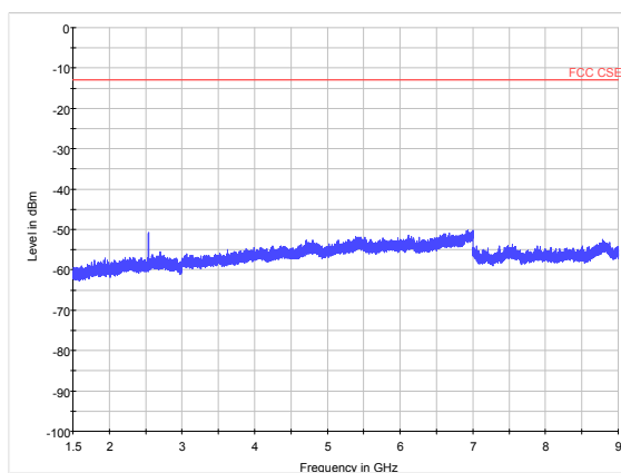
LTE Band 26 3MHz CH-High 1.5GHz~9GHz
