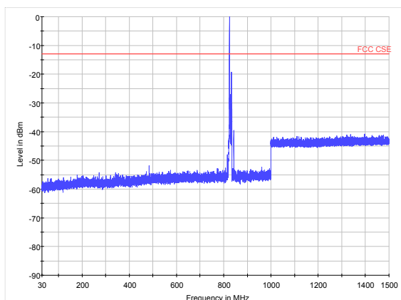
LTE Band 26 10MHz CH-Middle 30MHz~1.5GHz
