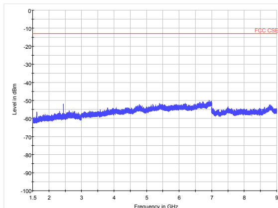
LTE Band 26 3MHz CH-Middle 1.5GHz~9GHz
