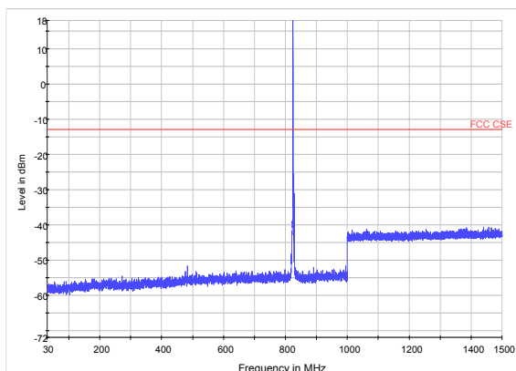
LTE Band 5 3MHz CH-Middle 30MHz~1.5GHz
