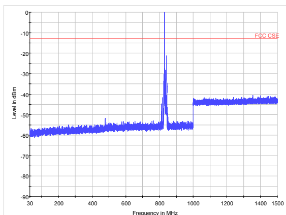
LTE Band 26 15MHz CH-High 30MHz~1.5GHz
