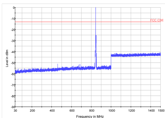
LTE Band 5 5MHz CH-High 30MHz~1.5GHz
